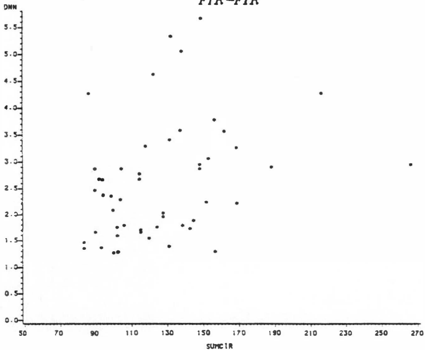
Fig. 22. Graphs of distance to nearest neighbor (m) vs. sum of trunk circumferences (cm) (spruce-birch, fir-fir). Correlations of spruce-birch values, and fir-fir values were both significant.
