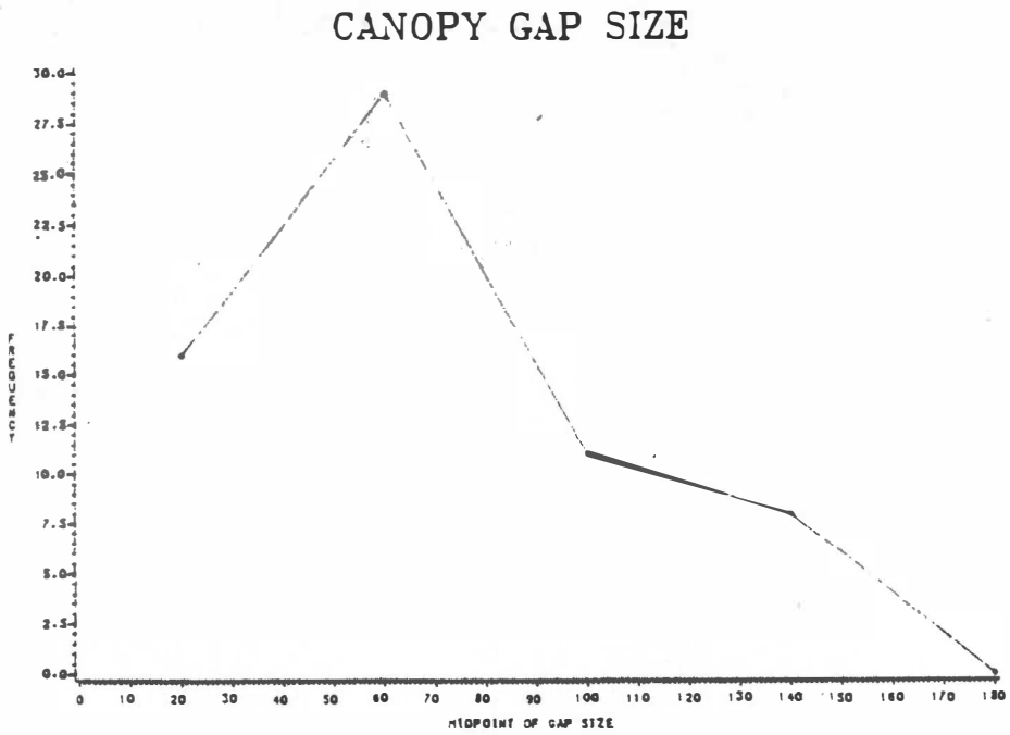
Fig. 6. Graph of canopy gap size distribution. Size is in m 2 .
