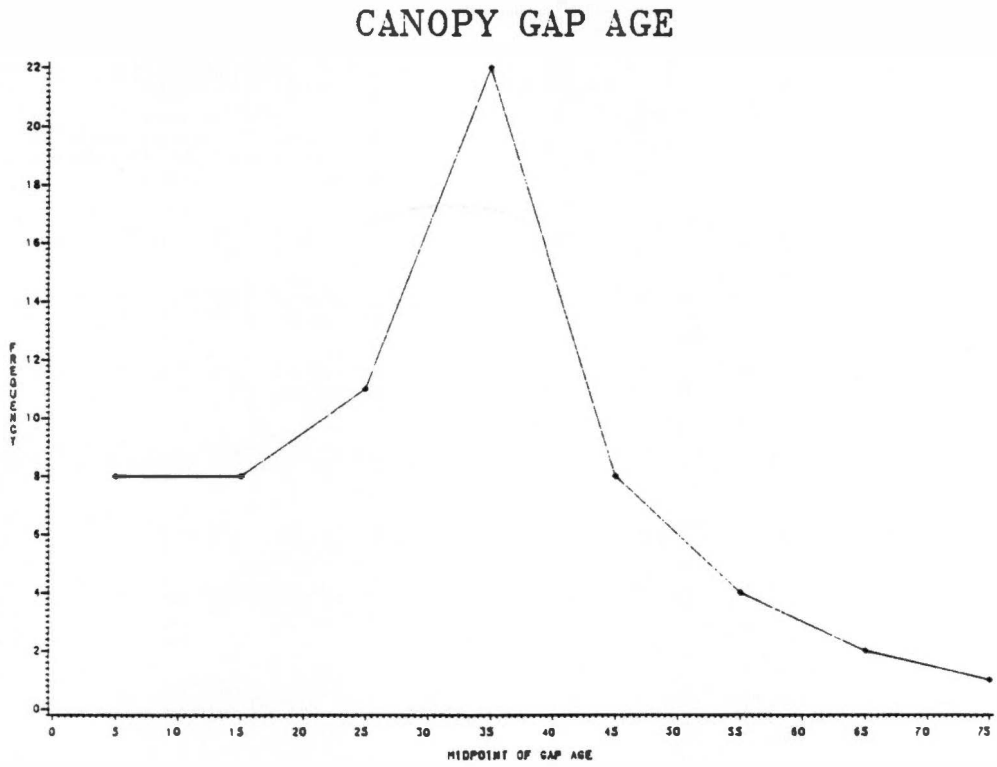
Fig. 5. Graph of canopy gap age distribution.
