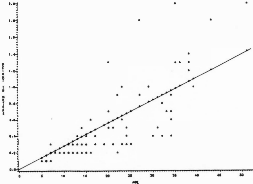
Fig. 61. Graph of Fraser fir height vs. age. Based on transect sampled individuals less than 2.0 m tall. Linear regression r^2=0.83 .
