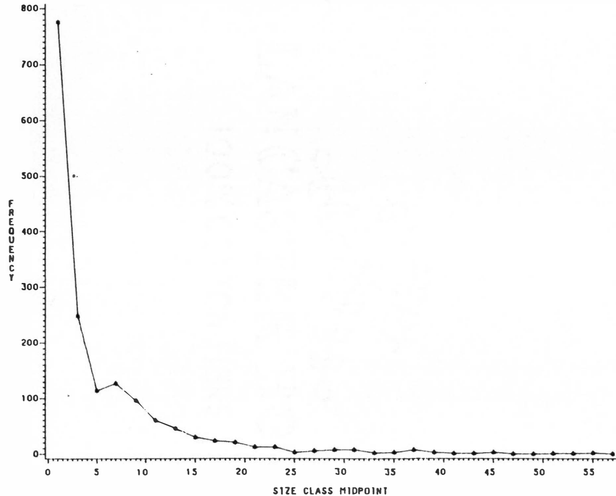
Fig. 24. Graph of Fraser fir size structure. Size is in cm DBH. Individuals less than 2.5 cm DBH are not included.
