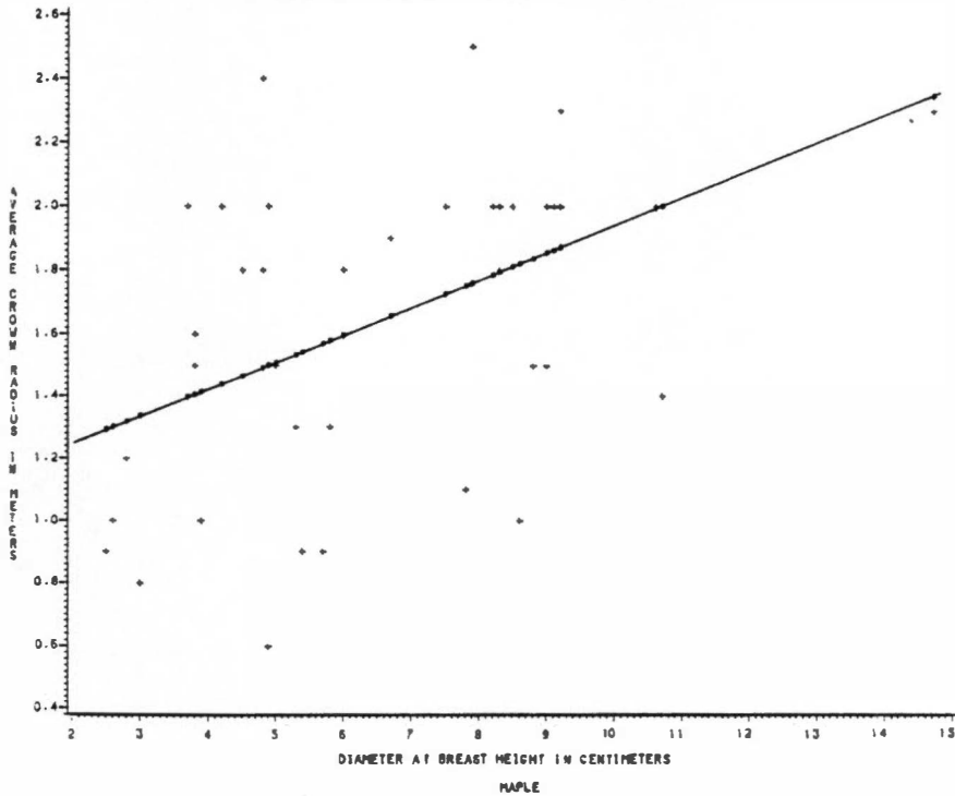
Fig. 65. Graph of mountain maple crown radius vs. DBH. Linear regression r^2=0.21 .
