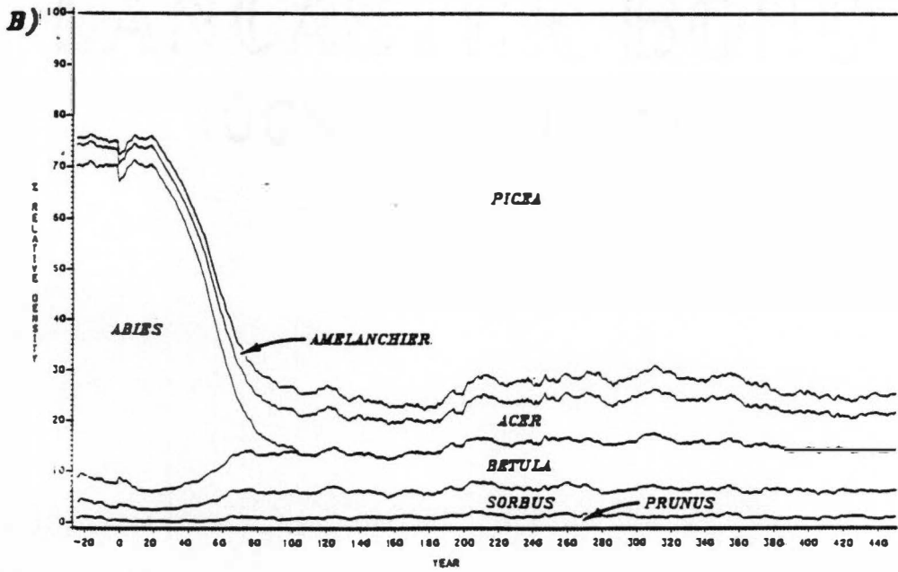
Fig. 45. Graphs of simulated density responses to the elimination of fir. These are: A) total stand density (stems > 1.27 cm DBH/ha), and B) relative density.
