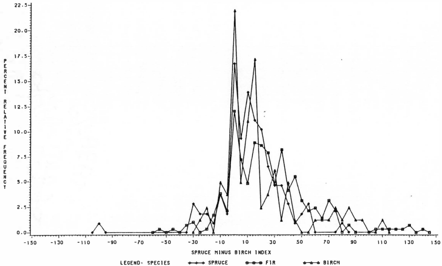
Fig. 13. Distribution of spruce, fir and birch saplings in relation to spruce and birch canopy trees as quantified by the spruce minus birch index.
