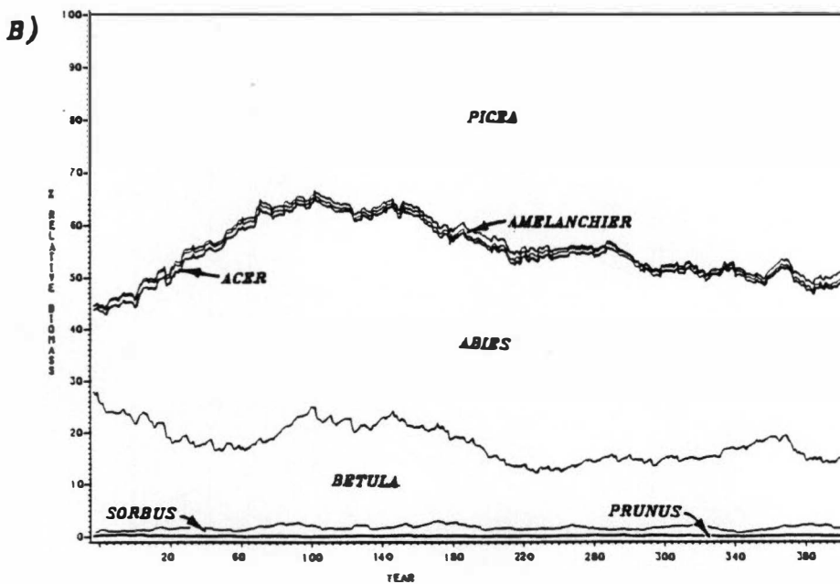
Fig. 52. Graphs of simulated biomass responses to a short-term, 30% spruce growth decline. These are: A) total stand biomass (t/ha), and B) relative biomass. The 30 yr growth decline begins at year 0.
