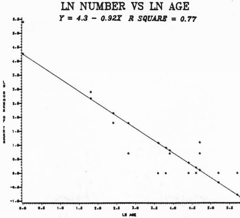
Fig. 30. Graph of red spruce survivorship with linear regression.
