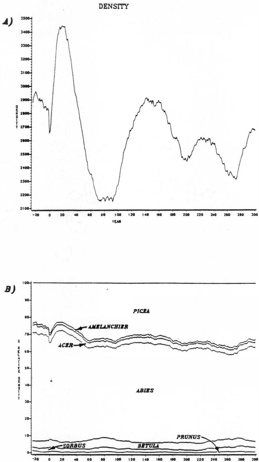
Fig. 47. Graphs of simulated density responses to a short-term fir infestation. These are: A) total stand density (stems > 1.27 cm DBH/ha), and B) relative density. The 10 yr infestation begins at year 0.
