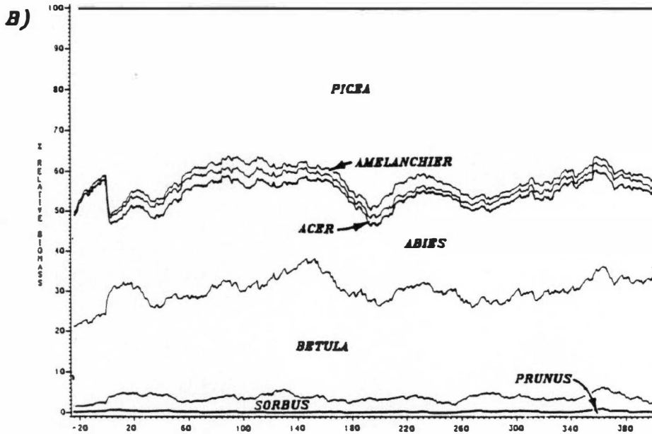
Fig. 54. Graphs of simulated biomass responses to continuous aphid infestation in combination with a 30% spruce growth decline. These are: A) total stand biomass (t/ha), and B) relative biomass. Disturbance begins at year 0.
