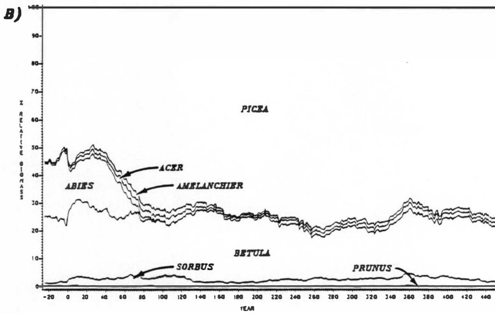
Fig. 46. Graphs of simulated biomass responses to the elimination of fir. These are: A) total stand biomass (t/ha), and B) relative biomass.
