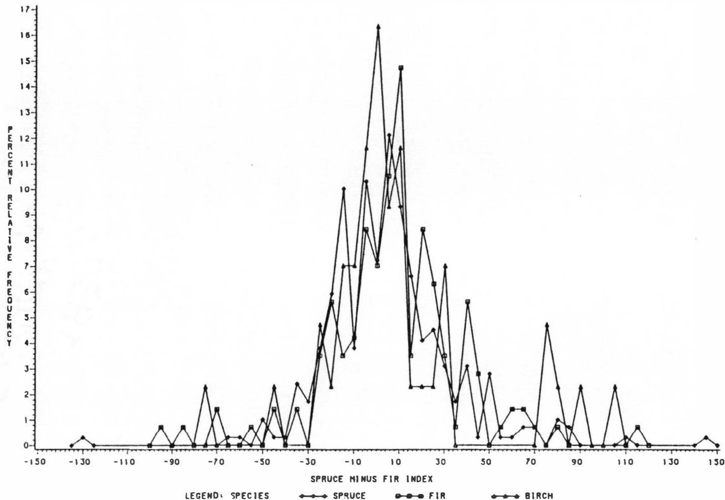
Fig. 8. Distribution of spruce, fir and birch seedlings in relation to spruce and fir canopy trees as quantified by the spruce minus fir index. No significant differences among distributions were revealed by rank-sum tests.
