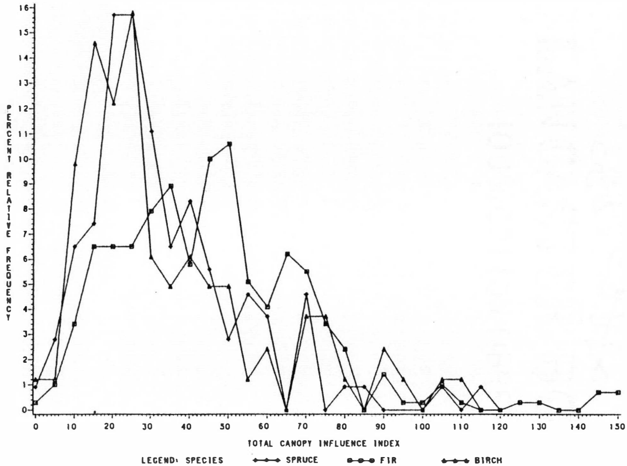
Fig. 18. Distribution of spruce, fir and birch saplings in relation to canopy trees as quantified by the total canopy influence index.
