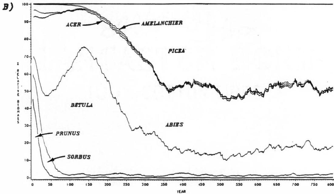
Fig. 38. Graphs of simulated biomass dynamics. These are: A) total biomass (t/ha), and B) relative biomass of individual species.
