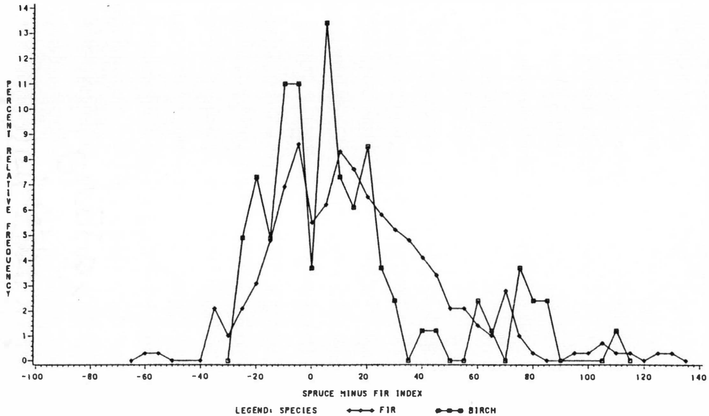
Fig. 11. Distribution of fir and birch saplings in relation to spruce and fir canopy trees as quantified by the spruce minus fir index. A significant difference between distributions was revealed by the rank-sum test ( p < 0.05 ).
