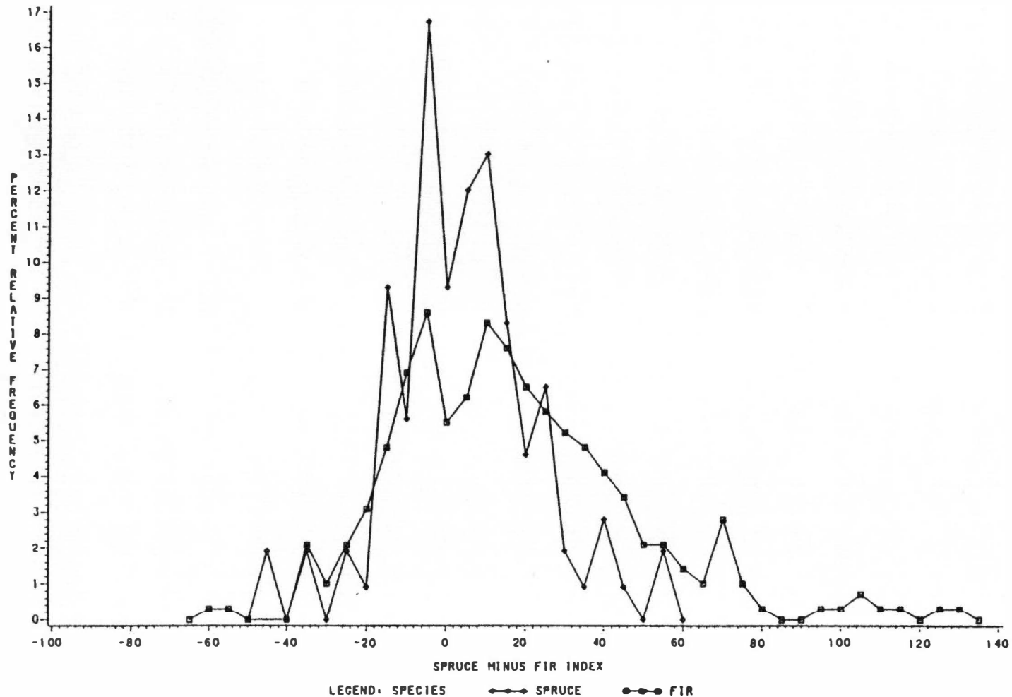
Fig. 10. Distribution of spruce and fir saplings in relation to spruce and fir canopy trees as quantified by the spruce minus fir index. A highly significant difference between distributions was revealed by the rank-sum test ( p < 0.01 ).
