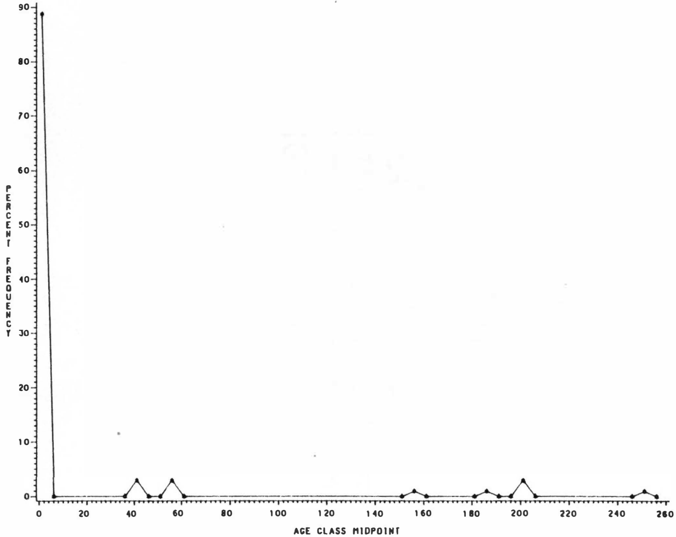
Fig. 27. Graph of yellow birch age structure.
