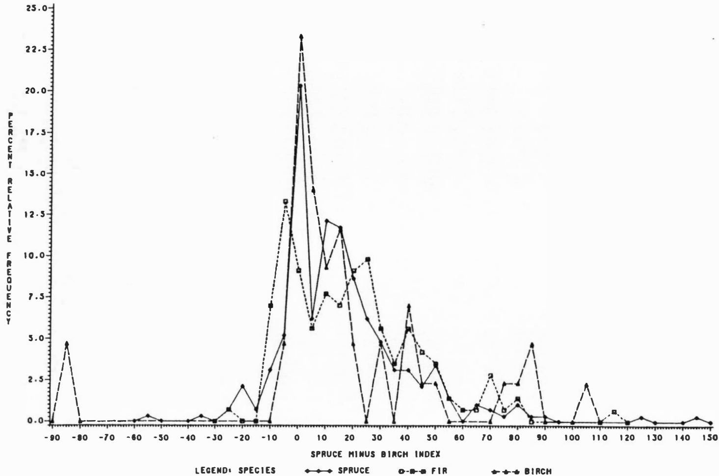
Fig. 12. Distribution of spruce, fir and birch seedlings in relation to spruce and birch canopy trees as quantified by the spruce minus birch index. No significant differences among distributions were revealed by rank-sum tests.
