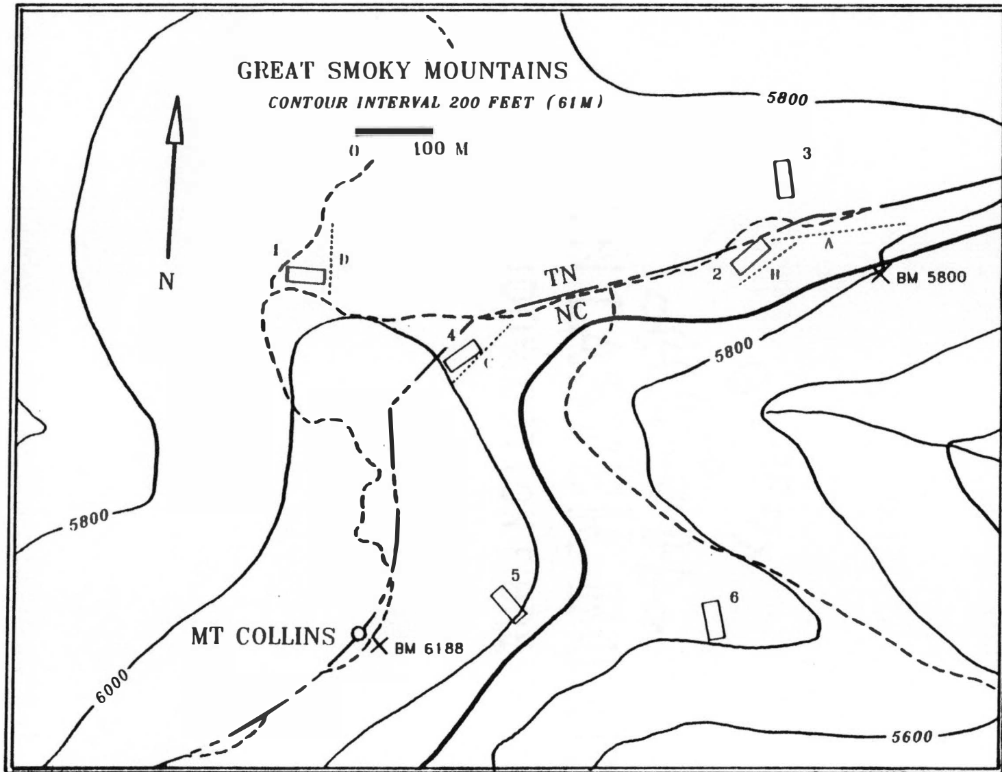
Fig. 3. Map of study area. Transects are labeled A-D, while 0.1 ha quadrats are labeled 1-6.
