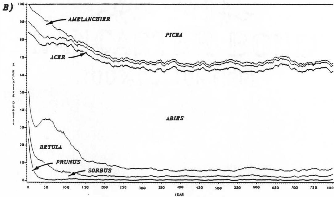
Fig. 39. Graphs of simulated density dynamics. These are: A) total density (stems > 1.27 cm DBH/ha), and B) relative density of individual species.
