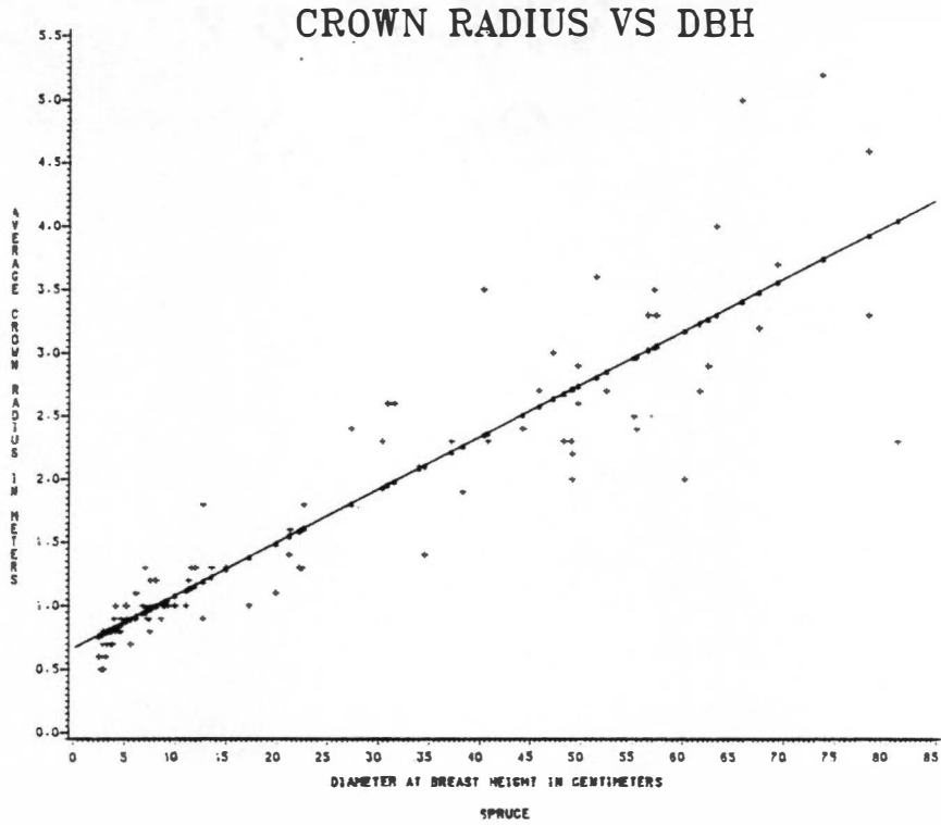
Fig. 62. Graph of red spruce crown radius vs. DBH. Linear regression r^2=0.83 .
