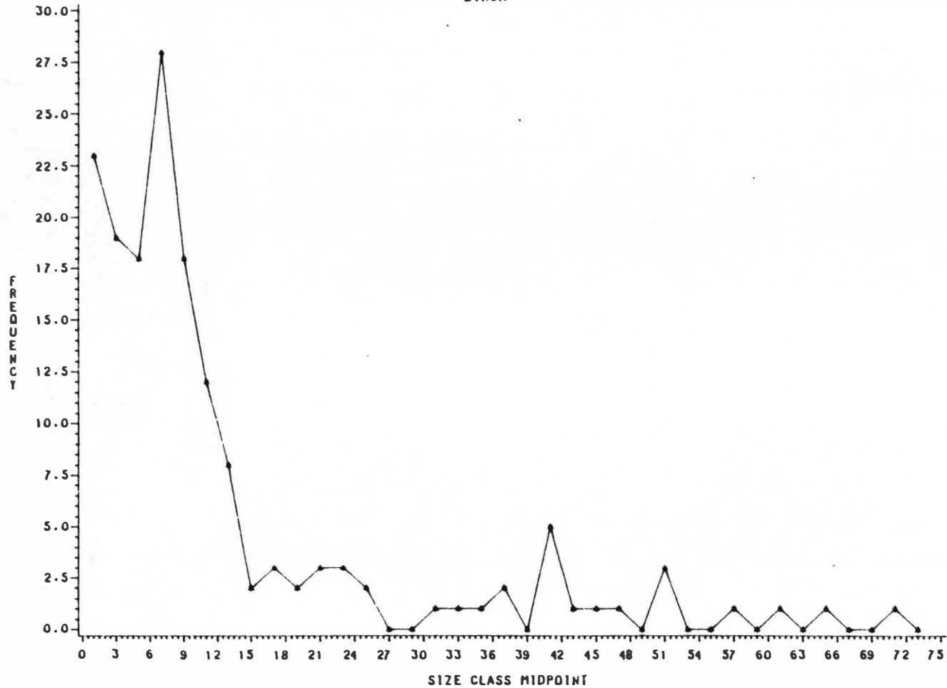
Fig. 26. Graph of yellow birch size structure. Size is in cm DBH. Individuals less than 2.5 cm DBH are not included.
