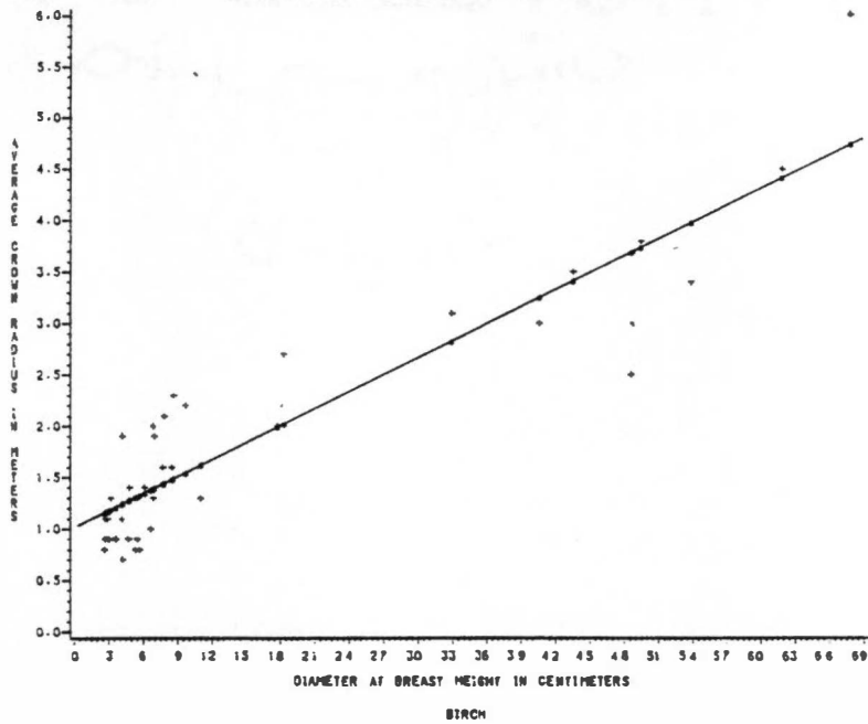
Fig. 64. Graph of yellow birch crown radius vs. DBH. Linear regression r^2=0.83 .
