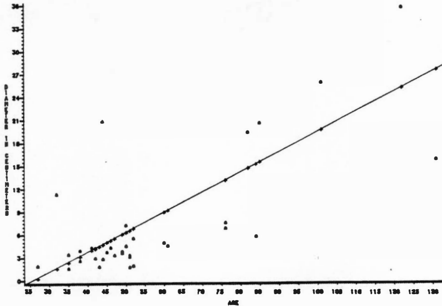
Fig. 60. Graph of Fraser fir diameter vs. age. Based on transect sampled individuals over 0 cm DBH. Linear regression r^2=0.71 .
