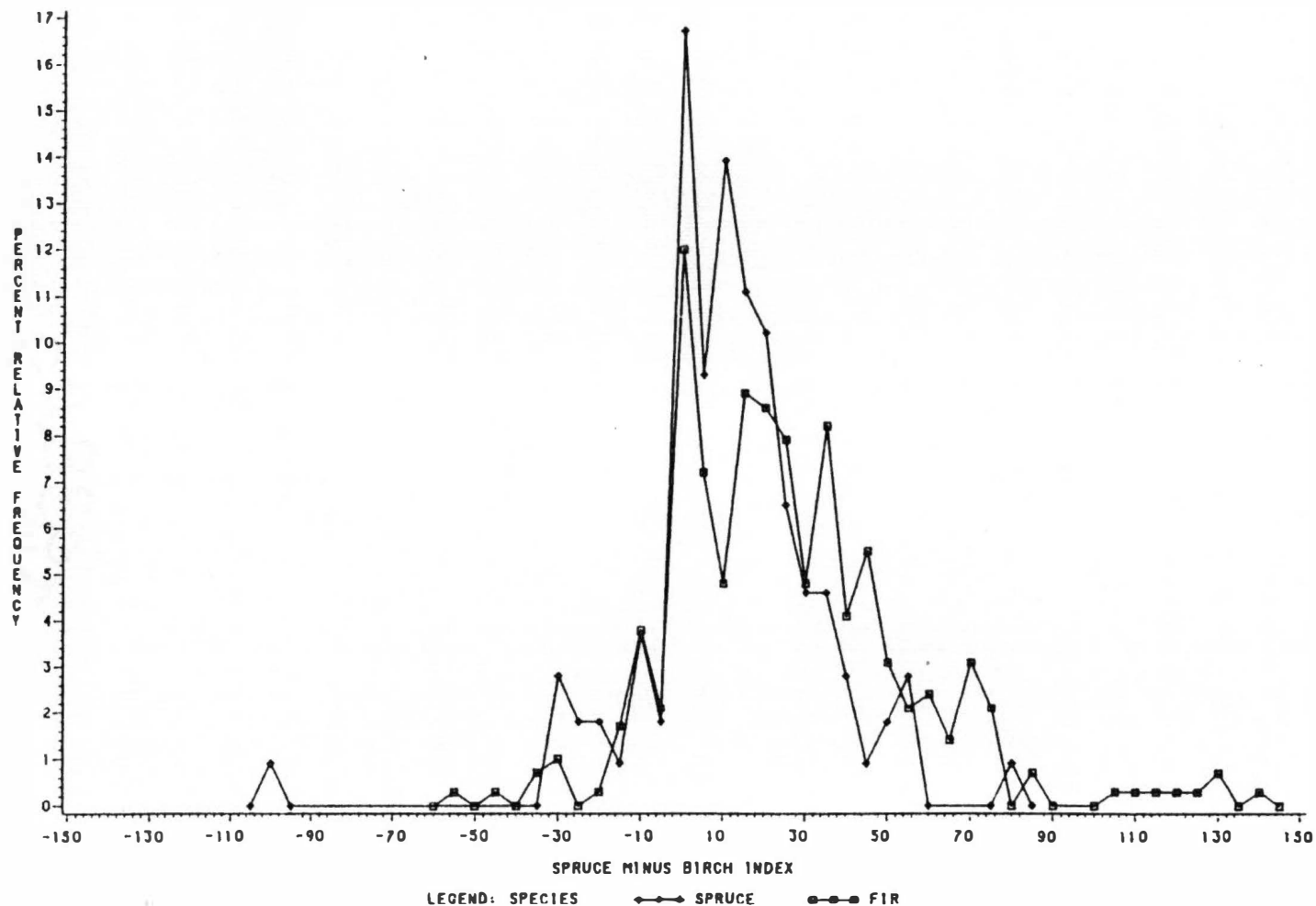
Fig. 14. Distribution of spruce and fir saplings in relation to spruce and birch canopy trees as quantified by the spruce minus birch index. A highly significant difference between distributions was revealed by the rank-sum test ( p < 0.01 ).
