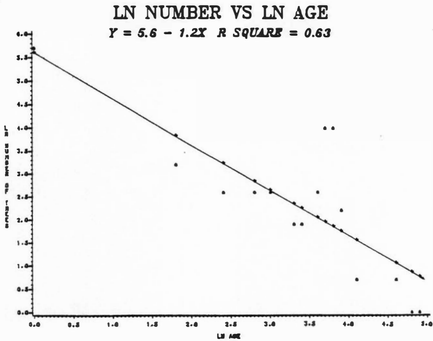
Fig. 31. Graph of Fraser fir survivorship with linear regression.
