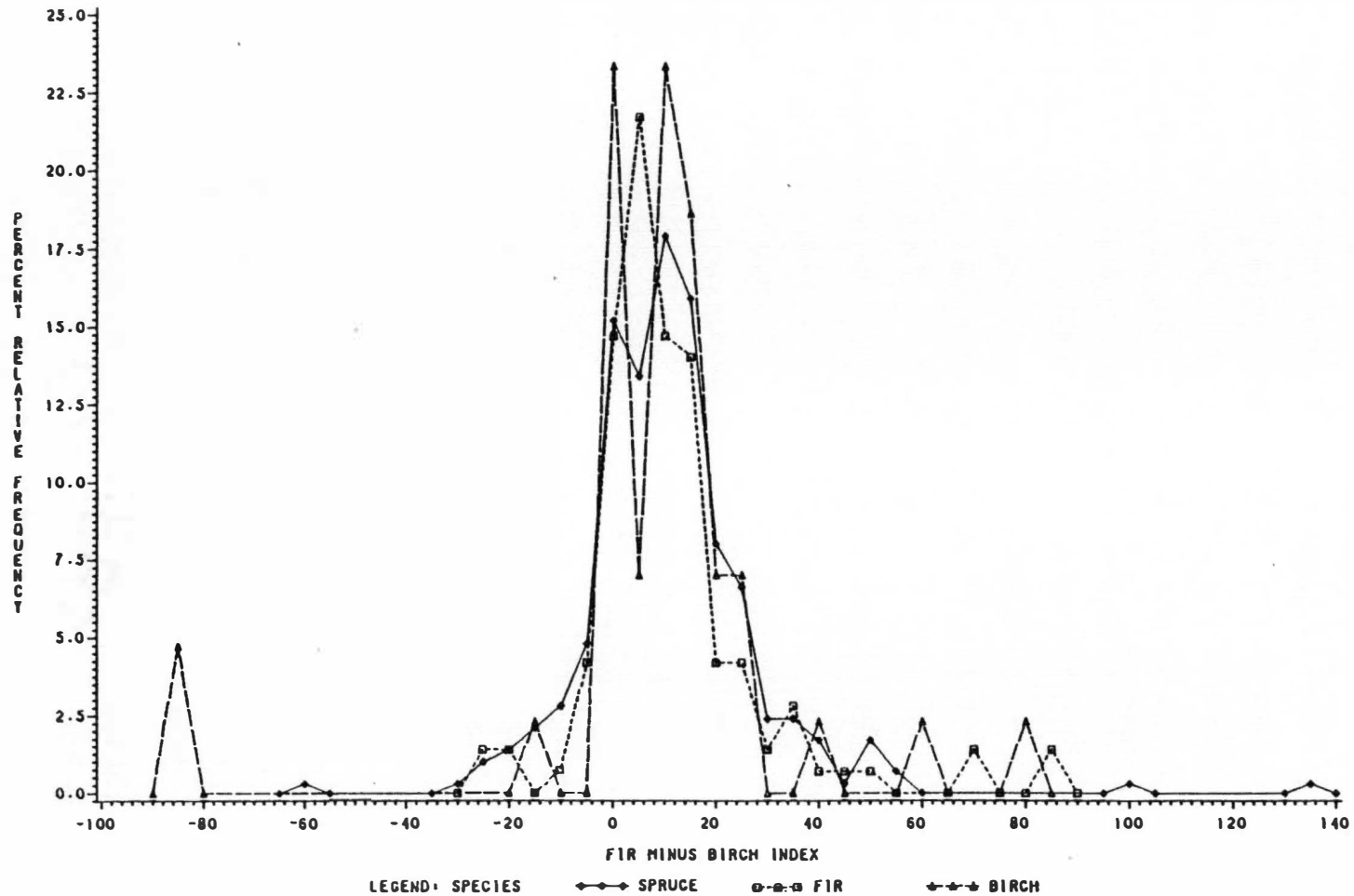
Fig. 16. Distribution of spruce, fir and birch seedlings in relation to fir and birch canopy trees as quantified by the fir minus birch index. No significant differences among distributions were revealed by rank-sum tests.
