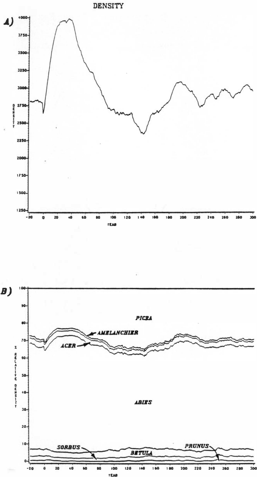
Fig. 42. Graphs of simulated density responses to continuous aphid infestation. These are: A) total stand density (stems > 1.27 cm DBH/ha), and B) relative density. Infestation begins at year 0.
