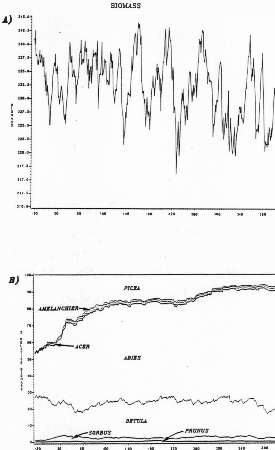
Fig. 51. Graphs of simulated biomass responses to a 30% spruce growth decline. These are: A) total stand biomass (t/ha), and B) relative biomass. Growth decline begins at year 0.
