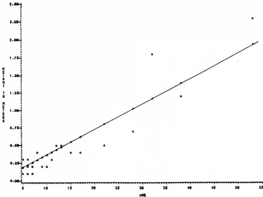
Fig. 59. Graph of red spruce height vs. age. Based on transect sampled individuals less than 2.3 m tall. Linear regression r^2=0.91 .
