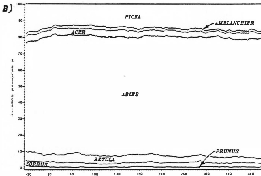
Fig. 50. Graphs of simulated density responses to a 30% spruce growth decline. These are: A) total stand density (stems > 1.27 cm DBH/ha), and B) relative density. Growth decline begins at year 0.
