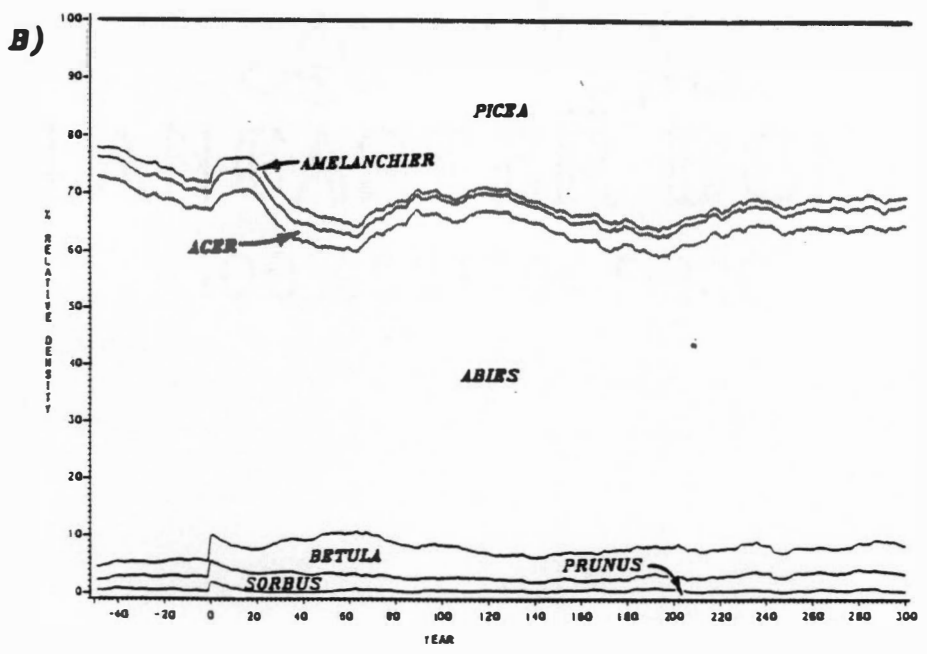
Fig. 40. Graphs of simulated density responses to logging. These are: A) total stand density (stems > 1.27 cm DBH/ha), and B) relative density. Logging occurs at year 0.
