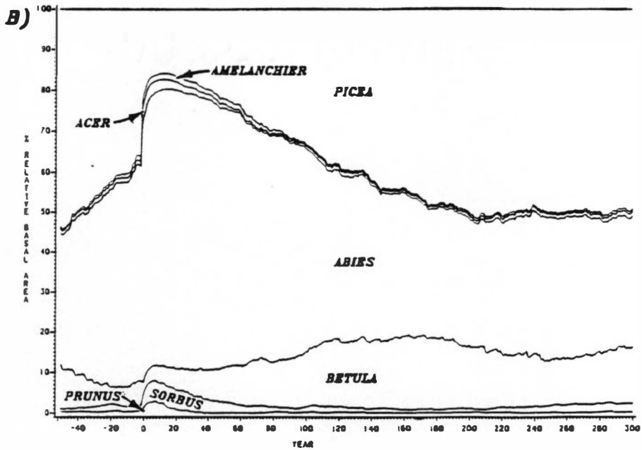
Fig. 41. Graphs of simulated basal area responses to logging. These are: A) total stand basal area ( m^2/ha ) and B) relative basal area. Logging occurs at year 0.
