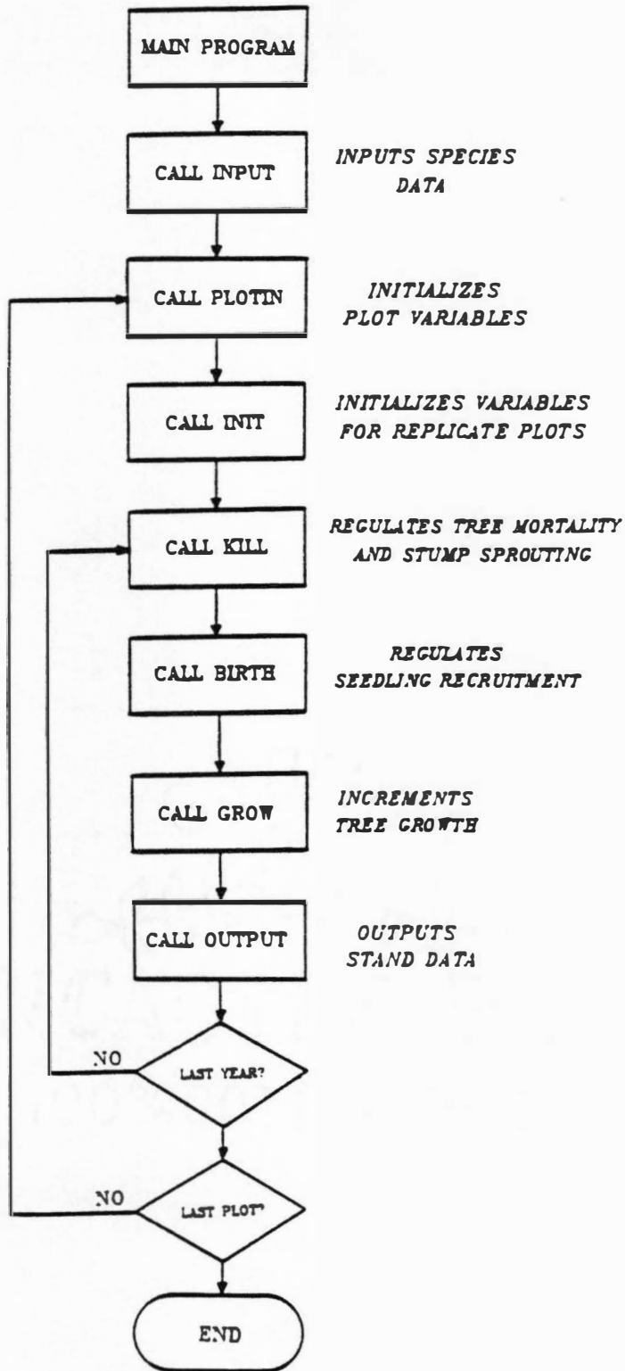
Fig. 32. Flow diagram and subroutine functions of the FORANAK model.
