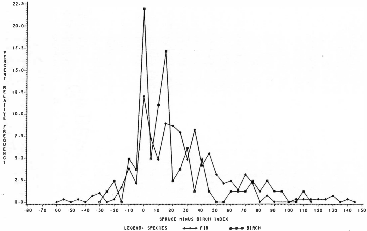
Fig. 15. Distribution of fir and birch saplings in relation to spruce and birch canopy trees as quantified by the spruce minus birch index. A significant difference between distributions was revealed by the rank sum test ( p < 0.05 ).
