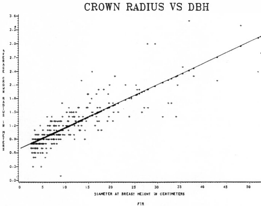
Fig. 63. Graph of Fraser fir crown radius vs. DBH. Linear regression r^2=0.69 .
