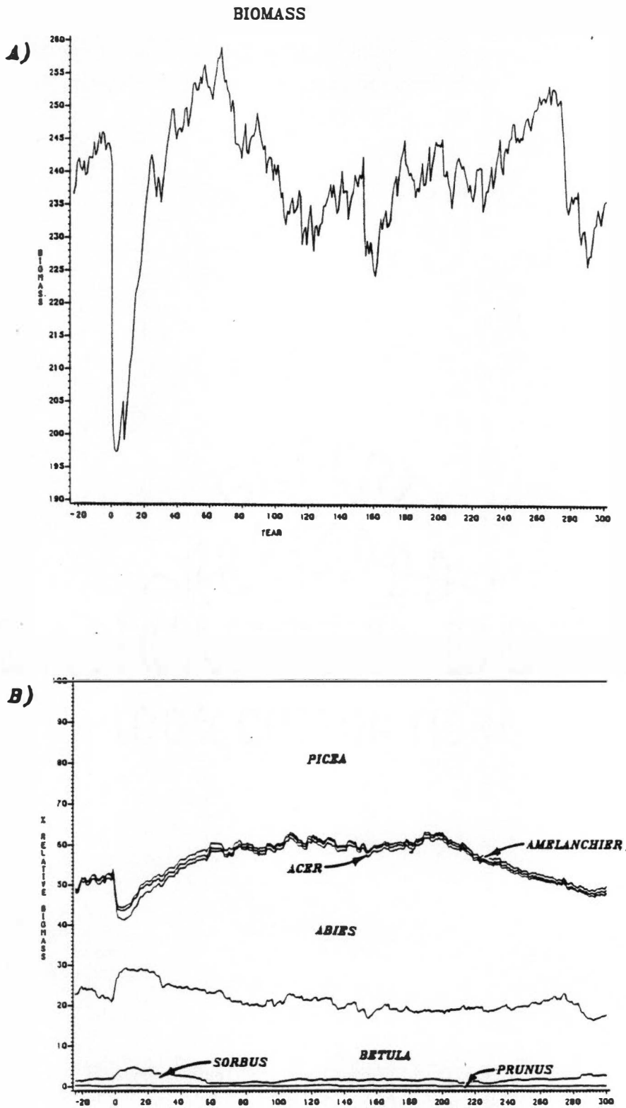
Fig. 48. Graphs of simulated biomass responses to a short-term fir infestation. These are: A) total stand biomass (t/ha), and B) relative biomass. The 10 yr infestation begins at year 0.
