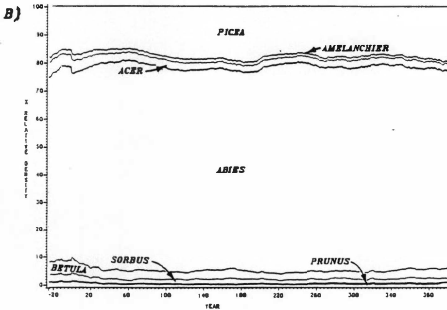
Fig. 53. Graphs of simulated density responses to continuous aphid infestation in combination with a 30% spruce growth decline. These are: A) total stand density (stems > 1.27 cm DBH/ha), and B) relative density. Disturbance begins at year 0.
