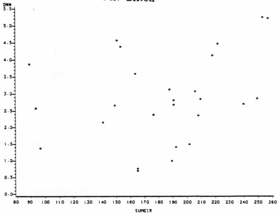
Fig. 21. Graphs of distance to nearest neighbor (m) vs. sum of trunk circumferences (cm) (birch-birch, fir-birch). Correlations of birch-birch values, and fir-birch values were both not significant.
