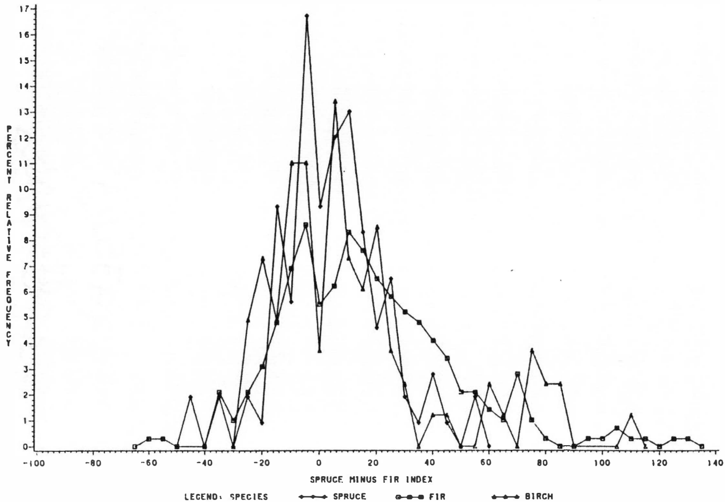
Fig. 9. Distribution of spruce, fir and birch saplings in relation to spruce and fir canopy trees as quantified by the spruce minus fir index.
