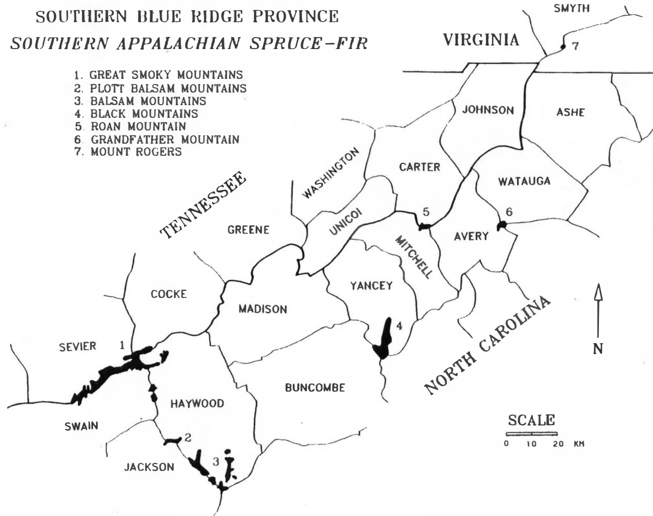
Fig. 1. Map of the present distribution of the southern Appalachian spruce-fir forest. Modified from Saunders (1979).
