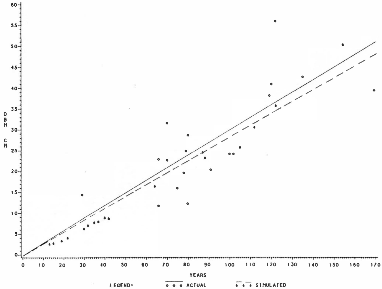
Fig. 37. Graph of simulated vs. actual Fraser fir growth rates with regression lines.
