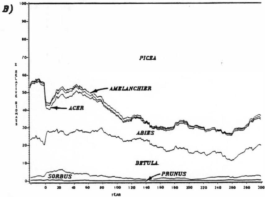
Fig. 43. Graphs of simulated biomass responses to continuous aphid infestation. These are: A) total stand biomass (t/ha), and B) relative biomass. Infestation begins at year 0.
