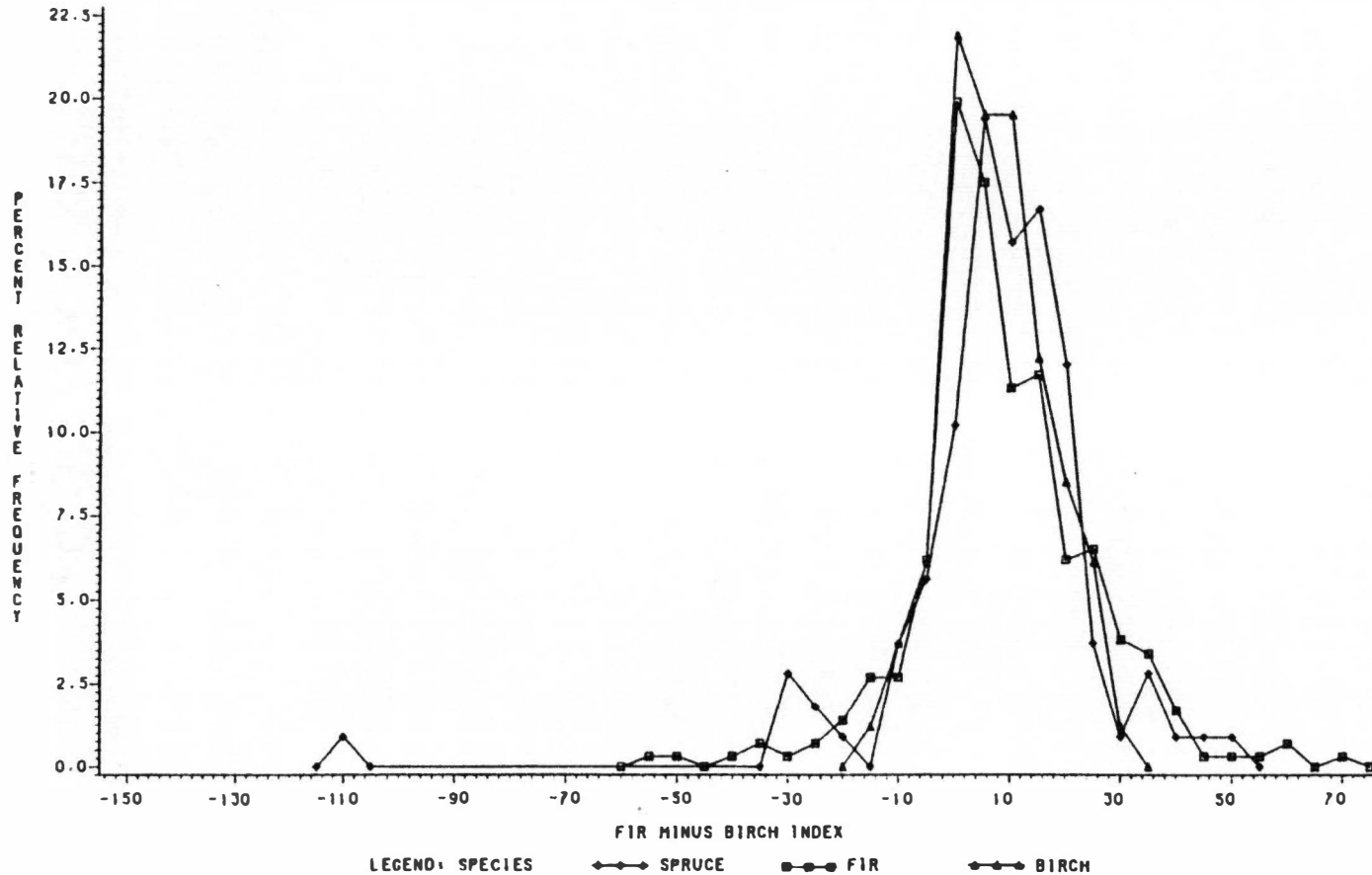
Fig. 17. Distribution of spruce, fir and birch saplings in relation to fir and birch canopy trees as quantified by the fir minus birch index. No significant differences among distributions were revealed by rank-sum tests.
