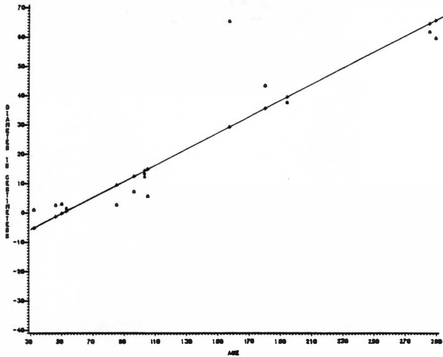
Fig. 58. Graph of red spruce diameter vs. age. Based on transect sampled individuals over 0 cm DBH. Linear regression r^2=0.79 .
