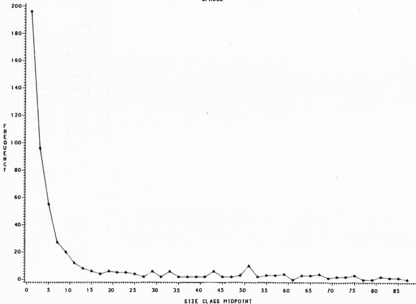
Fig. 23. Graph of red spruce size structure. Size is in cm DBH. Individuals less than 2.5 cm DBH are not included.
