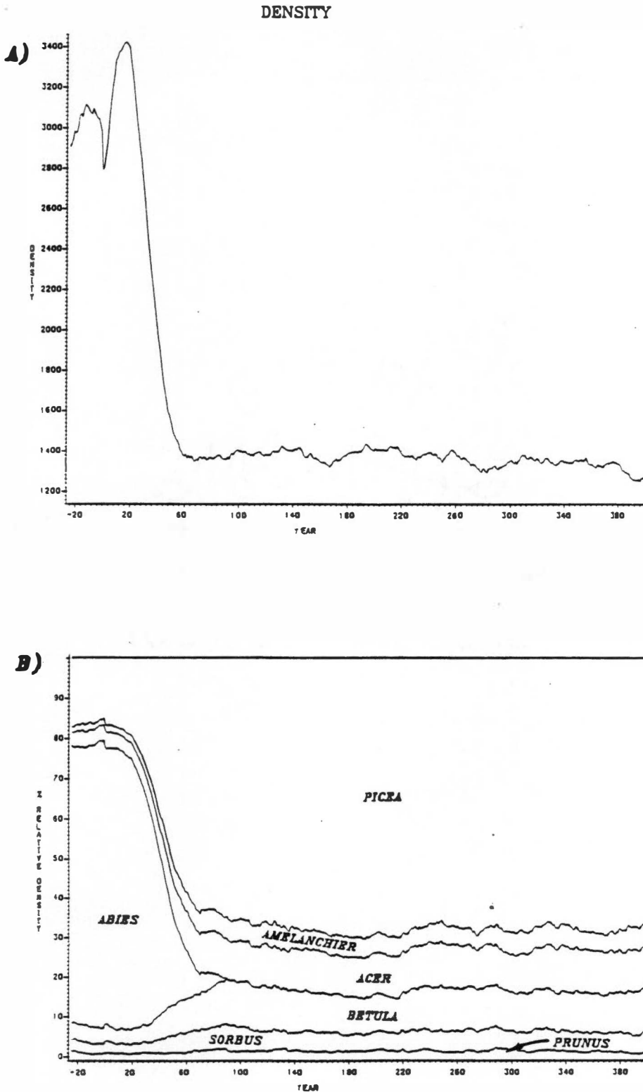
Fig. 55. Graphs of simulated density responses to the elimination of fir in combination with a 30% spruce growth decline. These are: A) total stand density (stems > 1.27 cm DBH/ha), and B) relative density. Disturbance begins at year 0.
