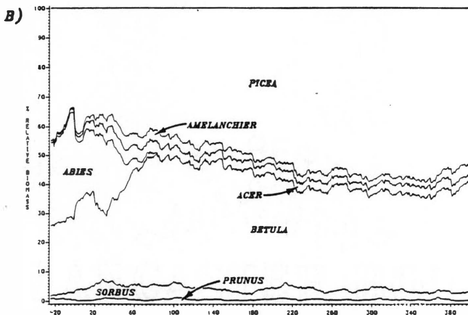
Fig. 56. Graphs of simulated biomass responses to the elimination of fir in combination with a 30% growth decline. These are: A) total stand biomass (t/ha), and B) relative biomass. Disturbance begins at year 0.
