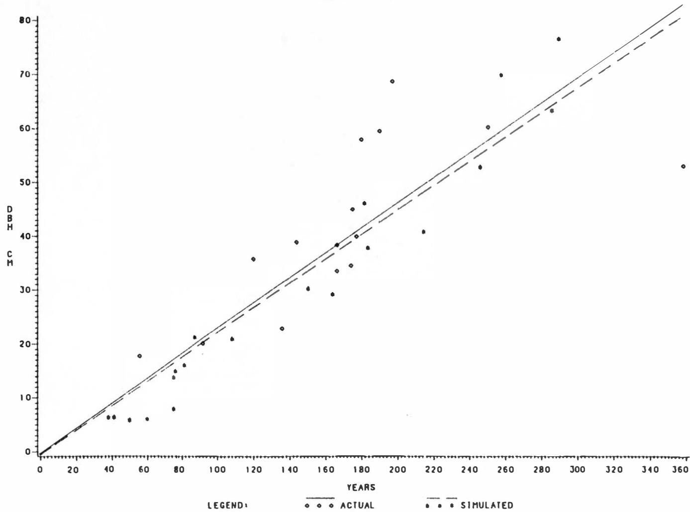
Fig. 36. Graph of simulated vs. actual red spruce growth rates with regression lines.
