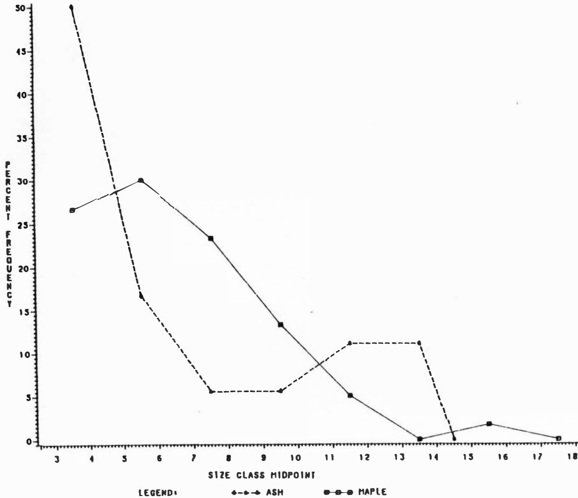
Fig. 28. Graph of mountain maple and mountain ash size structure. Size is in cm DBH. Individuals less than 2.5 cm DBH are not included.
