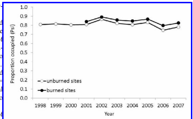
FIGURE 4. Mean annual probabilities of occupancy ( \psi ) of the California Spotted Owl at unburned sites (unfilled) from 1998 to 2007 and sites burned by fires (filled) from 2001 to 2007 in national forests in the Sierra Nevada, California. Mean annual probabilities of occupancy were derived from model-average estimates of colonization and local extinction.
