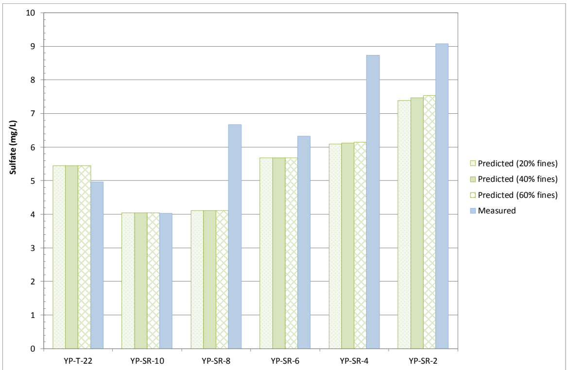
Figure F6: Grain Size Sensitivity Analysis for Predicted vs. Measured Sulfate under Average Flow Conditions
