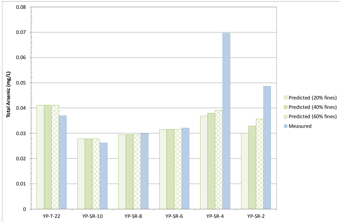
Figure F7: Grain Size Sensitivity Analysis for Predicted vs. Measured Total Arsenic under Average Flow Conditions
