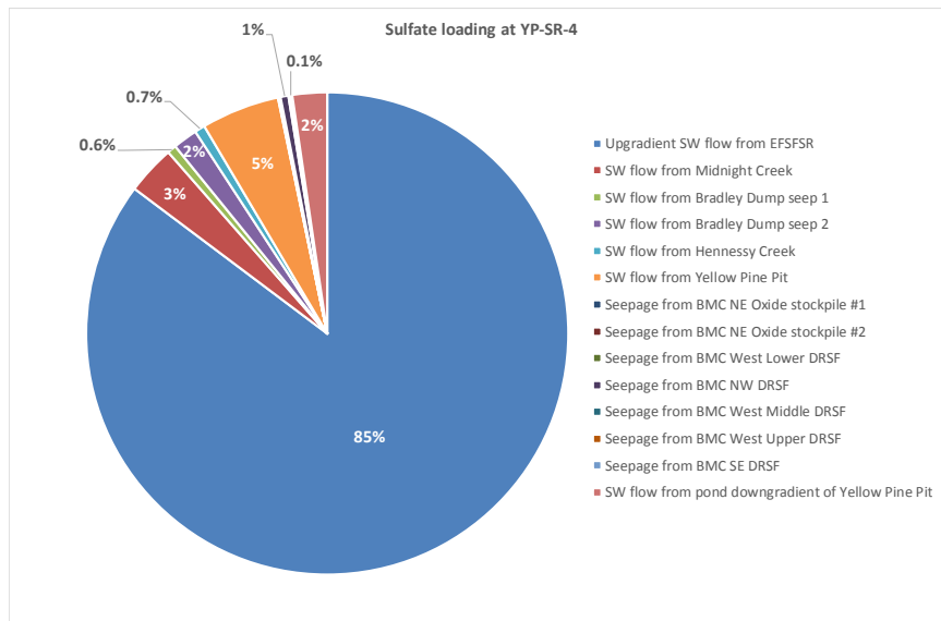
Figure D5: Total Arsenic, Total Antimony, Sulfate and Total Mercury Loading at YP-SR-4 (EFSFSR below Yellow Pine Pit)
