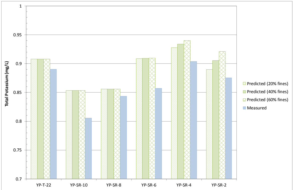
Figure F5: Grain Size Sensitivity Analysis for Predicted vs. Measured Total Potassium under Average Flow Conditions
