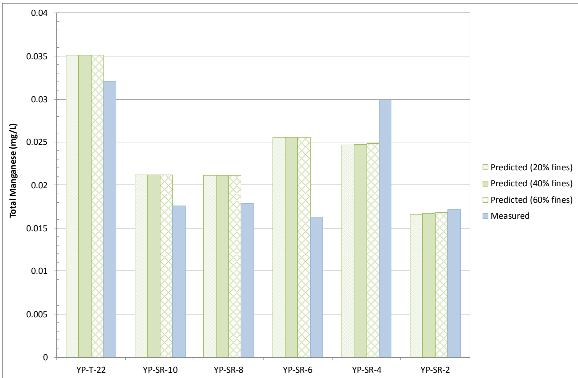
Figure F10: Grain Size Sensitivity Analysis for Predicted vs. Measured Total Manganese under Average Flow Conditions
