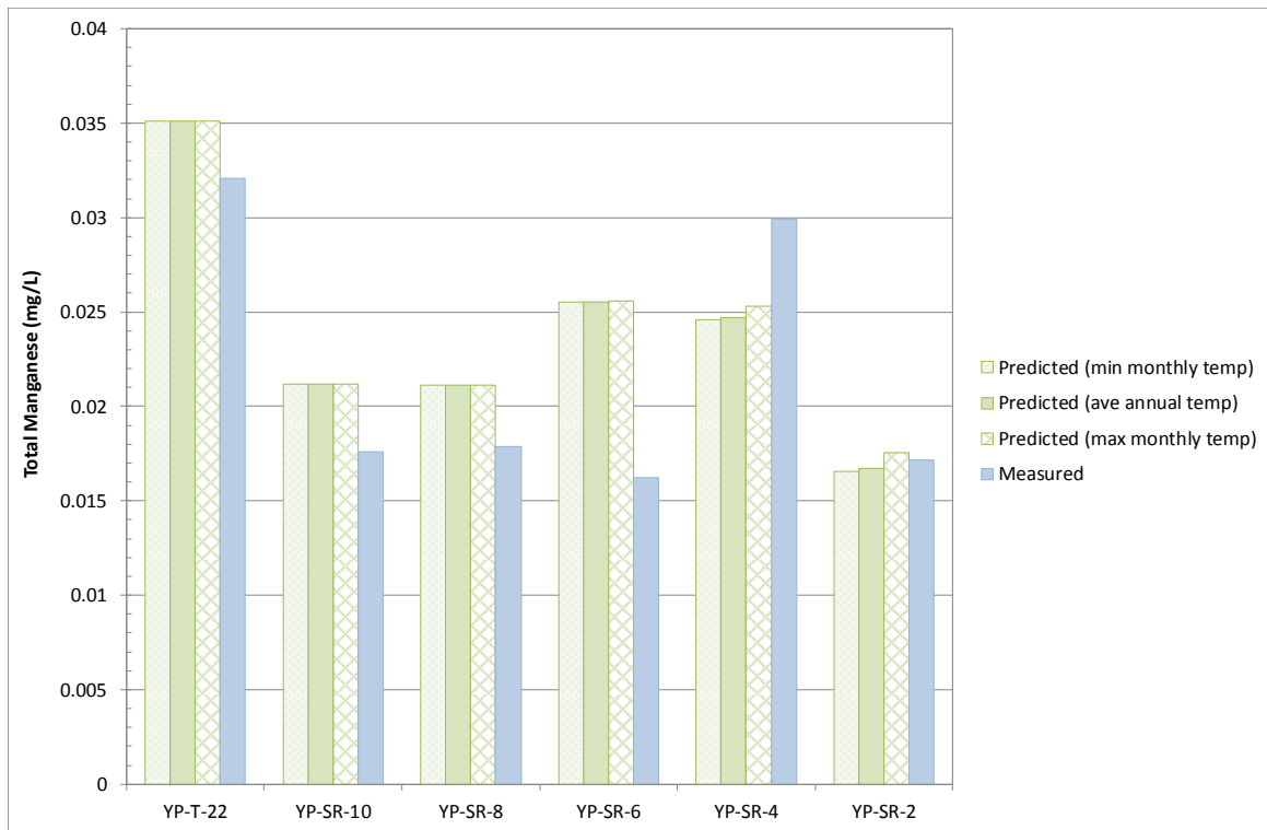
Figure E10: Temperature Sensitivity Analysis for Predicted vs. Measured Total Manganese under Average Flow Conditions
