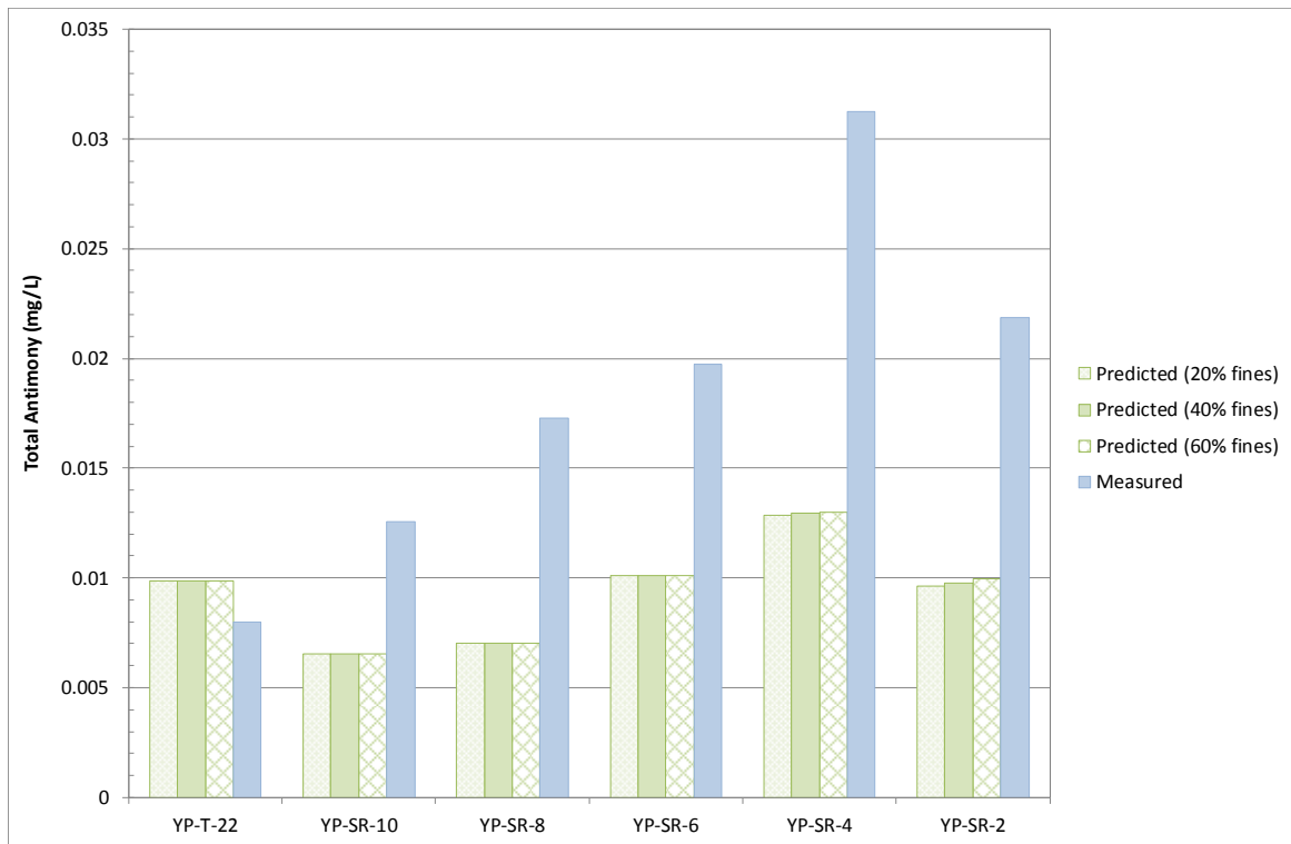
Figure F8: Grain Size Sensitivity Analysis for Predicted vs. Measured Total Antimony under Average Flow Conditions
