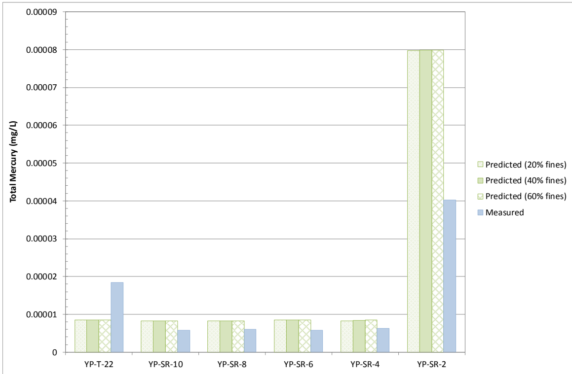
Figure F9: Grain Size Sensitivity Analysis for Predicted vs. Measured Total Mercury under Average Flow Conditions
