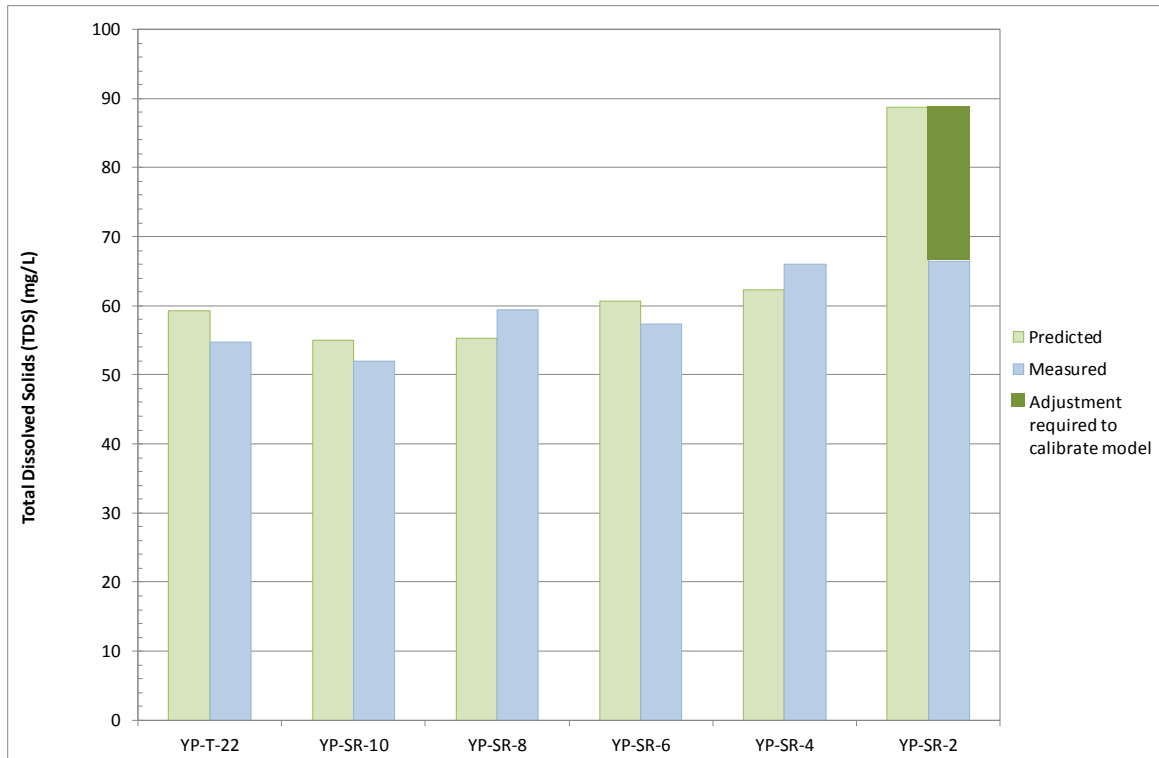
Figure 6-31: Predicted vs. Measured TDS under Average Flow Conditions
