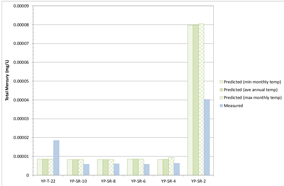
Figure E9: Temperature Sensitivity Analysis for Predicted vs. Measured Total Mercury under Average Flow Conditions
