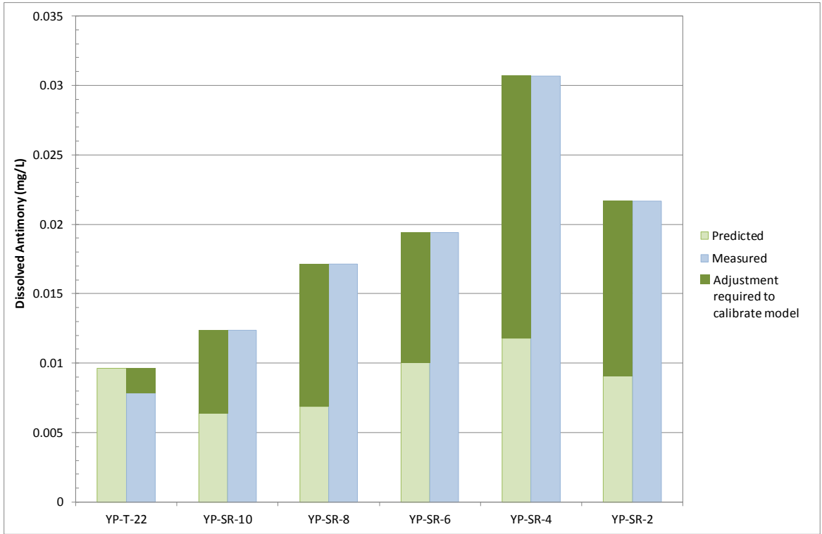
Figure 6-13: Predicted vs. Measured Dissolved Antimony under Average Flow Conditions
