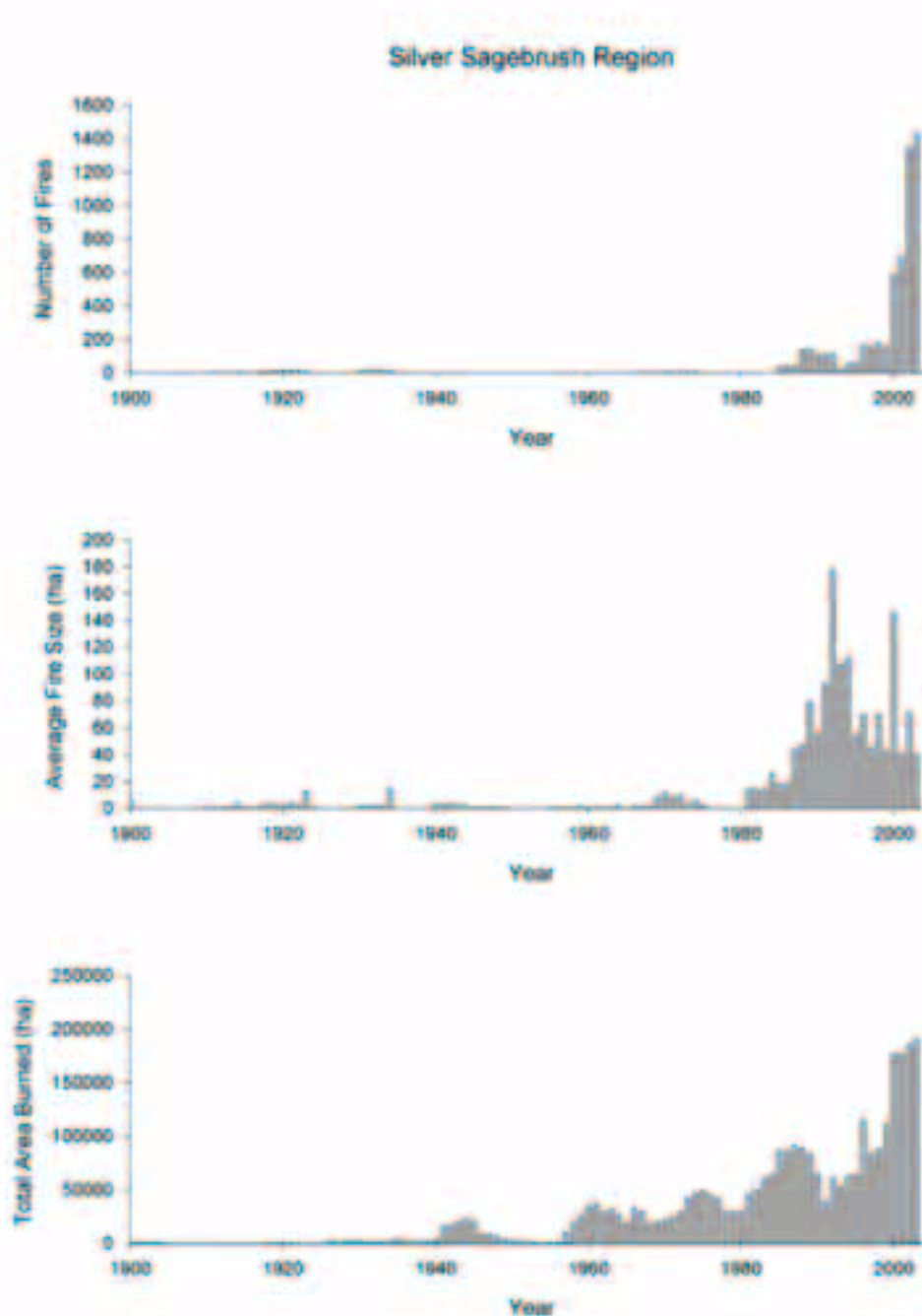
Fig. 7.3. Number of fires, average fire size (ha), and total area burned (ha) within the Silver Sagebrush division (Fig. 5.2) of the sagebrush biome. Regression models of changes in fire statistics from 1980 through 2003 are presented in Table 7.1.
