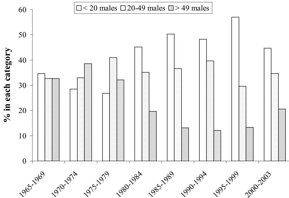
Fig. 6.7. Change in lek size class for Colorado, summarized over 5-year periods, 1965 - 2003.
