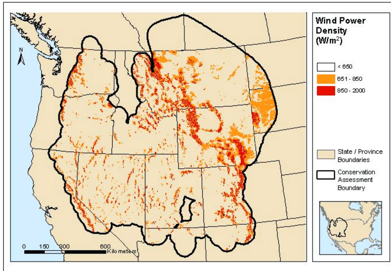
Fig. 7.31. Potential for wind energy in the western United States
