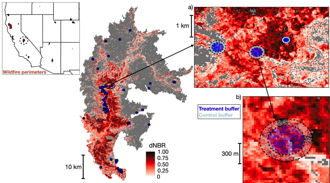
Figure 1. Approach to estimating the impact of Rx fire on burn severity, using the Creek Fire as an example. The Creek Fire perimeter contains 30 m pixels of dNBR values from Sentinel-2 with higher values in dark red indicating more severe burns. Blue dots represent Rx fire treatment locations recorded by NFPORS ( n = 59 ) from October 2018 to May 2020. Insets (a, b) show zoomed-in views of our randomly generated treatment buffers centered on the NFPORS coordinates (blue dots) and the surrounding control buffers (cyan dots).
