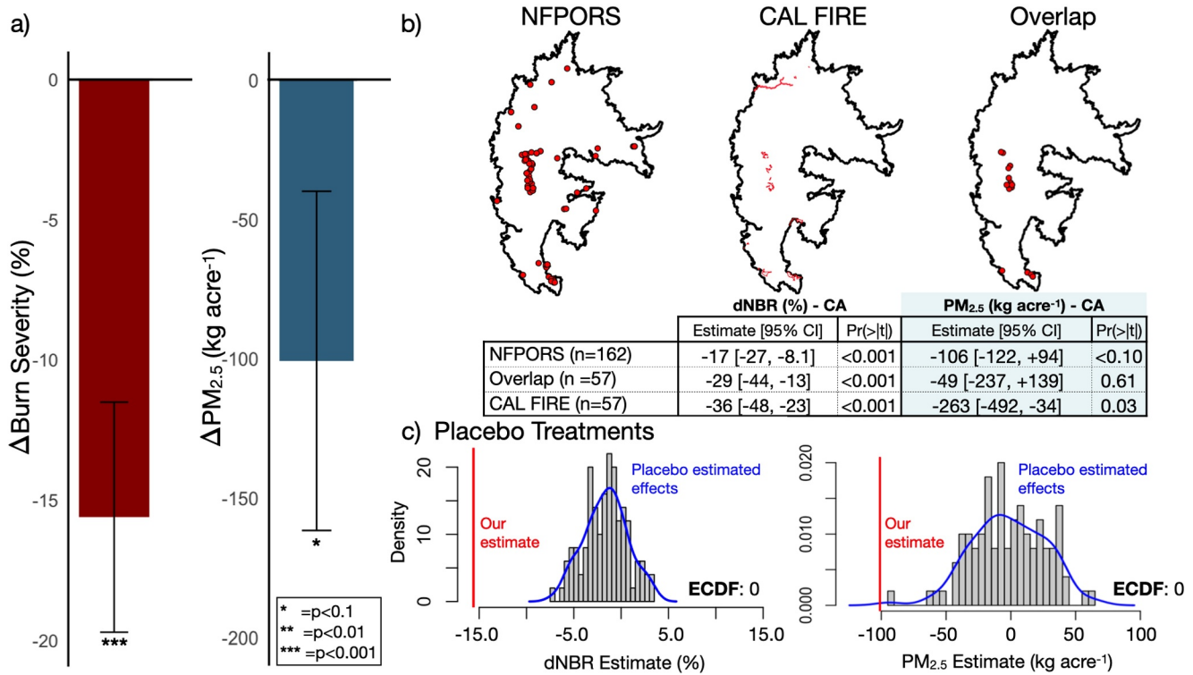
Figure 2. Impact of Rx fire treatments on burn severity in the western US and smoke emissions in California. (a) All sample estimates of burn severity and smoke PM 2.5 emissions changes in Rx fire-treated areas compared to control areas during the 2020 wildfire season. (b) Comparison of estimates using NFPORS (treatment and control circular buffers), CAL FIRE (treatment perimeters, control circular buffers), and the “overlap” (treatment and control circular buffers) subset of NFPORS inside CAL FIRE perimeters. Maps show overlaps for a single fire (Creek Fire) and the table of estimates shows pooled treatment effect estimates across all fires for which we have data. (c) Results from 100 randomized placebo treatments demonstrate that our estimates of the treatment effect of Rx fires are extremely unlikely to occur by chance ( p < 0.001 ). The blue line on the empirical cumulative distribution function (ECDF) plots outlines the distribution density and the red line corresponds to our estimates from (a).
