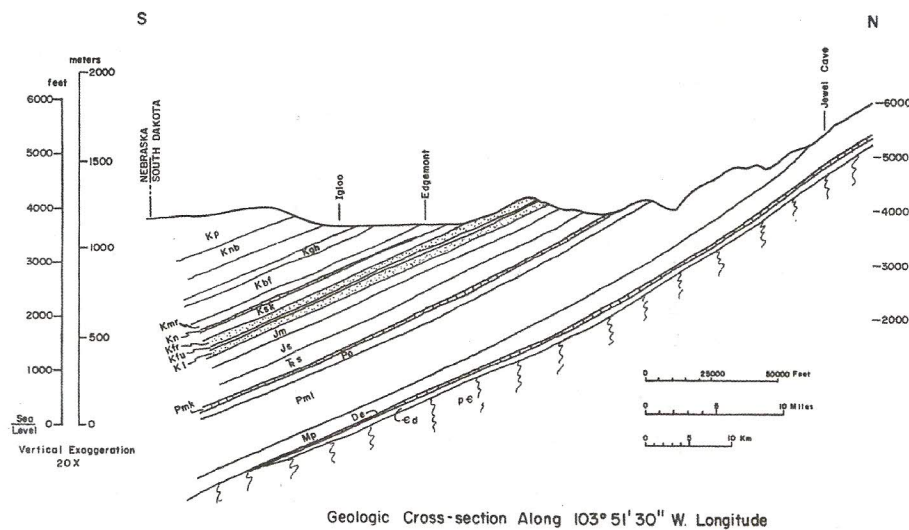
Figure 6. Geologic cross section near Edgemont, South Dakota (from Roggenthen et al. 1985). The sedimentary rocks include the Fall River Formation ( K_f ), the Lakota Formation ( K_l ) and the Pahasaapa Limestone ( M_p ).
