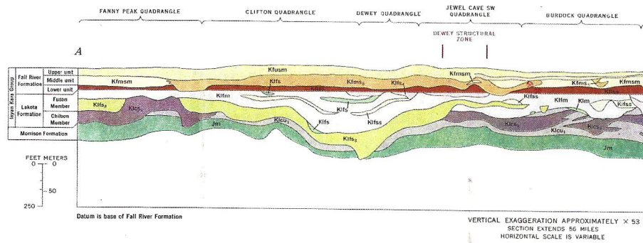
Figure 2. Diagrammatic geologic cross section showing stratigraphy of the Inyan Kara Group in the southern Black Hills (from Gott et al. 1974). The Fall River Sandstone is shown as Kfms, and the Chilson sandstone member of the Lakota Formation is shown as Klcs. The two main sandstone units show great variability in thickness from the Wyoming border through the Dewey, Burdock and Edgemont areas.
