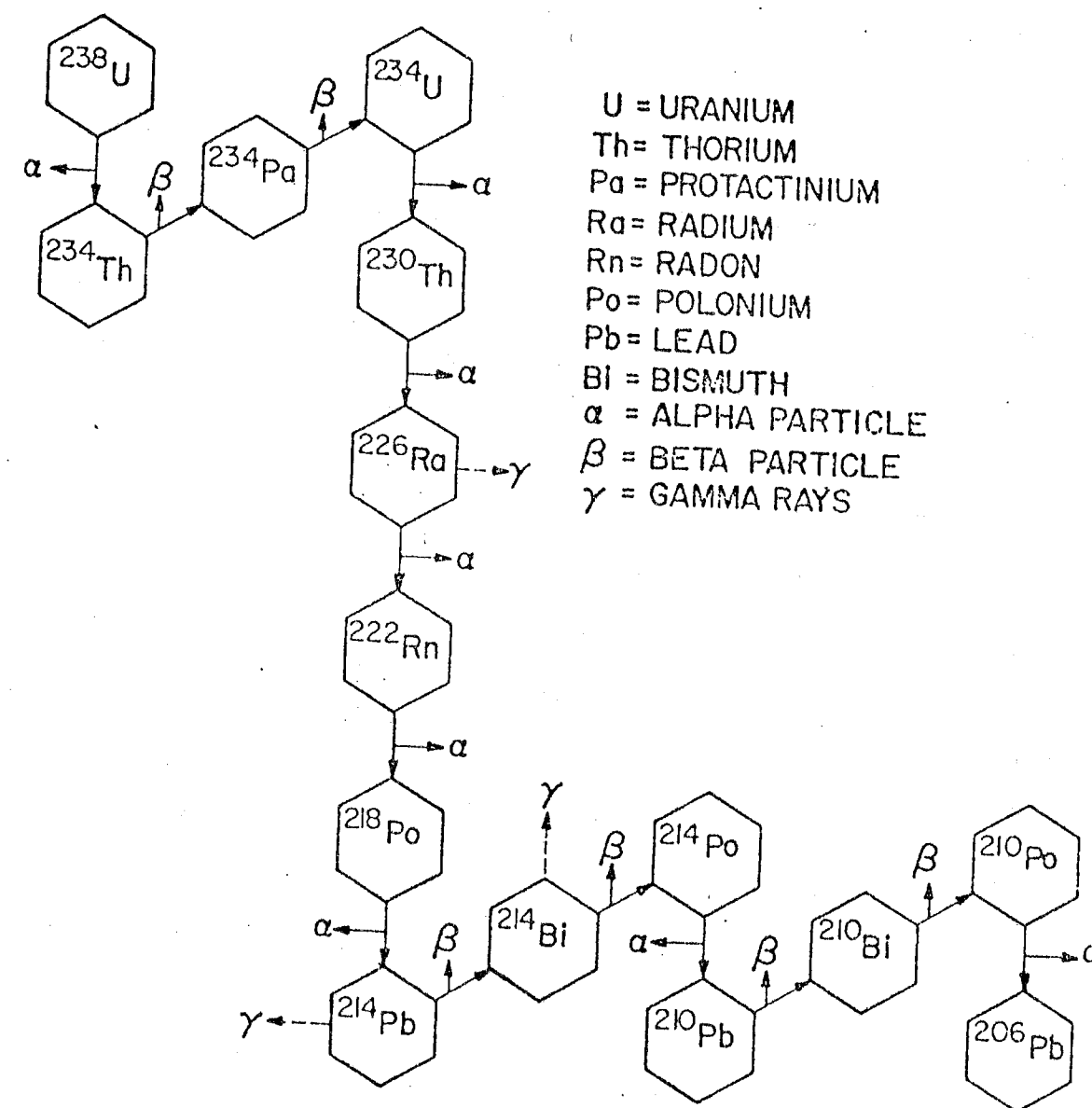
Figure 19 - Principal Branch of Uranium-238 Decay Series (DOE, 1979)
