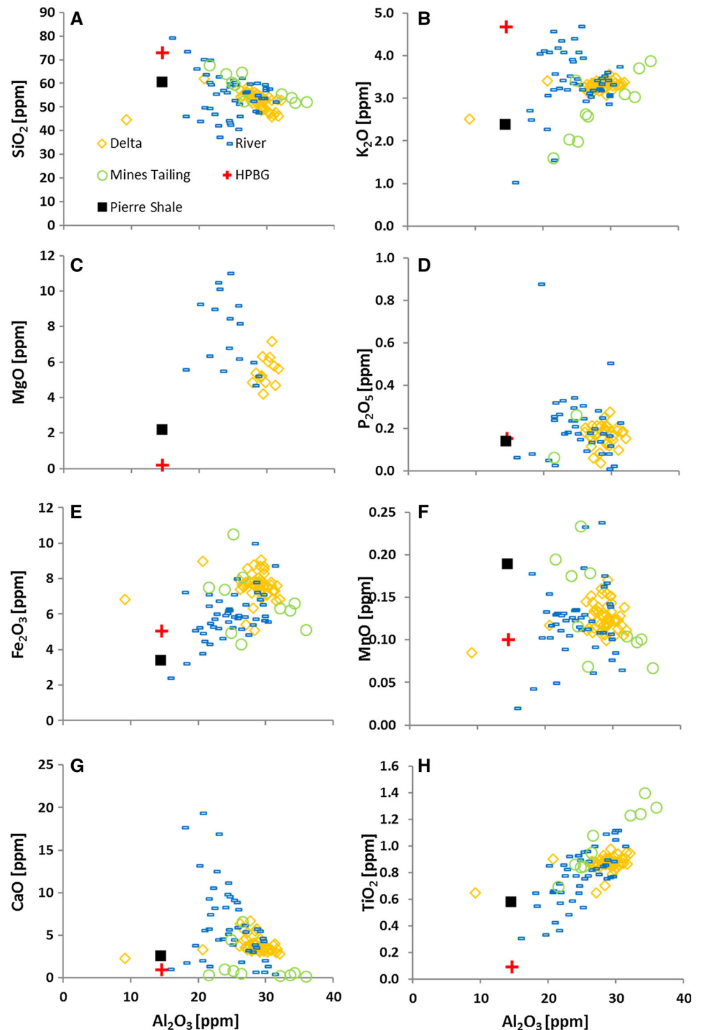
Fig. 3 a \text{SiO}_2 , b \text{K}_2\text{O} , c \text{MgO} , d \text{P}_2\text{O}_5 , e \text{Fe}_2\text{O}_3 , f \text{MnO} , g \text{CaO} , h \text{TiO}_2 compared to \text{Al}_2\text{O}_3 for the study samples. Red “+” reference Harney Peak Biotitic Granite (HPBG)
