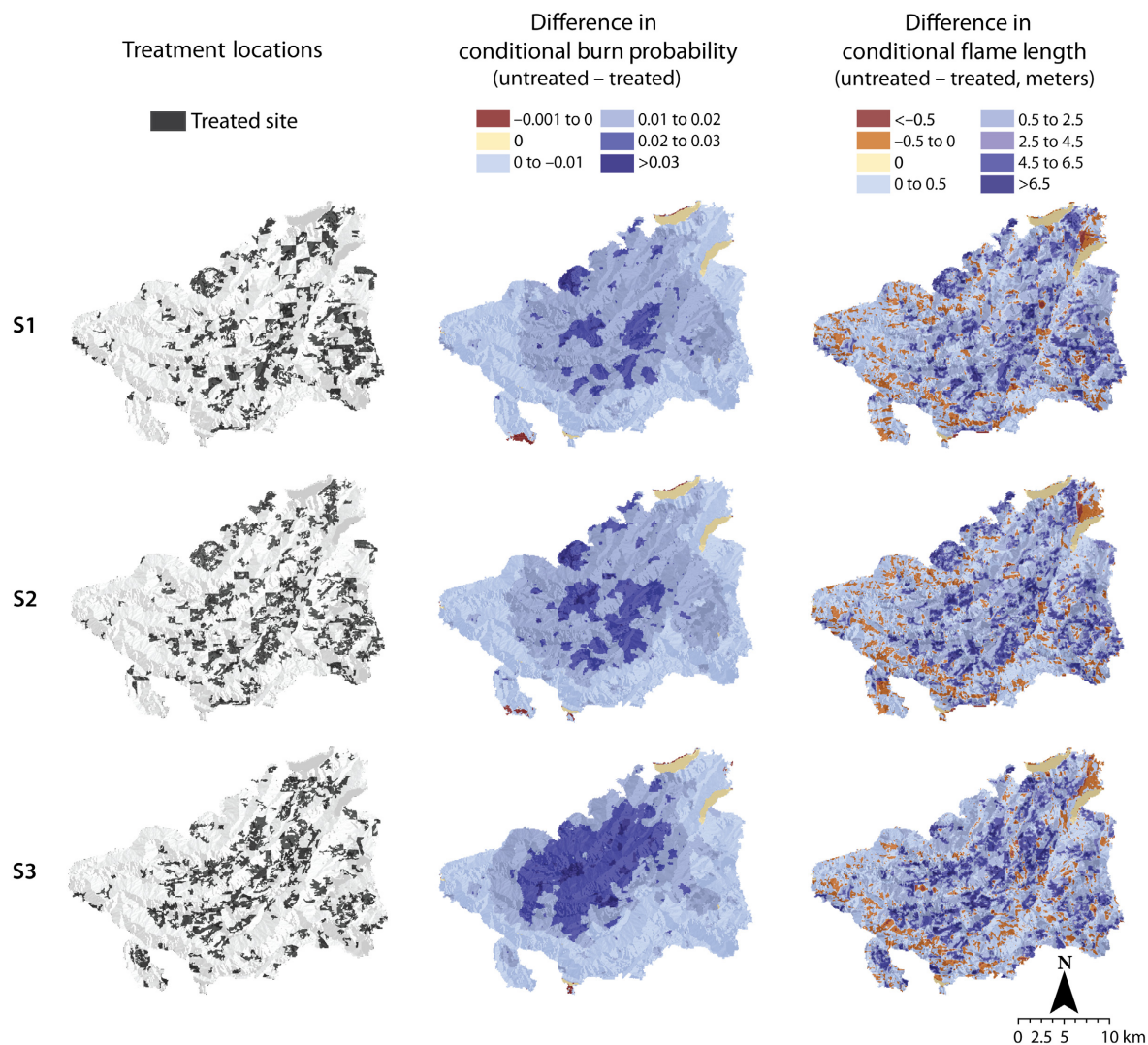
Fig. 5. Treatment locations and high fuel model range difference in conditional burn probability and conditional flame length (untreated-treated) for each treatment scenario.
