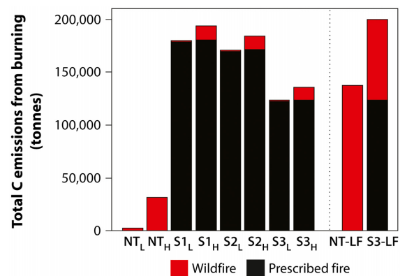
Fig. 7. Carbon emissions (tonnes) from wildfire and prescribed burning. X-axis labels indicate no-treatment (NT) and treatment scenarios (S1–S3); subscripts denote fuel model ranges used in fire modeling (L: low, H: high). Large fire scenarios, which were modeled with the high fuel model range only, are indicated by LF.
