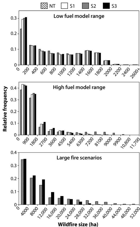
Fig. 6. Wildfire size relative frequency distributions from wildfire simulations. Bar color represents no-treatment (NT) and treatment scenarios (S1–S3).
