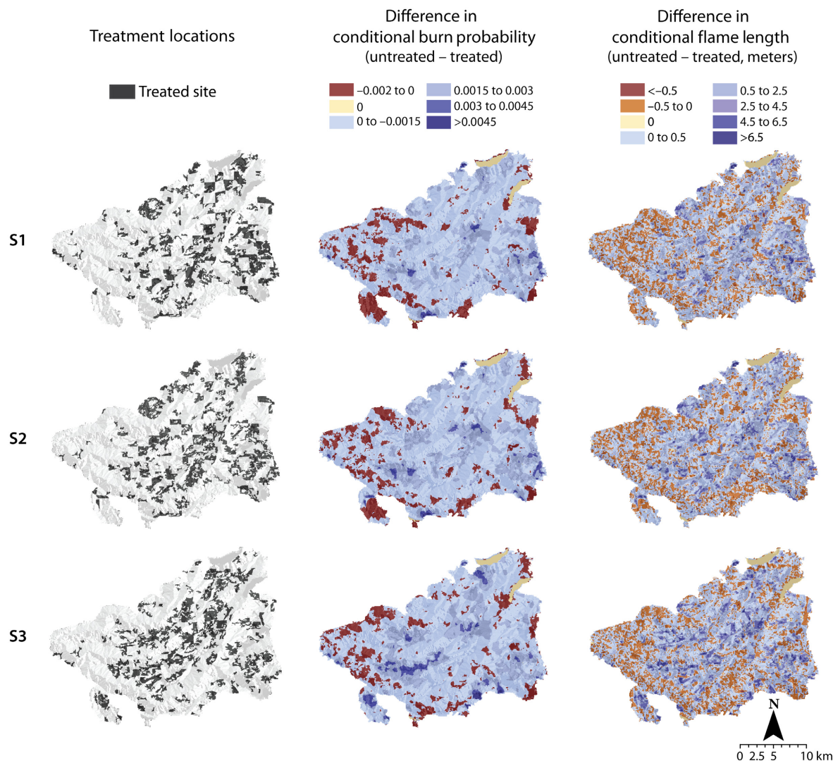
Fig. 4. Low fuel model range treatment locations and difference in conditional burn probability (CBP) and conditional flame length (CFL) (untreated–treated) for each treatment scenario. Negative values indicate an increase in CBP or CFL, while positive values represent a reduction. CBP is the likelihood that a pixel will burn given a single ignition on the landscape and assuming the simulation conditions described in Appendix S1: Table S1 and in the text. Conditional flame length is the probability-weighted flame length, given these same assumptions.
