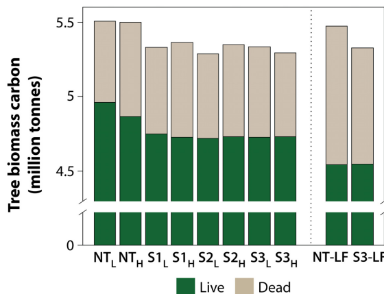
Fig. 8. Expected carbon contained in aboveground live and dead tree biomass. Expected C is that remaining in the core study area following treatment (if applicable) and a single random ignition within the larger buffered study area. X-axis labels indicate no-treatment (NT) and treatment scenarios (S1–S3); subscripts denote fuel model ranges used in fire modeling (L: low, H: high). Large fire scenarios, which were modeled for the high fuel model range only, are indicated by LF.
