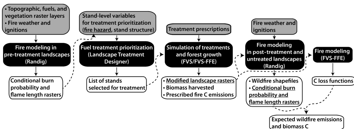
Fig. 3. Work flow used in the present study to evaluate landscape fuel treatment effects on wildfire hazard and carbon pools and emissions.
