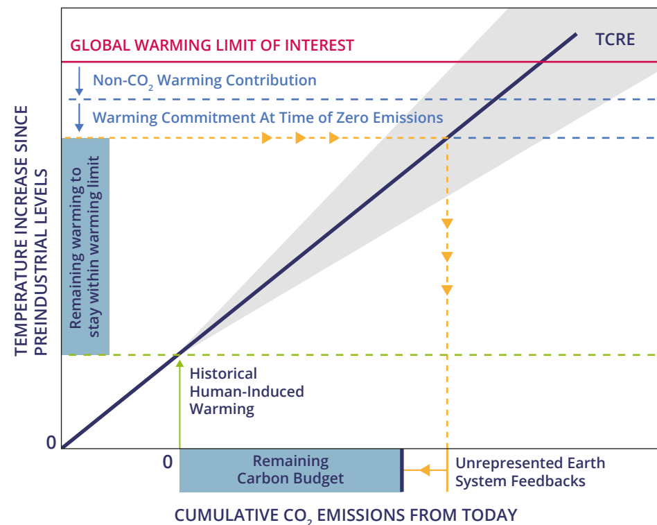
FIGURE 1: A schematic representation of the methodological approach used to derive the remaining carbon budget and related uncertainties. The various components like Transient Climate Response to Cumulative Emissions of CO 2 (TCRE) are explained in Scientific Background 1. Figure based on (5).
