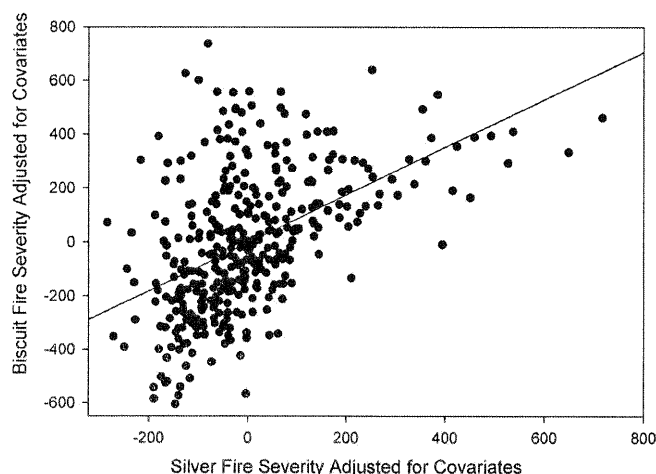
Fig. 2. Added variable plot displaying the relationship between Silver and Biscuit Fire severity as estimated through a Landsat-derived burn metric, dNBR. The effect of elevation, slope, PAG, day-of-burn, 1986 greenness, and topographic position on Biscuit Fire severity has been removed to illustrate the association between fire severities from both fires. See Table 2 for descriptions of the covariates.
