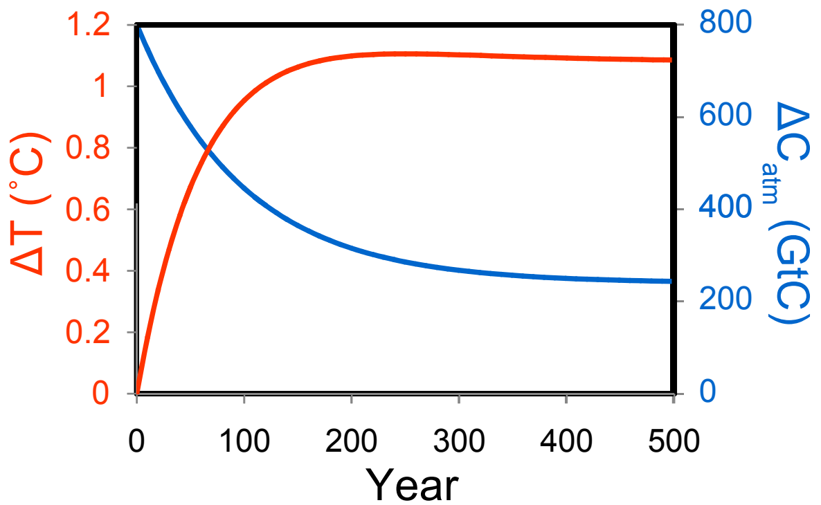
Figure S1: Result for representative values as described in the text. The blue line (right axis) shows GtC in the atmosphere after an 800 GtC release at time zero. The red line (left axis) shows temperature change. Following a release of CO 2 , atmospheric CO 2 concentrations diminish as the Earth warms.
