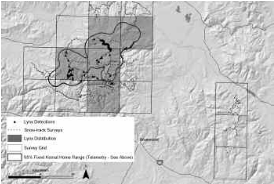
FIGURE 2. The local distribution of lynx in the Garnet Range delineated from: (A) radio telemetry of all individuals combined (95% fixed kernel, n = 96 locations from 7 individuals, \bar{z} = 13 locations per individual) compared to, (B) the local distribution based on sample units with track detections.
