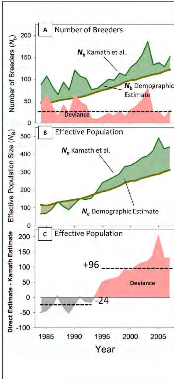
Figure 30. The panels at left illustrate discrepancies between (A) numbers of breeder ( N_b ) and (B-C) effective population sizes ( N_e ) estimated by Kamath et al. (2015) from genetic data versus results for the same calculated directly from demographic data (see below for details). All demographic results are based on population estimates reported by Van Manen et al. (2023a). The trend lines in (A) show numbers of breeders from Kamath et al in bright green and demographic estimates in dusky green. The red shaded area in (A) shows the numeric discrepancy between these two estimates. Estimates from Kamath et al. are consistently higher, especially during 1984-1993. Panel (B) shows trend lines in the same colors for the two sources but comparing estimates of effective population size ( N_e ). Estimates by Kamath et al. for N_e were similar to those derived from numbers of reproductive-aged bears in the population during 1984-1993 but exhibited a rapid comparative escalation after 1995. Panel (C) shows this deviation, with discrepancies averaging -24 during 1984-1993 and +96 during 1995-2007, comparable to the trend shown for N_e/N_b in Figure 29.
