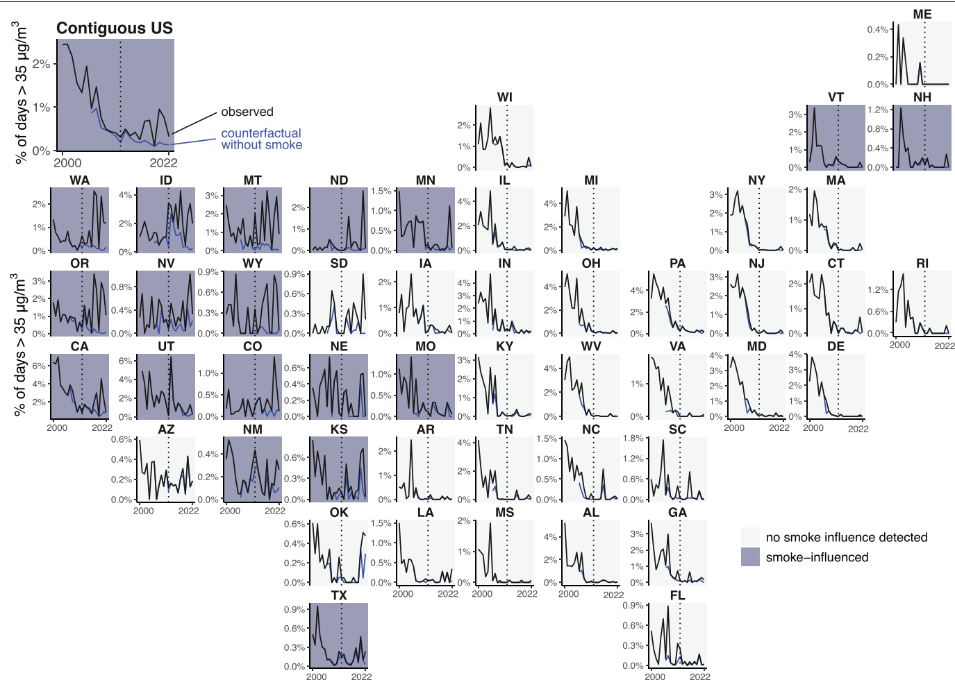
Extended Data Fig. 3 | Influence of wildfire smoke on daily PM_{2.5} extremes is mainly concentrated in states in the West, Northwest, and Great Plains.
