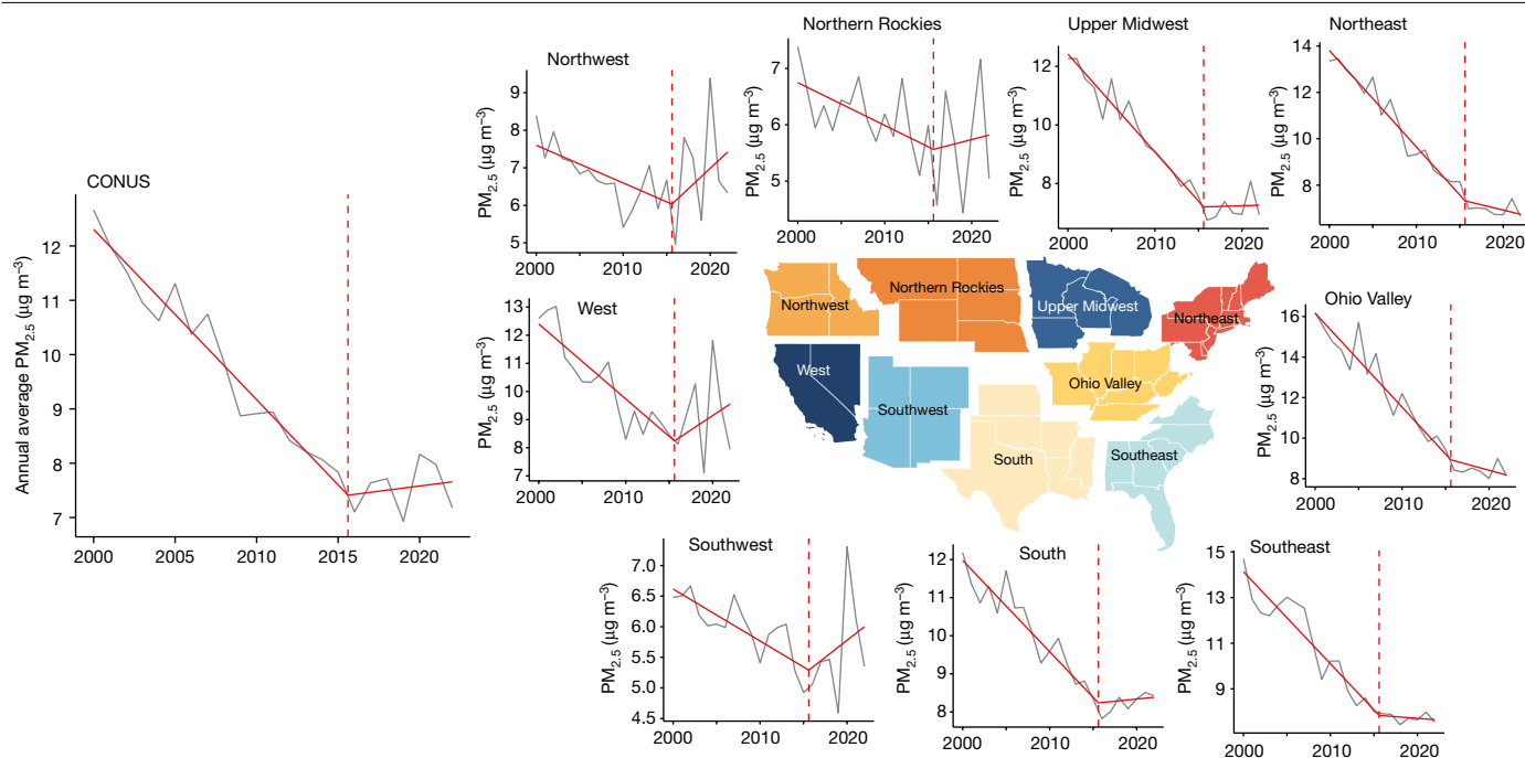
Fig. 1 | National and regional trends in ambient concentrations of \text{PM}_{2.5} show steady declines through 2016 and then stagnation or reversal. Grey lines in each subplot are annual average regional or CONUS concentrations of \text{PM}_{2.5} averaged over monitoring stations reporting consistently over the period in each US climate region 32,33 . Regional and national averages are computed
