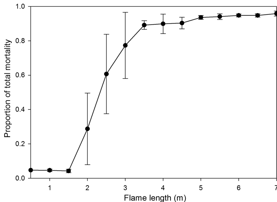
Fig. 5. Mortality of old growth ponderosa pine as a function of flame length for modeled fire behavior in untreated stands. Data obtained from simulations of the 16,632 stands in the study area using conditions described in the text. Bars are standard deviation for 0.5 m flame length intervals.
