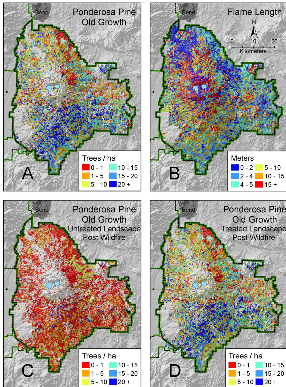
Fig. 4. Maps showing modeled outputs: (A) Predicted tree density of ponderosa pine old growth (PPOG), (B) potential flame length from a modeled wildfire (untreated), (C) predicted PPOG after a wildfire (untreated), and (D) predicted PPOG after treatment and wildfire. Wildfire weather conditions assume 97th percentile conditions as determined from local weather data.
