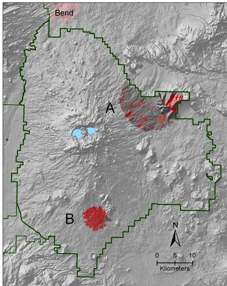
Fig. 7. Project areas and suggested treatment locations for two model simulations. The northern project area resulted from optimizing expected PPOG for a 6.5 m flame length threshold and 3000 ha treatment allowance, while the southern project area resulted from a 3 m flame length threshold and the same treatment allowance. Areas shaded in red were selected for treatment based on the expected flame length exceeding the threshold established in the simulation. Areas in dark gray are within the project areas but were not selected for treatment.
