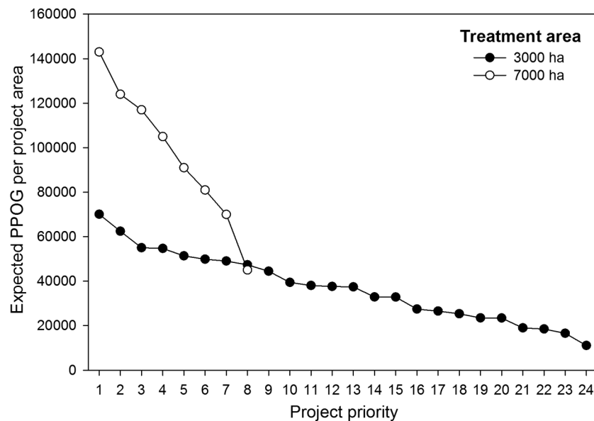
Fig. 9. Expected ponderosa pine old growth (PPOG) per project area for the two simulations shown in Fig. 8. Project priority refers to the restoration priority, as determined by iteratively executing the optimization process and removing the optimum project areas from consideration. Project priority values correspond to Fig. 8.
