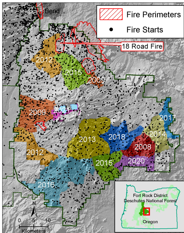
Fig. 2. Map of the study area showing past and proposed project area boundaries (solid colored polygons). Perimeters for recent (1990–2012) wildfires are red hatched polygons. Historical ignition points (1970–2010) are black dots.
