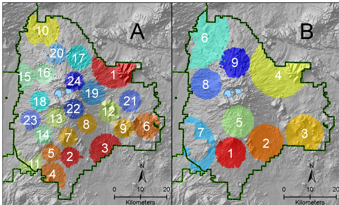
Fig. 8. Results of recursive simulations to prioritize the entire study area into a sequence of project areas. Ranked projects with (A) 3000 ha treatment allowance and 4 m flame length (FL) threshold, and (B) 7000 ha treatment allowance and 4 m FL threshold. The maps show the ranking of projects in terms of maximizing objectives subject to treatment area constraints and FL thresholds. The model cycles through the landscape until insufficient area exists to build additional projects.
