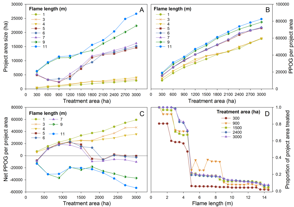
Fig. 6. Outputs from the optimization model under different combinations of flame length (FL) threshold and treatment area constraint. (A) Project area size; (B) ponderosa pine old growth (PPOG) per project; (C) net PPOG per project area calculated as the difference between the PPOG in treated stands minus the PPOG mortality in untreated stands, post wildfire; and (D) proportion of project area treated.
