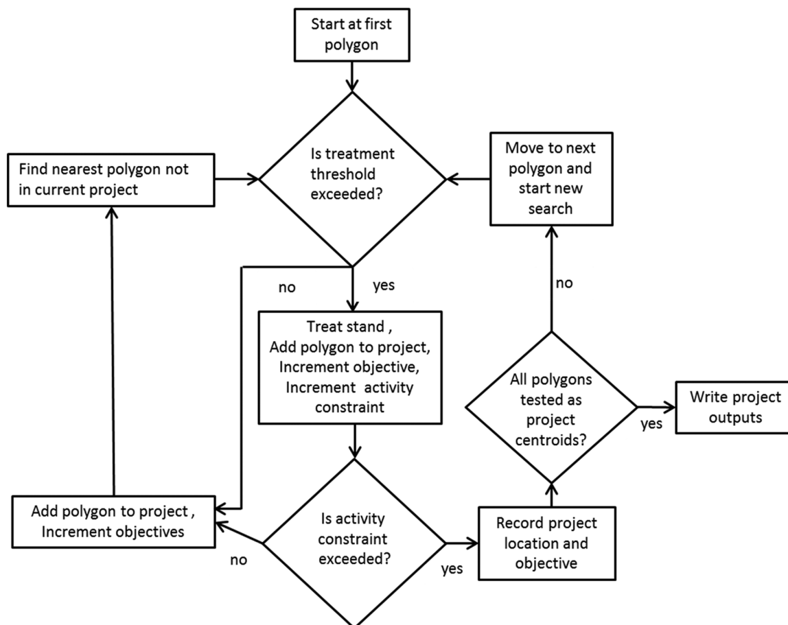
Fig. 3. Decision logic for the optimization model used to locate project areas. The algorithm tests each stand as the seed location for a project, and absorbs adjacent stands until a total area treated constraint is met. Stands that exceed a predetermined fire behavior threshold require treatment. The model identifies the aggregate of polygons that maximize the restoration objective and the polygons that require treatment. In the current study, polygons were defined as stands, treatment thresholds were measured by potential flame length, activity constraint was the total treatment allowance, and restoration objective was the total predicted post-wildfire, old growth ponderosa pine in the project area.
