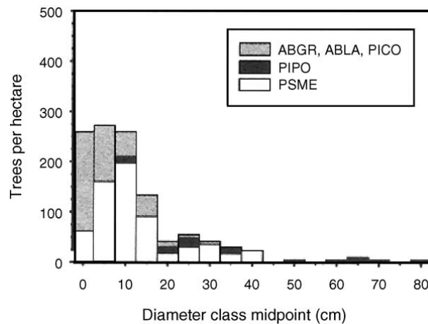
Fig. 4. Structure of a dry forest (from Scott and Reinhardt, 2001) indicating the predominance of very small, unmerchantable trees in the current structure (similar to bottom photo, Fig. 1). A low thinning of merchantable trees would begin at about 10 cm diameter, and crown or selection thinning would concentrate on even larger stems. Commercial harvest without treatment of the unmerchantable material will leave canopy base height unchanged and could increase surface fuel loads. ABGR = grand fir ( Abies grandis ), ABLA = subalpine fir ( Abies lasiocarpa ), PICO = lodgepole pine ( Pinus contorta ), PIPO = ponderosa pine ( Pinus ponderosa ), PSME = Douglas-fir ( Pseudotsuga menziesii ).
