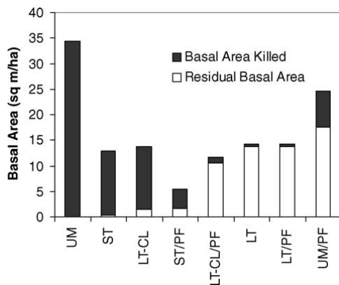
Fig. 6. Survival from a severe-fire-weather wildfire of the stand structures shown in Fig. 4. Columns are organized by absolute amount of residual basal area (white part of column). UM: unmanaged, ST: selection thin, LT: low thin, CL: commercial limit (>15 cm), PF: prescribed fire. The unharvested stand was assumed to be NFFL fuel model 10, harvested stands with no prescribed fire were assumed to be NFFL Model 11, and any stand treated with prescribed fire was assumed to be NFFL model 9. Fuel moistures for 1-, 10-, and 100-h fuels were 4, 5, and 6% for models 9 and 11 and 5, 6, and 7% for model 10. Open windspeed of 36 kph was adjusted to 0.4 for models 9 and 11 and 0.2 for model 10.
