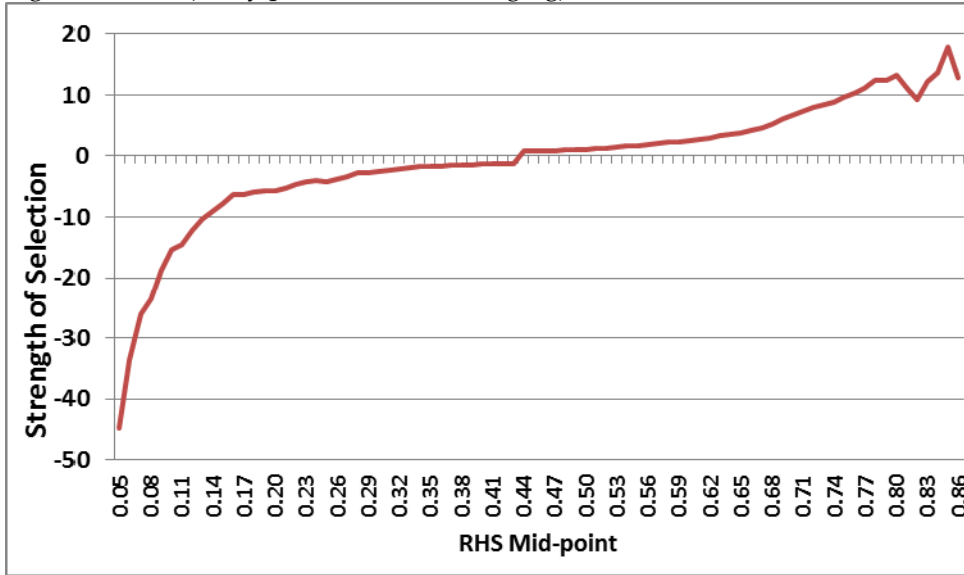
Figure C-4. This example of the strength of selection (SOS) evaluation shows a well-calibrated model. Areas with a mid-point RHS ( i.e. , relative habitat suitability value) of 0.05 (the moving window size here was 0.1) were used ~45-times less than would be expected based on its extent in the study area. Similarly, areas with a mid-point RHS of 0.8 (window of 0.75-0.85) were used ~12-times more than expected based on its extent in the study area. This figure was developed from a model trained on >3,000 spotted owl night locations (many presumed to be foraging).
