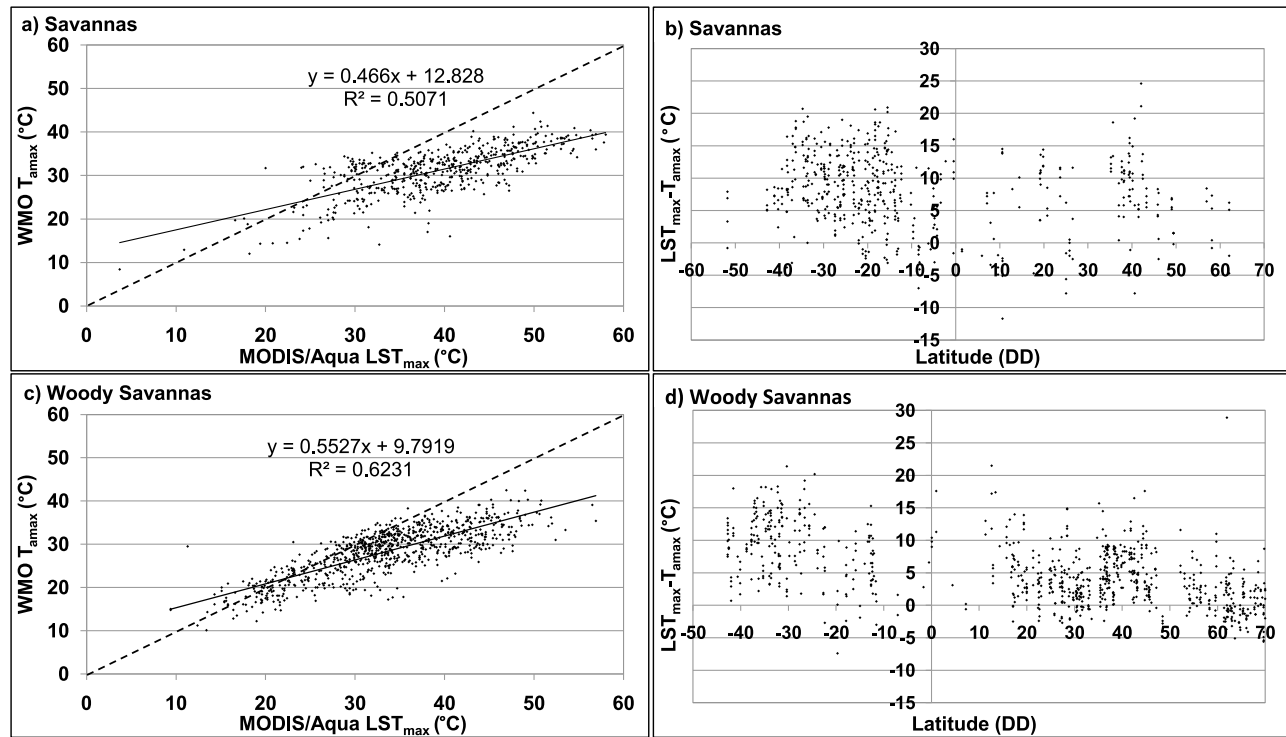
Figure 8. Observed LST_{\max}/T_{\max} relationship for (a, b) savannas and (c, d) woody savannas. Stomata are shut in savannas trees when extreme maximum temperatures occur, and the affect of increased surface roughness on the LST_{\max}/T_{\max} relationship in woody savannas can be observed. Woody savannas have a boreal and subarctic woodland component in the Northern Hemisphere where LST_{\max} and T_{\max} are tightly coupled (Figure 8d).
