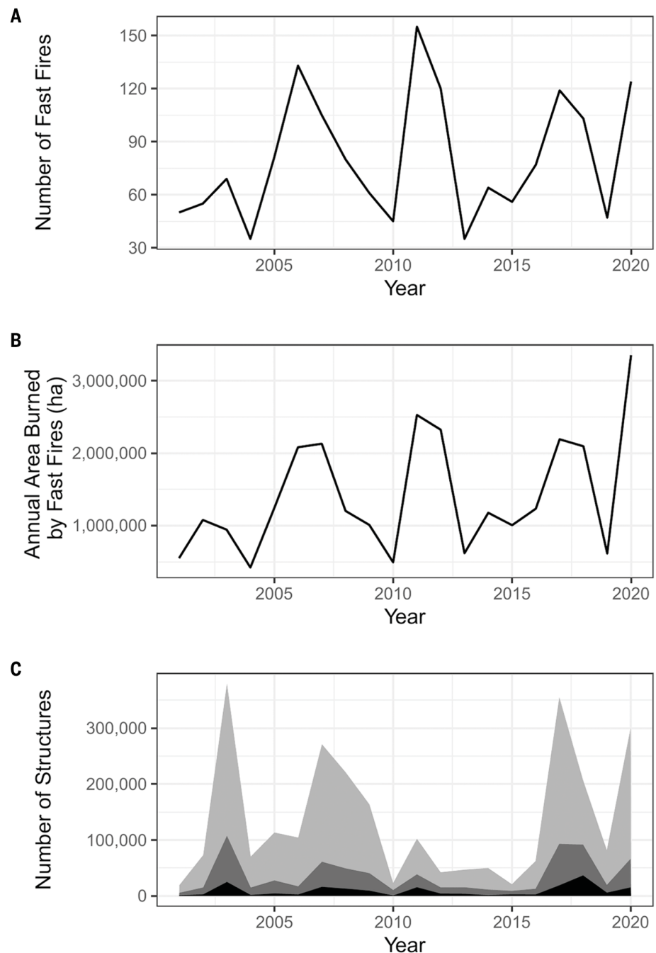
Fig. 4. Exposure to fast fires (>1620 ha/day) from 2001 to 2020. (A) Number of fast fires per year. (B) Annual area affected by fast fires. (C) Trends in the number of structures (based on the BUPR dataset) within the perimeters of fast fires (black), within 1 km of the perimeters of fast fires (dark gray), and within 4 km of the perimeters of fast fires (light gray).
