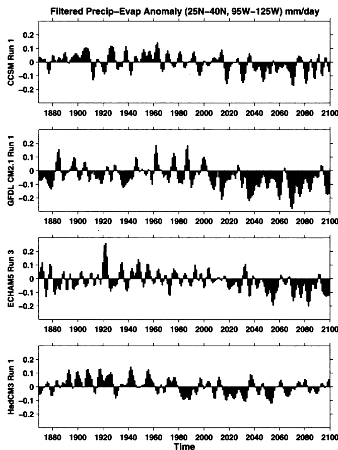
Fig. 3. The change in annual mean P - E over the American Southwest (125°W to 95°W and 25°N to 40°N, land areas only) for four coupled models, relative to model ensemble mean climatologies from 1950–2000. The results are from individual simulations of the 1860–2000 period, forced by known and estimated climate forcings and individual projections of future climate with the SResA1B scenarios of climate forcings. Because the modeled anomalies have not been averaged together here, these time series provide an idea of plausible evolutions of Southwest climate toward a more arid state. The models are the National Center for Atmospheric Research Community Climate System Model (CCSM), GFDL model CM2.1, Max Planck Institut Für Meteorologie model ECHAM5, and Hadley Centre for Climate Change model HadCM3. All time series are for annual mean data, and a 6-year low-pass Butterworth filter has been applied.
