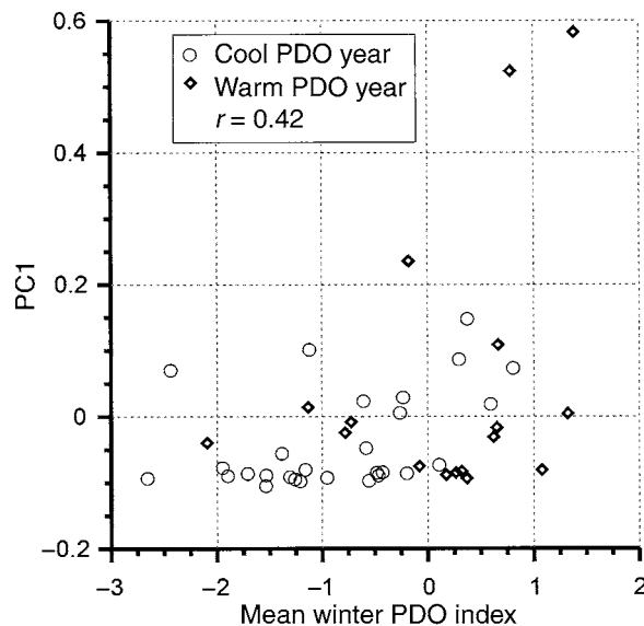
FIG. 17. Scatterplot of leading principal component of area burned (PC1) vs. mean winter (December, January, February) Pacific Decadal Oscillation (PDO) index. Warm PDO phase years (1978–1994) are indicated by diamonds, and cool phase years (1949–1976) are indicated by circles.
