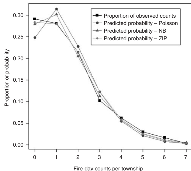
Fig. 3. Observed distribution of lightning fire-day counts per township ( \sim 10\,000 ha cell), compared with the predicted probability for each count category under a Poisson, Negative Binomial (NB) and Zero-Inflated Poisson (ZIP) regression model. Predicted probabilities were calculated using models P-BM t , NB-BMO t and ZIP-BM t respectively (Table 2).
