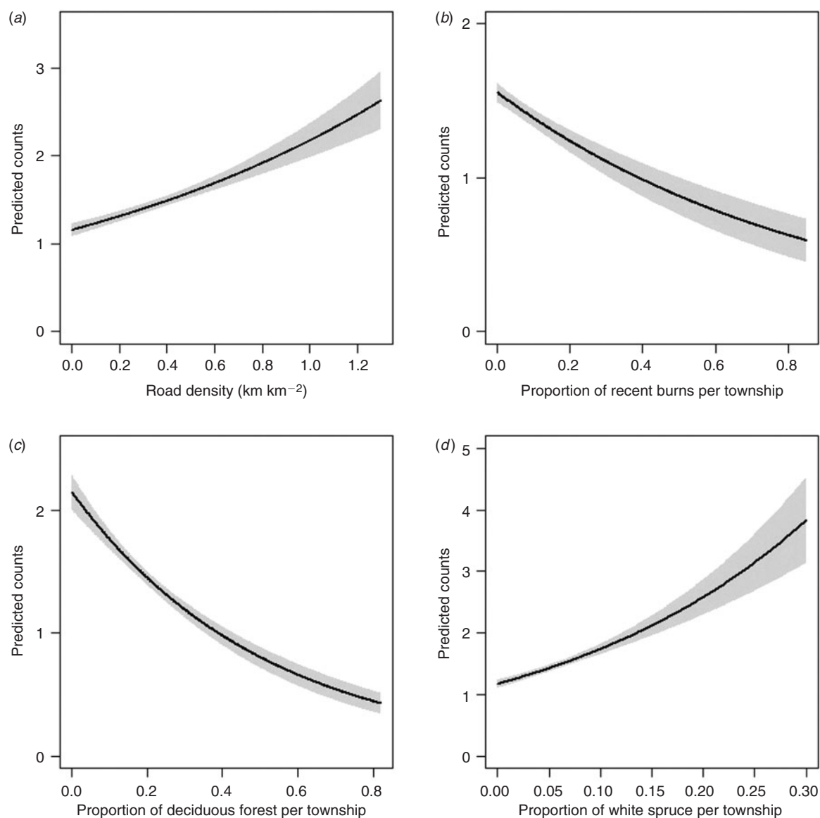
Fig. 4. Predicted lightning fire-day counts per township (black lines), together with 95% confidence interval (grey envelopes), as a function of (a) road density ( \text{km km}^{-2} of dry land); (b) proportion of recent burns; (c) proportion of deciduous-dominated forest; and (d) proportion of white spruce-dominated forest. Fitted frequencies were calculated using model NB-BMO t (Table 3), and the mean values for the remaining covariates in the model. Note: the scale of the y-axis differs between (a), (b), (c) and (d).
