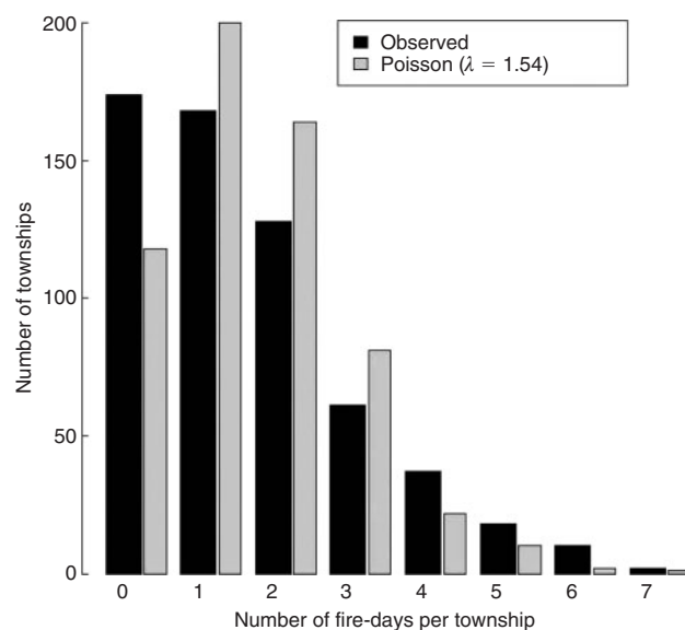
Fig. 2. Histogram of the number of lightning-caused fire days per township ( \sim 10\,000 ha). The grey bars show the expected number of fire days under a Poisson distribution with parameter \lambda = 1.54 . The sample consisted of 919 single fire day events that occurred within 598 townships between 1995 and 2002.
