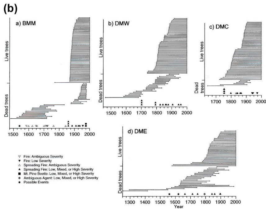
Figure 3. Two sources of evidence, early oblique photographs, and tree-ring reconstructions of age structure and fire scar dating of high-severity fires in dry forests in the Colorado Front Range: (a) high-severity fire identified by Jack [46] as in ponderosa pine and subsequent ponderosa pine (dark black) and quaking aspen regeneration in central Colorado in the Plum Creek Reserve; original photo, taken 18 August 1889, probably by John Jack, labeled “Looking north at Devils Head (Platte) Mt. from east side”. Original photo in the National Archives, FRA no. 008, (b) event diagram for four sample plots in which a tree-ring reconstruction of age structure of live and dead trees was completed in dry forests in Rocky Mountain National Park, Colorado. The severity of an event is indicated by the number of symbols stacked vertically: 1, low severity; 2, mixed severity; and 3, high severity. For example, in plot BMM, a high-severity fire was identified in the 1870s by a fire scar, extensive regeneration after the fire, and dead trees before the fire. Each line shows the lifespan of one tree. Reprinted from ([14] Figure 2) with permission from John Wiley and Sons.
