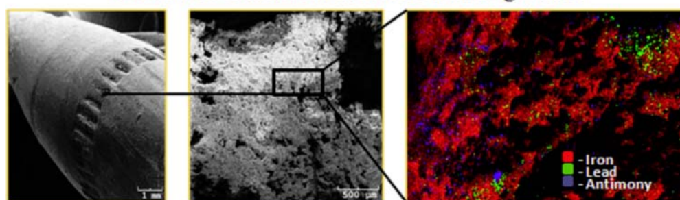
Figure 2. Chemical characterization of a 5.56mm corroding bullet that underwent 15 years of weathering in Alaskan soils using scanning electron microscopy (SEM) and energy dispersive x-ray analysis (EDX). Relative concentrations for iron (red), lead (green), and antimony (purple) are shown in the right x-ray map. Data was collected at the Advanced Instrumentation Laboratory (AIL), University of Alaska Fairbanks (UAF). Data collected by A.J. Barker
