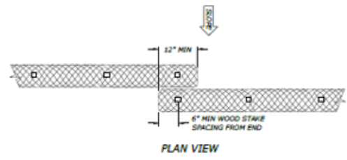
5 STRAW WATTLE NTS
