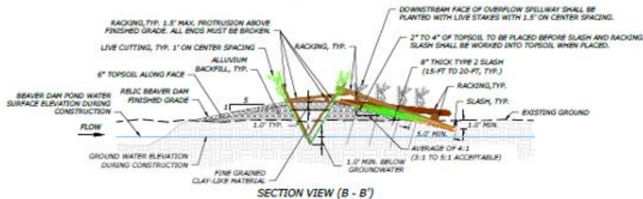
1 RELIC BEAVER DAM ANALOGUE
