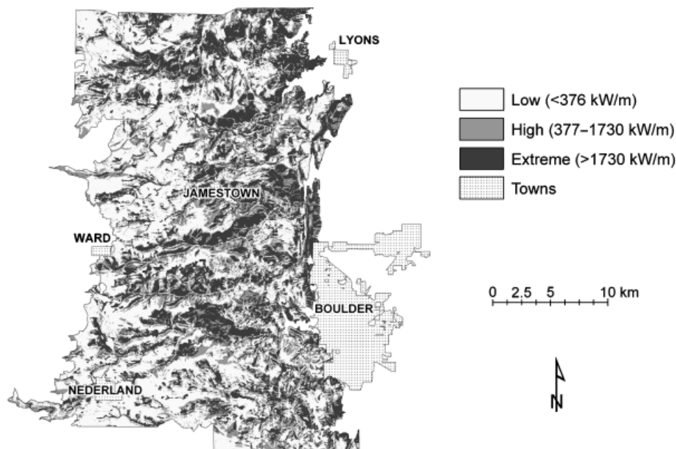
Figure 2. Potential fireline intensity in the montane zone of Boulder County under 24-kph upslope winds, classified from FlamMap output.
