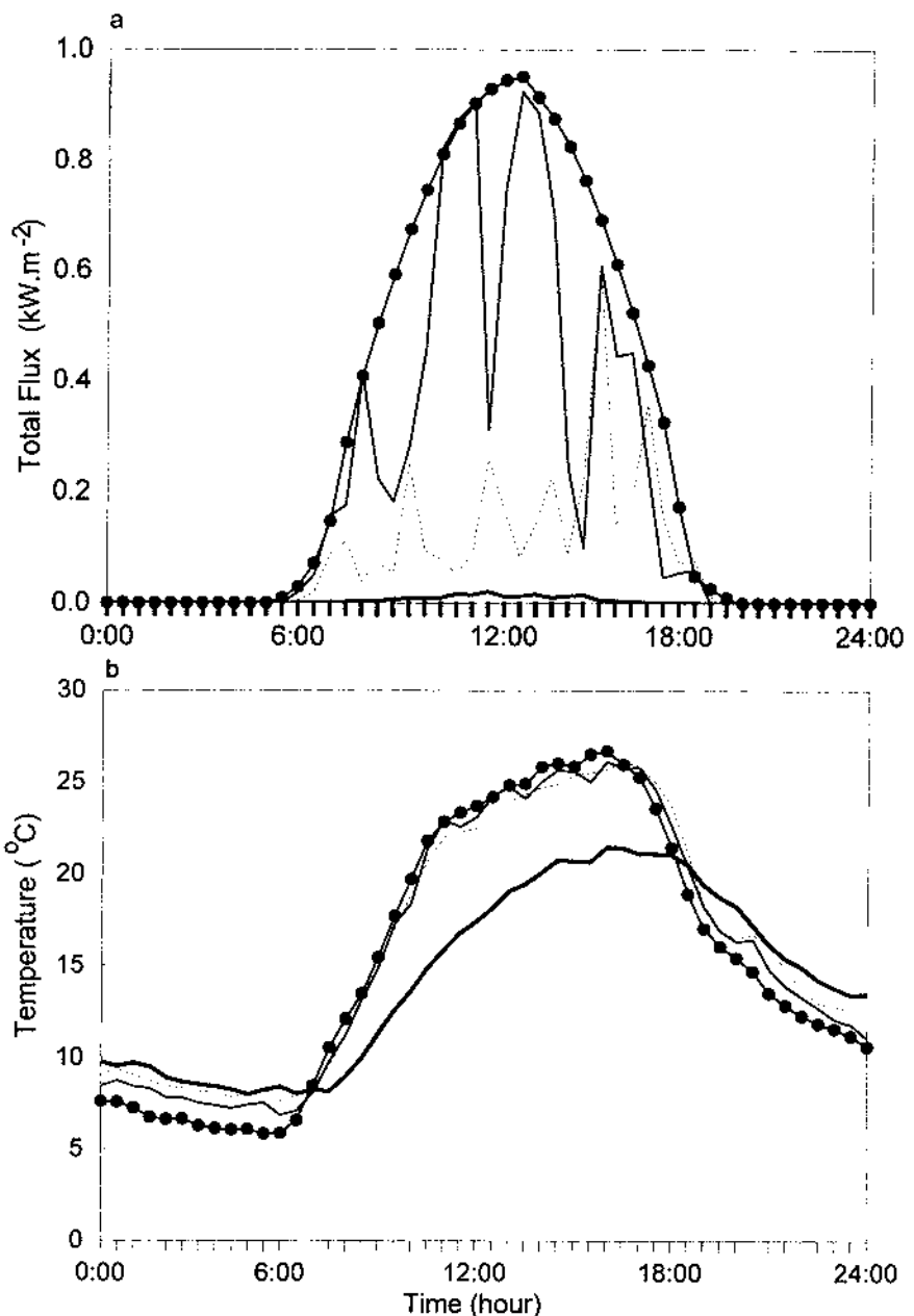
Figure 4. Diurnal changes in microclimate under different harvest regimes. (a) Patterns of shortwave radiation ( \text{kW}/\text{m}^2 ) for a 70-year-old Douglas-fir ( Pseudotsuga menziesii ) forest (thick black line) and three sites recently harvested using clearcut (solid line with circles), dispersed green-tree retention (partial cut; solid line), and aggregated green-tree retention (patch; dashed line) techniques. (b) Patterns of air temperature ( ^{\circ}\text{C} ) at 2 m above the ground for the same sites. Data were collected in western Washington on 25 August 1992 (the study sites are shown in Figure 2).
