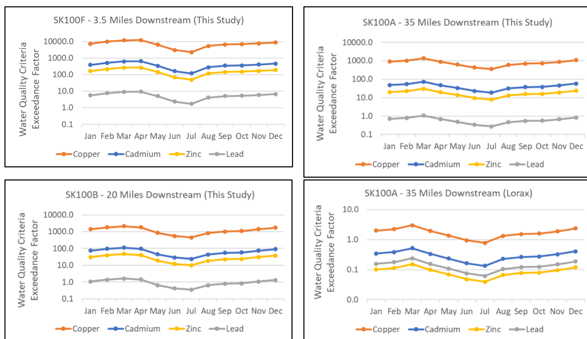
Figure 8. Results for water quality criteria exceedance factors at gaging stations in the South Fork Kokoiti River for this study and for the Lorax Environmental [23] study. Note the log scale on the y-axis. At an exceedance factor of 1.0, the predicted stream concentration equals the water quality criterion.
