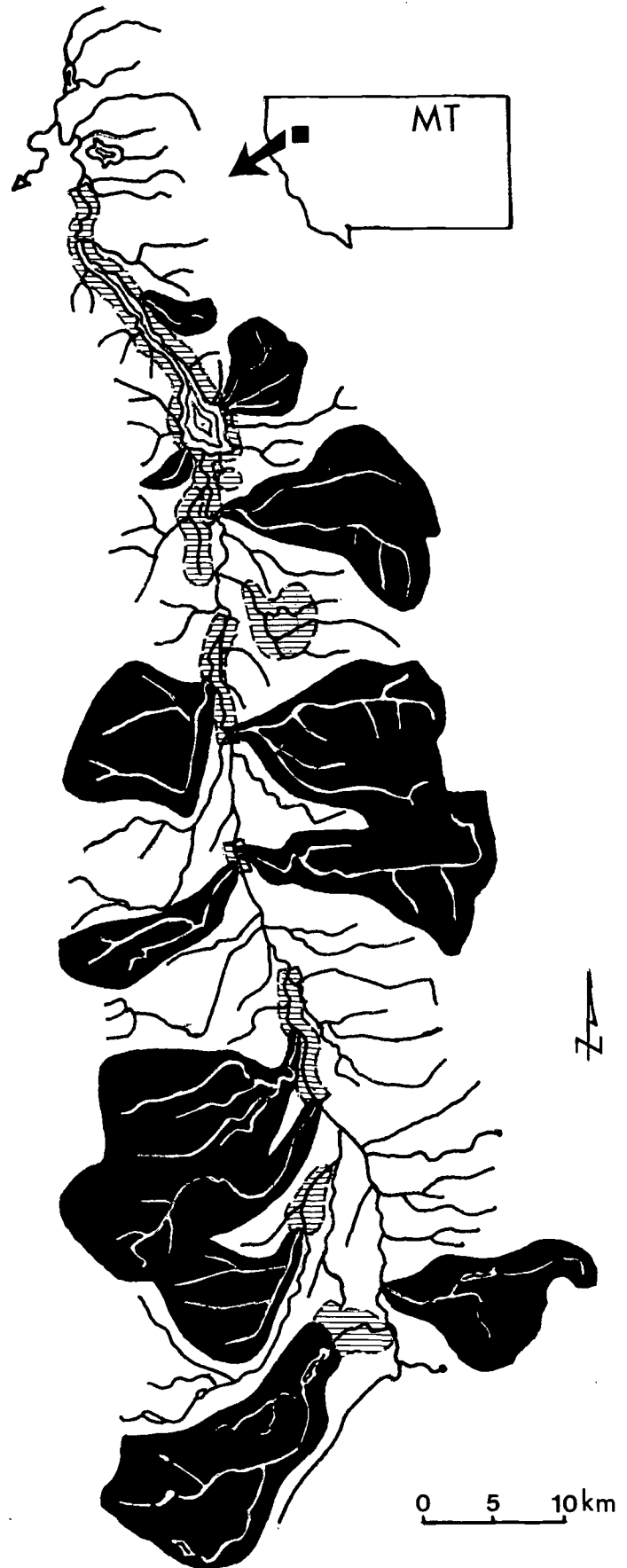
Figure 2. Example of a Recommended Design for an Aquatic Diversity Reserve Network for the Swan River Basin, an Area of 2,070 km 2 in Northwest Montana, USA (after Frissell et al. , 1995). The figure shows critical watersheds (black tone) and river-lake corridors and wetland complexes (line shaded). Critical watersheds contain relatively well-distributed populations of native fishes, restricted distribution of non-native fishes, and limited fish stocking history. Watersheds selected by biological criteria turned out to be among those least-impacted by land use activities in the basin.
