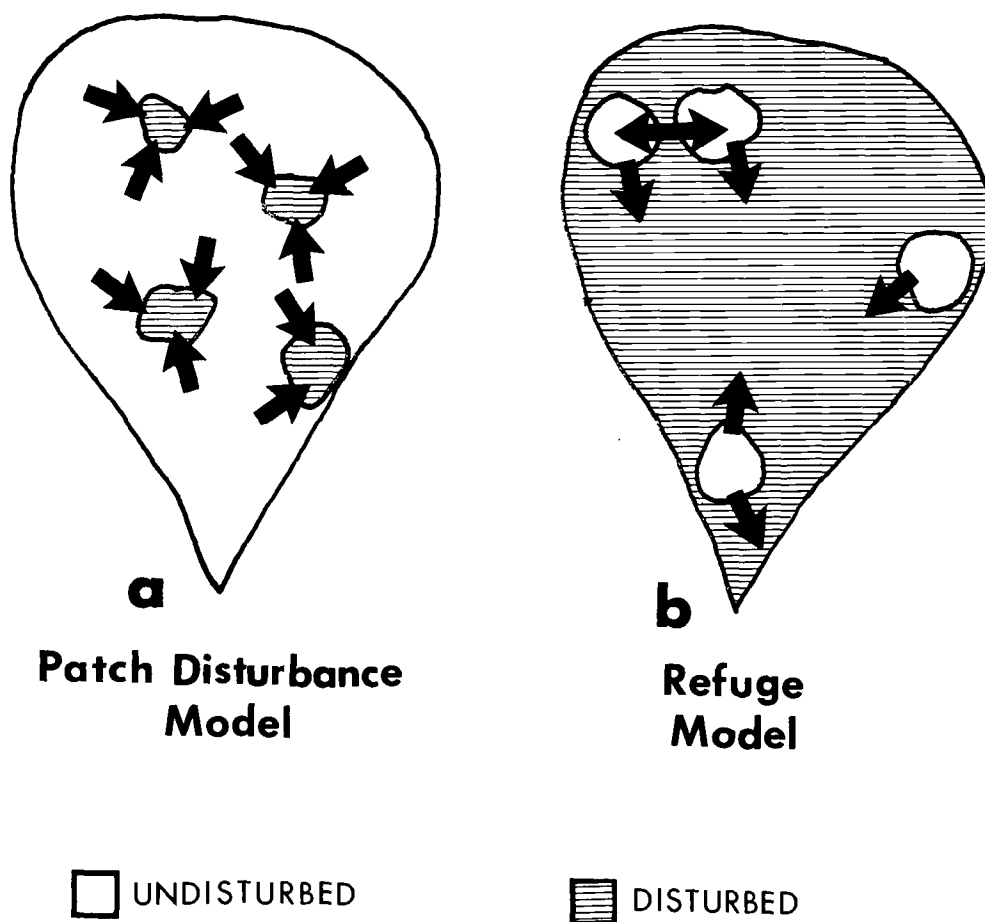
Figure 1. The Changing Biogeographic Context of Aquatic Ecosystem Management. In catchment a, degraded aquatic habitats (shaded) constitute isolated patches within a matrix of high-quality, richly-inhabited areas. Abundant, well-connected populations supply a steady supply of colonists (arrows represent colonization vectors) to re-establish populations in disturbed areas. In catchment b, high-quality habitats are isolated remnants in a matrix of disturbed and degraded habitat. Fragmented habitat islands serve as refugia for sensitive species and provide weak and localized or unidirectional sources of colonists to the degraded and relatively hostile matrix. Many refugia are sufficiently distant from others that little successful exchange of individuals between populations occurs, but some migration still occurs between patches that are closely spaced.
