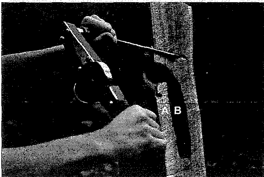
This photo shows the longitudinal section of an American three-toed woodpecker ( Picoides dorsalis ) nest and the procedure the study used to quantify wood hardness. First, the researchers use a drill to create a small hole about one-third inch in diameter above the nest cavity opening (top). Then they record the torque required to spin an increment borer into the predrilled hole (bottom). The area marked "A" represents the nest sill, and the area marked "B" represents the nest cavity body.
