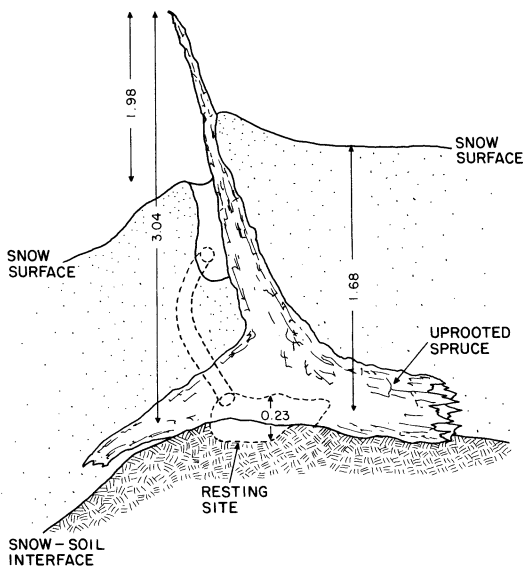
Fig. 1. Side view of resting site used by marten during winter 1985–86 (excavated 31 Jan 1986) in relation to uprooted spruce and snow layer. Partially decomposed wood formed the roof of the resting chamber. Dimensions are in meters.
