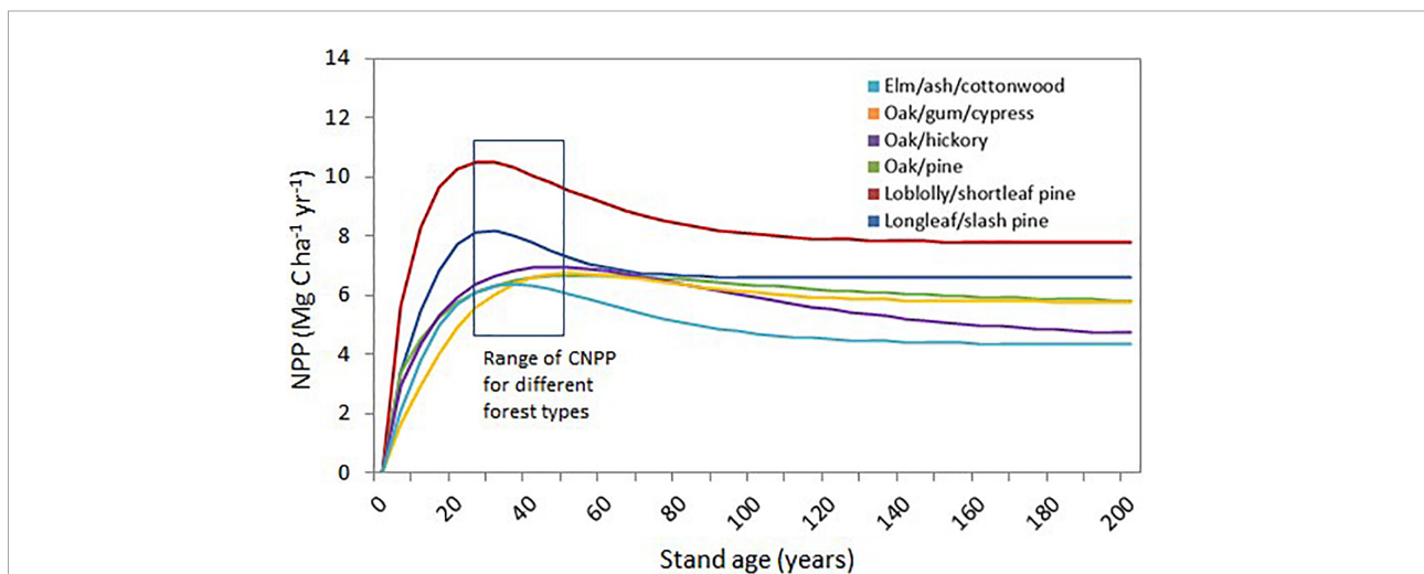
FIGURE 2 Net primary productivity (NPP) for selected forest types in the South (He et al., 2012). Culmination of NPP (CNPP) occurs at the stand age having the greatest annual increment rate, typically at or just after the tree canopy closes. Younger stands are those with ages less than CNPP. Older stands have ages greater than CNPP. CNPP is highly variable among forest types and geographic regions—in this example, from ages 23 to 45. The He et al. (2012) paper includes detailed uncertainty analyses of these and other NPP curves.
