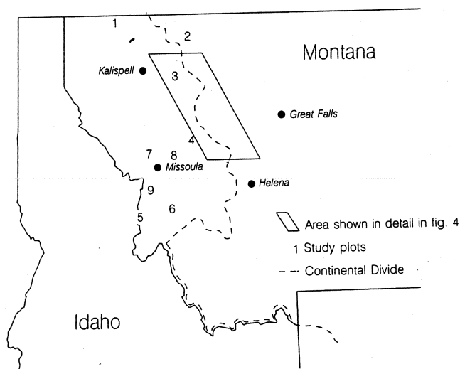
Figure 2. Location of study areas. 1—Mt. Marston, 2—Divide Mt., 3—25 Mile Creek, 4—Morrell Mt., 5—Twin Lake, 6—Skalkaho Pass, 7—Point Six, 8—Mineral Peak, 9—St. Mary's Peak.
