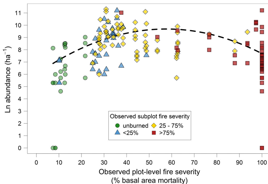
Fig. 2. Correlation of the natural logarithm of total tree regeneration abundance with observed basal area mortality at the 1-ha plot-scale. The dashed line represents the statistical relationship from our top model quantifying regeneration abundance at the nested 0.10-ha regeneration plot-scale in relation to observed basal area mortality at the 1-ha plot-scale. Points are observations of regeneration abundance at each of the four nested regeneration plots, and their color and shape schema represent the observed basal area mortality at the 0.10-ha scale. The x-axis represents basal area mortality at the 1-ha plot-scale. Most a priori low-severity plots transitioned to moderate-severity, most likely a result of delayed mortality, by the time we sampled these forests a decade or two after the fire.
