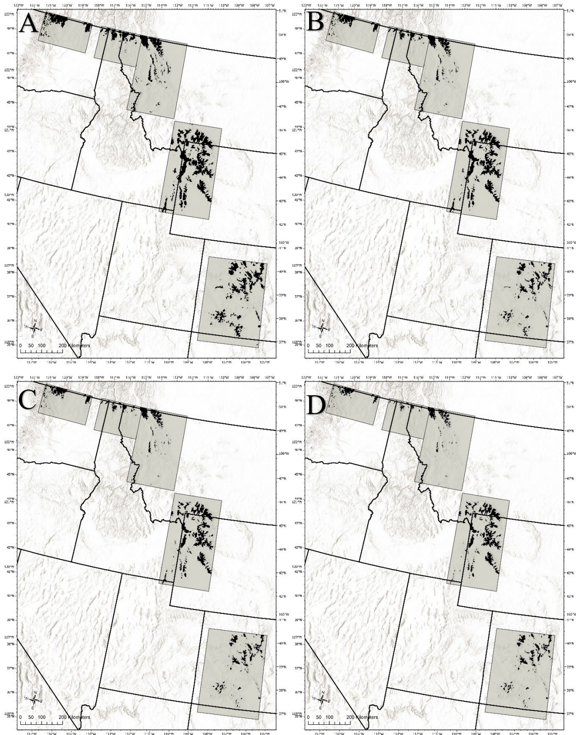
Figure 8. Snow model projections \geq 1m on May 1 (lower quartile for future projections) using SSP 5-8.5 projection. A. Historical (1995–2014); B. (2036–2055); C. (2056–2075); and D. (2076–2095).
