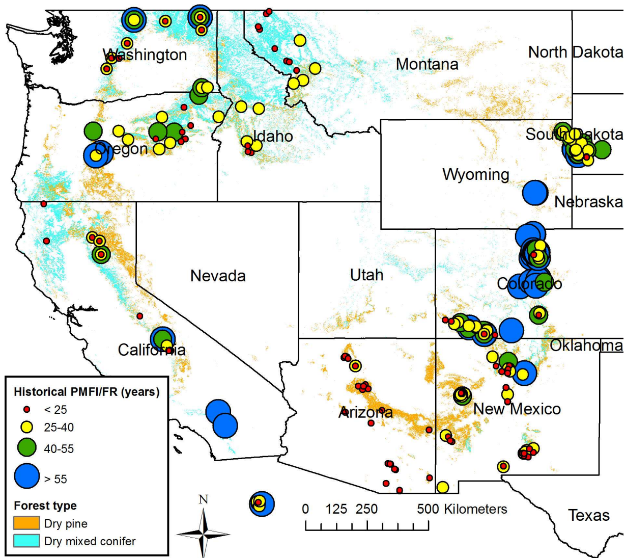
Fig 3. Estimated historical low-severity population mean fire interval/fire rotation (PMFI/FR) for the combined set ( n = 342 ) of calibration cases and prediction sites in dry forests of the western USA.
