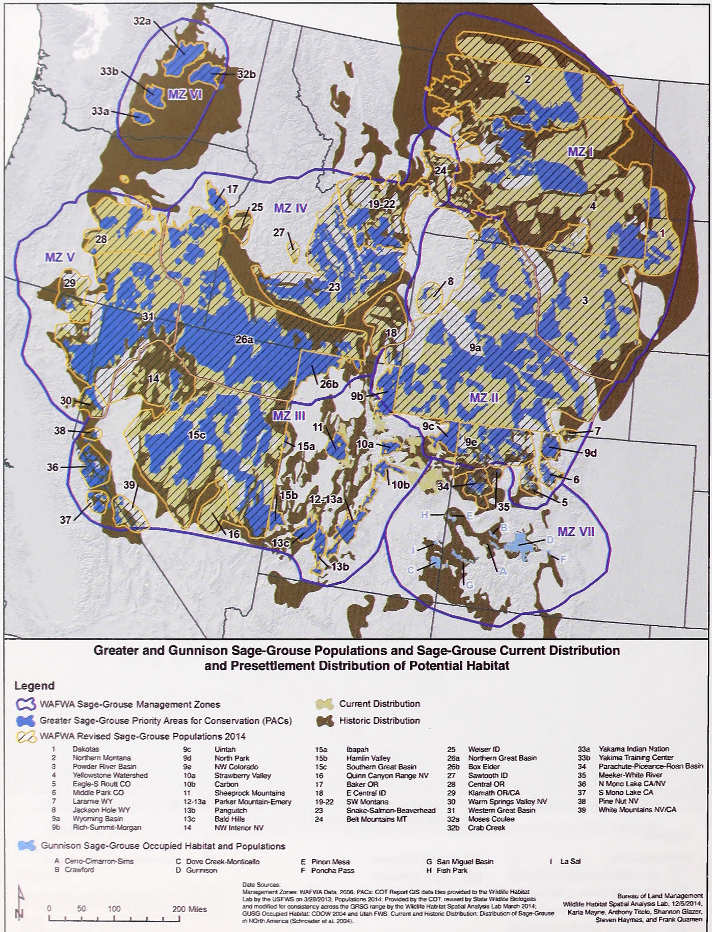
Figure 3. Priority areas for conservation (PACs) as identified by the Conservation Objectives Team (COT) and Gunnison Sage-Grouse occupied habitats. PACs are encircled by seven sage-grouse management zones established by the Western Association of Fish and Wildlife Agencies (WAFWA) based on populations within floristic provinces (Stiver et al. 2006).
