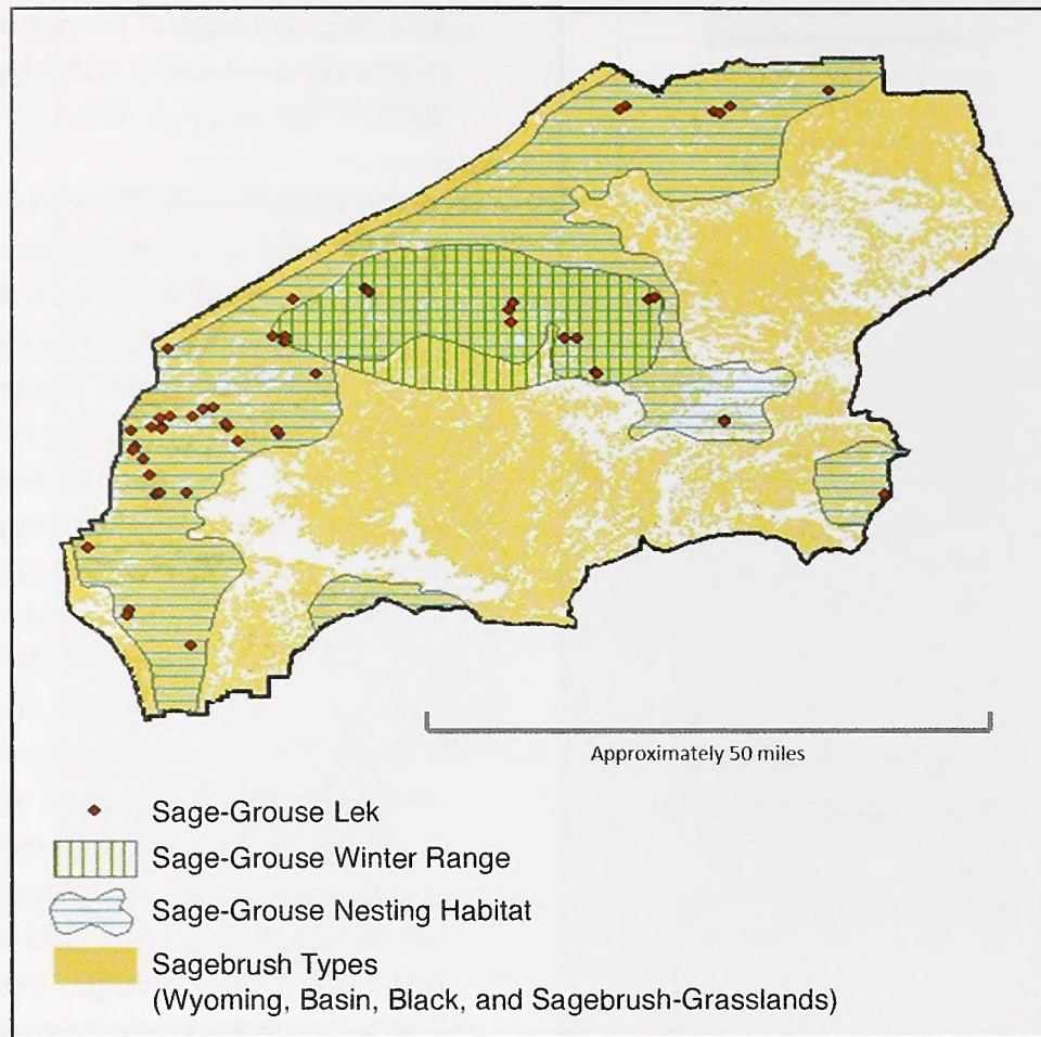
Figure 10. Fine-scale (third-order) habitat selection.
