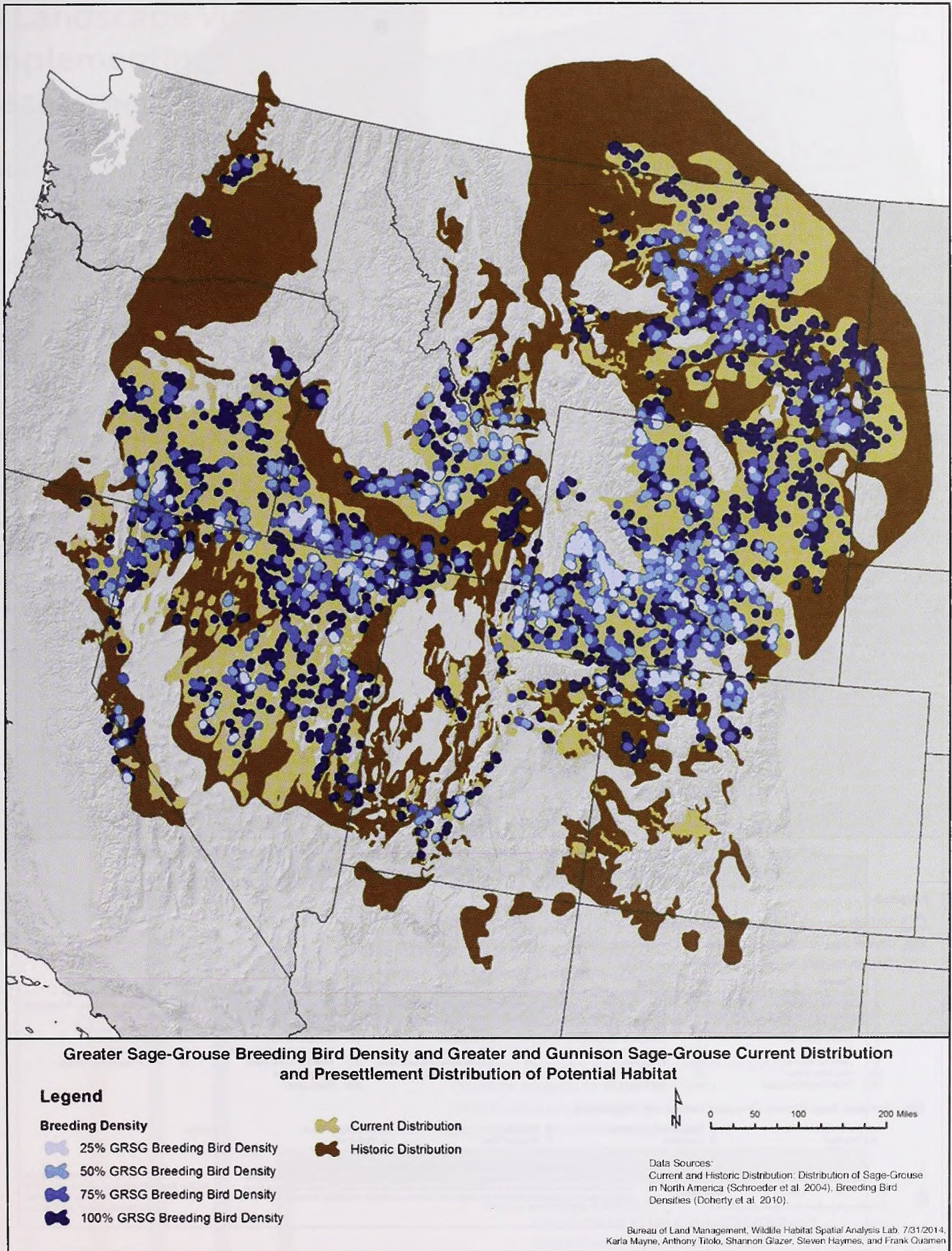
Figure 2. Greater Sage-Grouse (GRSG) population centers or “core areas” across the species’ range. The lightest blue areas contain 25 percent of the breeding population, and each darker shade of blue indicates an additional 25 percent. Gunnison Sage-Grouse breeding bird density is not displayed.
