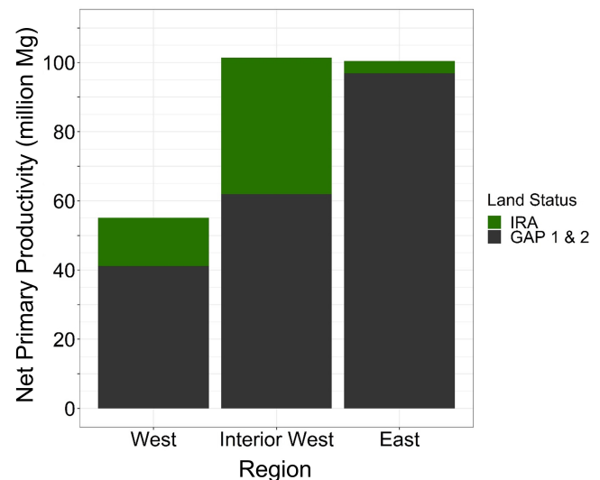
FIGURE 5 Total carbon captured (estimated using net primary productivity) in protected areas (GAP 1 and 2 lands) as well as within Inventoried Roadless Areas in three regions of the contiguous US. Only Gap 1 and 2 lands and IRAs larger than 1 km 2 were included in this analysis
