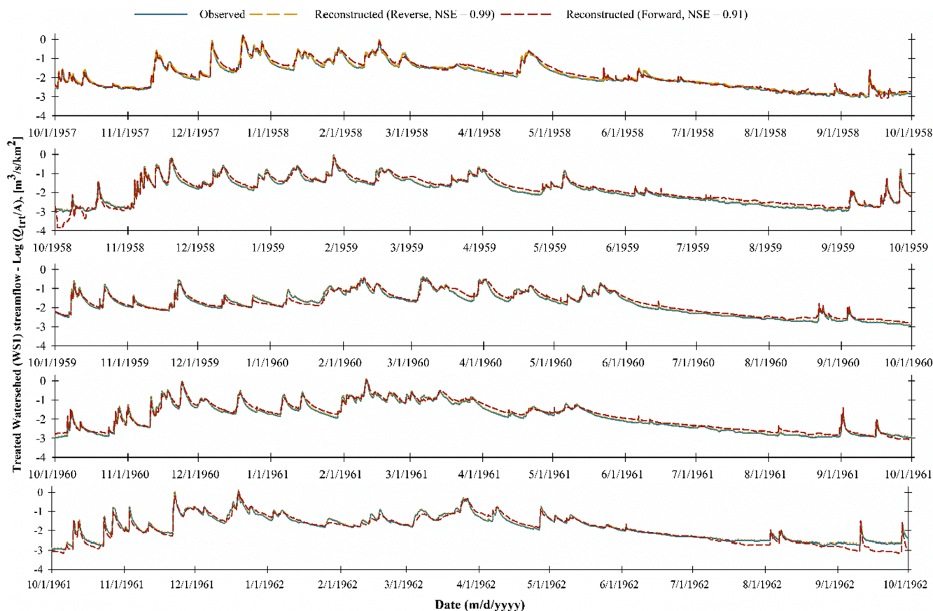
Fig. 9. Validation of streamflow reconstruction technique using forward and reverse regression.
