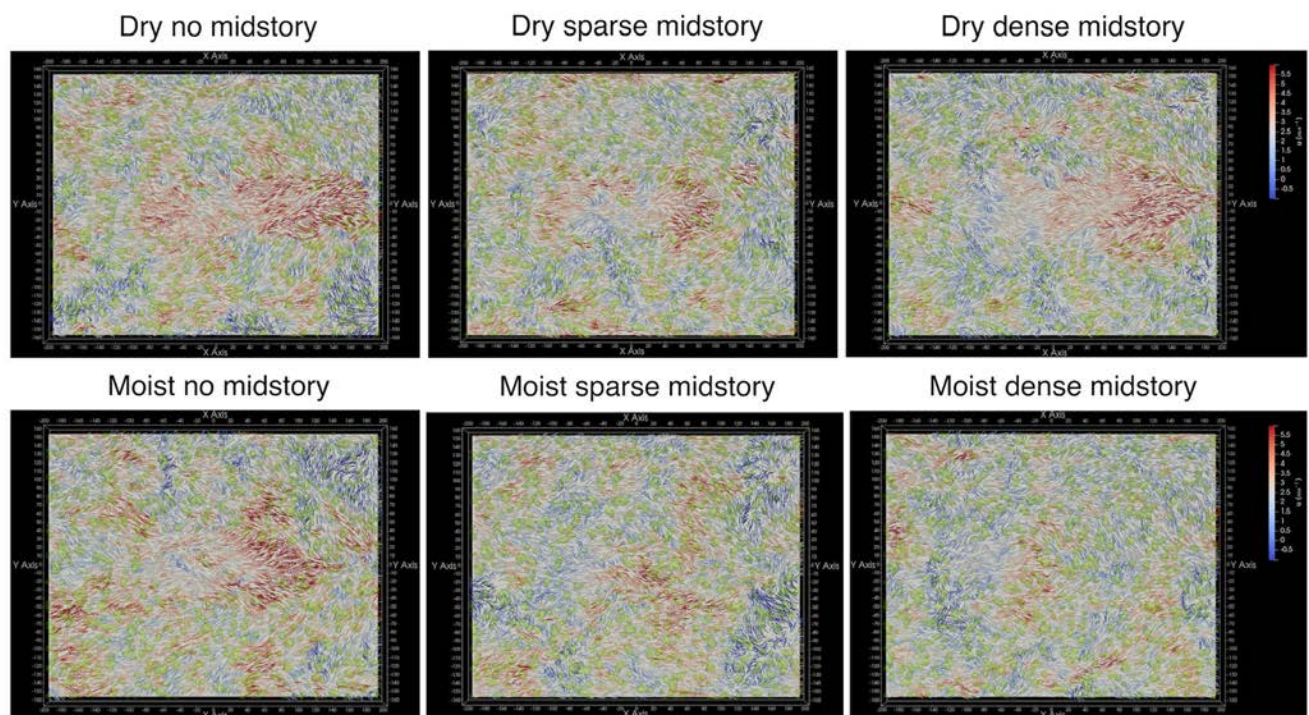
Figure 2. Sub canopy wind field ( u-v plane at 7 m height) with arrows colored by instantaneous streamwise velocity component ( u ) after 520 s for the six scenarios.
