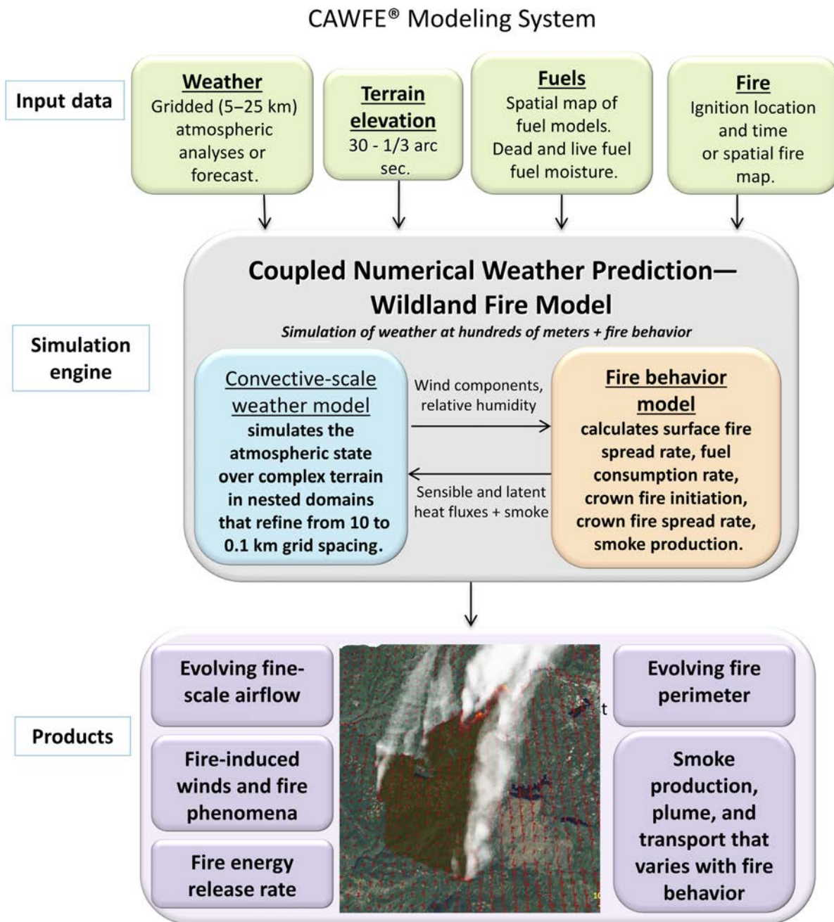
FIG. 2. Overview of the CAWFE modeling system.
