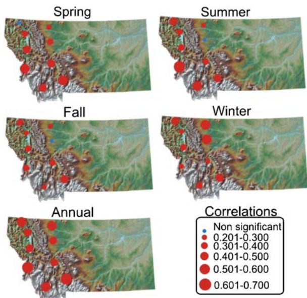
Fig. 8 Correlations between average annual and seasonal temperature records for the Northern Hemisphere and the nine individual Montana stations. Correlations are calculated between the unsmoothed time series and significant values are based on p -value \leq 0.05
