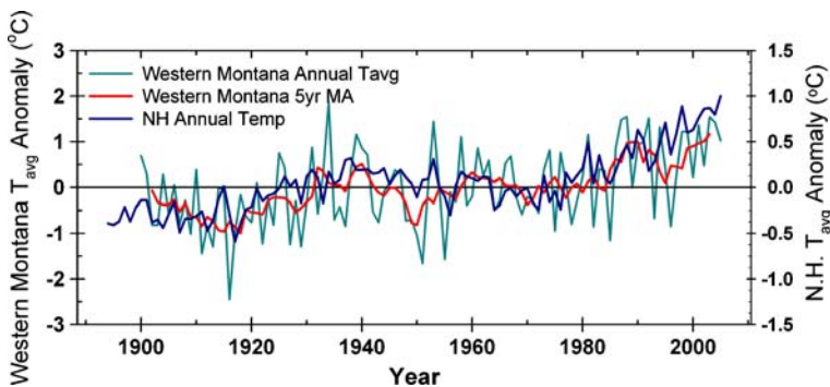
Fig. 6 Comparison of variability and trends in western Montana (blue-green) and Northern Hemisphere (dark blue line) annual average temperatures. A 5-year moving average (red line) highlights the similarity in trends and decadal variability between records
