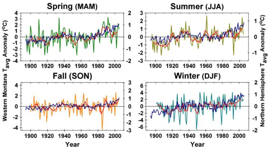
Fig. 7 Comparison between trends in western Montana and Northern Hemisphere (blue line) seasonal temperatures. Red line displays the western Montana 5-year running mean. Note change in scale of temperature axis for each season, this has implications related to absolute temperature change
