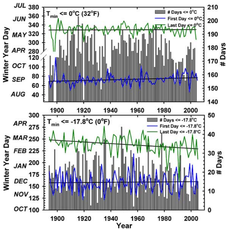
Fig. 5 Average number of frost/freeze days ( \#days^{-yr} T_{min} \leq 0.0^{\circ}\text{C} ( 32.0^{\circ}\text{F} )) or extremely cold days ( \#days^{-yr} T_{min} \leq -17.8^{\circ}\text{C} ( 0.0^{\circ}\text{F} )) per winter year in Western Montana (gray bars). Graphs also depict the first day of fall (blue line) and last day of spring (green line) temperature equaled or exceeded the defined threshold
