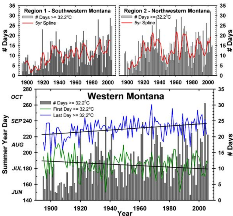
Fig. 4 Top: Graphs showing the different rates of change in number of days -yr T_{\max} \geq 32.2^{\circ}\text{C} (gray bars) for southwestern (left) and northwestern Montana (right) from 1895–2006. A 5-year moving average (red line) highlights trends and variability in #days -yr \geq 32.2^{\circ}\text{C} . Bottom: Trends in number of days (gray bars), and the first (green line) and last (blue line) day of every summer, that temperature in western Montana equaled or exceeded 32.2^{\circ}\text{C}
