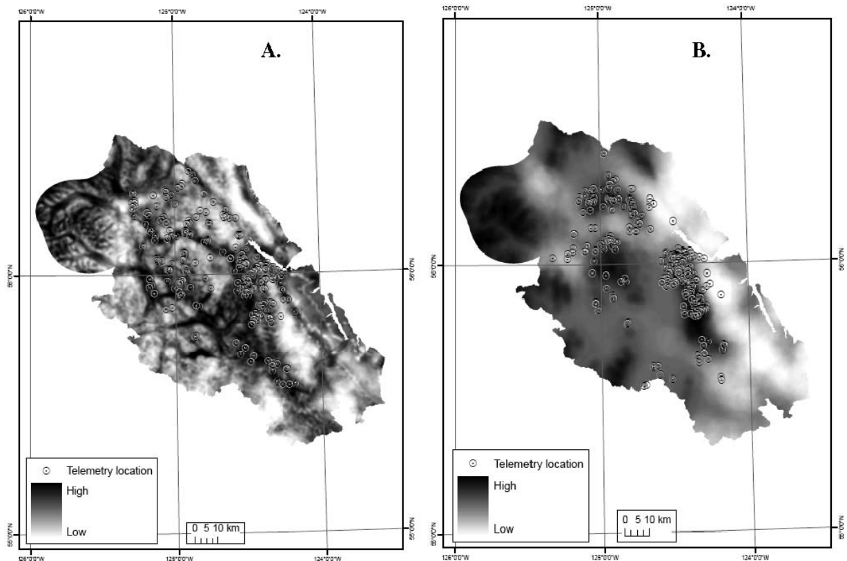
Figure 7. Multivariate logistic regression models depicting female wolverine habitat quality within the Omineca Mountains study area, near Mackenzie, British Columbia, Canada in A) winter and B) summer. Telemetry points were gathered from radiomarked adult females from the study area, 1995–2002. Darker area represents higher probability of habitat selection.
