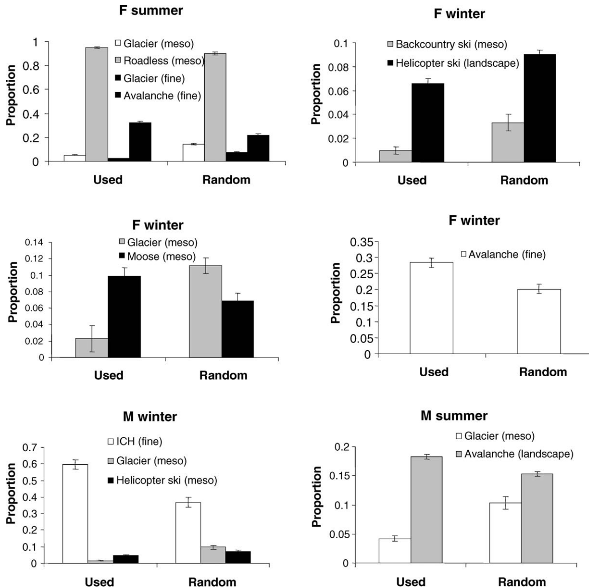
Figure 4. Univariate means and standard errors for selected predictor variables from most supported female and male wolverine seasonal habitat use models for the Columbia Mountains, British Columbia, Canada, 1995–2003. Habitat composition (proportion) was measured in a scale-dependent manner (fine, meso, landscape) around each telemetry location (used) and paired random (random) point.
