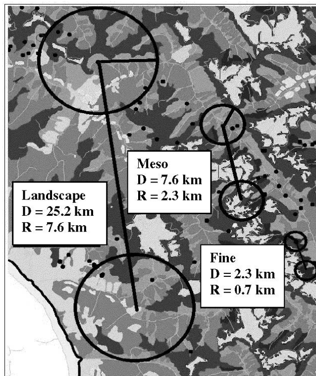
Figure 3. Multiscale (landscape, meso, fine) design used to analyze wolverine habitat selection using Columbia Mountain, British Columbia, Canada, males as an example. "D" refers to distance between used and random points; "R" is the radius within which habitat composition is measured. Baseline Thematic Mapper habitat layer (Surveys and Resource Mapping Branch 1995) is shown. Approximate scale, 1:350,000.
