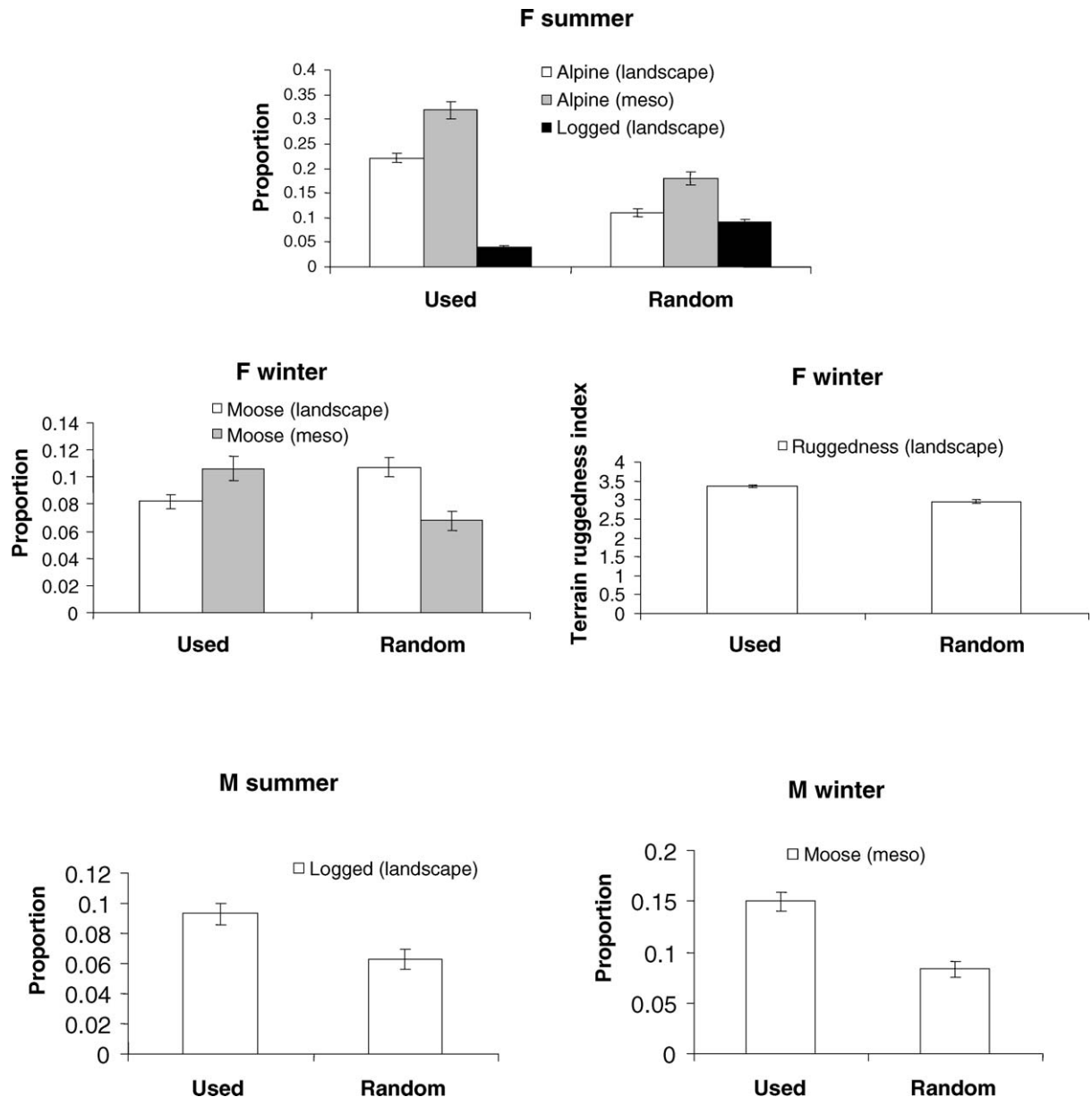
Figure 5. Univariate means and standard errors for predictor variables from most supported female and male wolverine seasonal habitat use models for the Omineca Mountains, British Columbia, Canada, 1995–2003. Habitat composition (proportion) was measured in a scale-dependent manner (fine, meso, landscape) around each telemetry location (Used) and paired random (Random) point.
