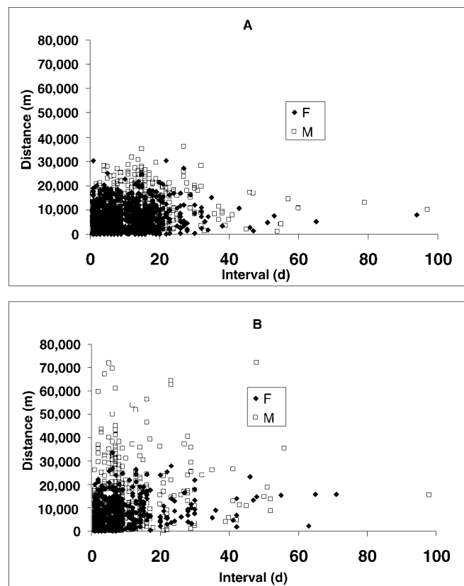
Figure 2. Distance (m) and interval (d) between sequential radiotelemetry locations for male and female wolverines monitored in (A) Columbia Mountains, British Columbia, Canada, 1995–2003, and (B) Omineca Mountains, 1995–2002.
