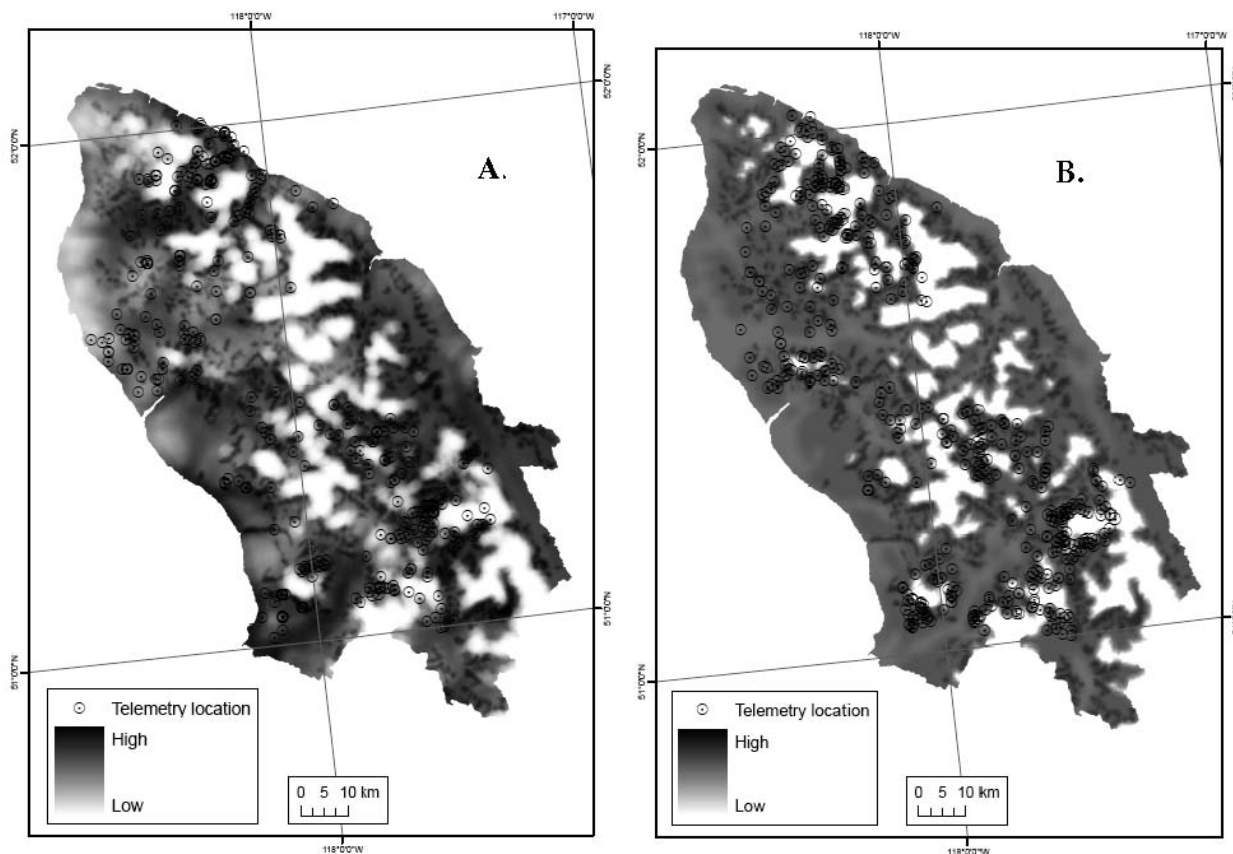
Figure 6. Multivariate logistic regression (resource selection function) models depicting female wolverine habitat quality within the Columbia Mountains study area, near Revelstoke, British Columbia, Canada in A) winter and B) summer. Telemetry points were gathered from radiomarked adult females from the study area, 1995–2003. Darker area represents higher probability of habitat selection.
