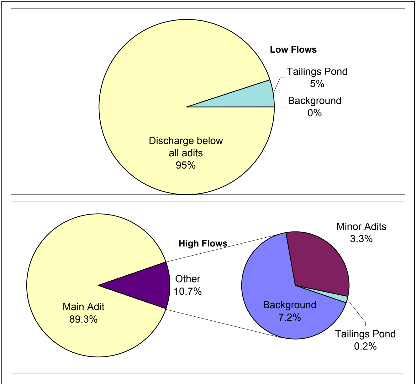
Figure 4.4 Percent Contribution of Source Areas to Zinc Loading at Standard Mine for low flow (upper) and high flow (lower) data sets
