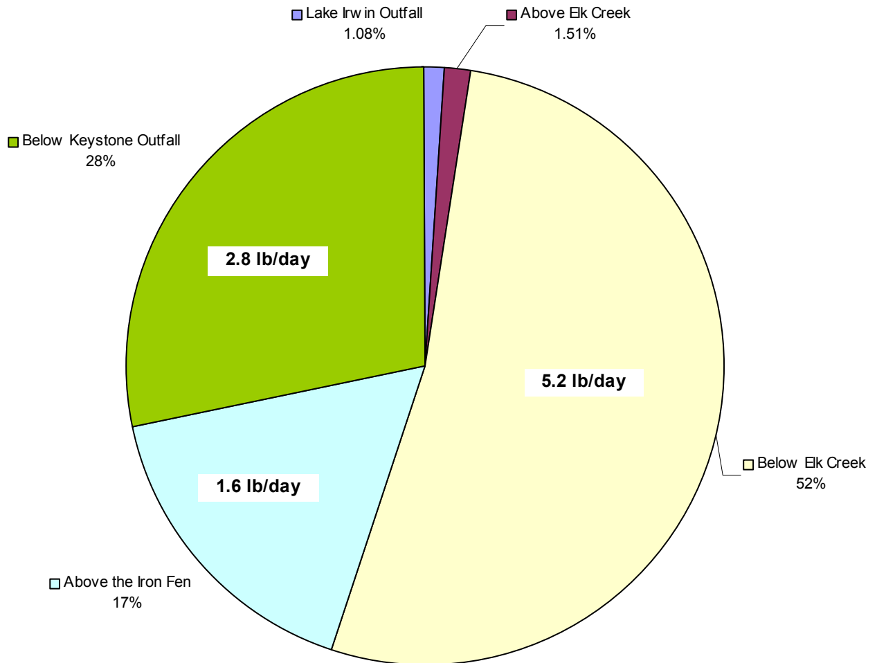
Figure 4.3 Percent Contribution from Pollutant Source Areas to main stem of Coal Creek in June 1999 (URSOS, 1999)
