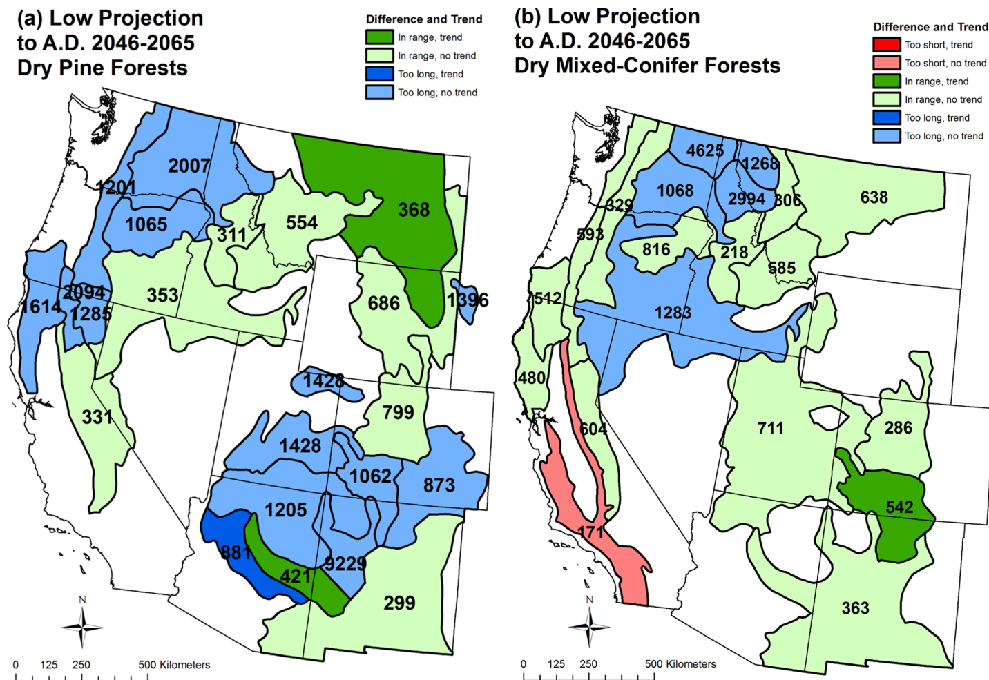
Fig 5. Low projection (to A.D. 2046–2065) of differences relative to the historical range of high-severity fire rotations, given 1984–2012 trends, and projected fire rotations for high-severity fire in (a) dry pine forests and (b) dry mixed-conifer forests by analysis region. See Fig 3 for an explanation of figure contents.
