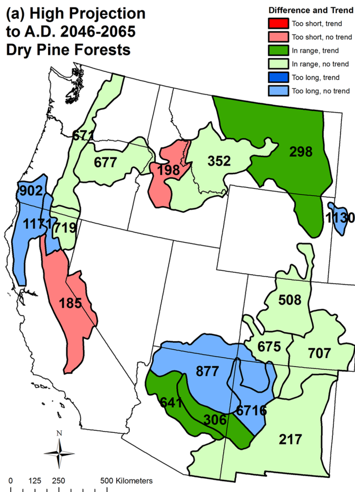
Fig 6. High projection (to A.D. 2046–2065) of differences relative to the historical range of high-severity fire rotations, given 1984–2012 trends, and projected fire rotations for high-severity fire in (a) dry pine forests and (b) dry mixed-conifer forests by analysis region. Several analysis regions are omitted, because the high projections by Yue et al. [42] were not possible for those areas. See Fig 3 for an explanation of figure contents.
