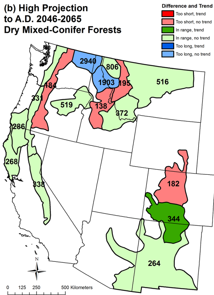
Fig 6. High projection (to A.D. 2046–2065) of differences relative to the historical range of high-severity fire rotations, given 1984–2012 trends, and projected fire rotations for high-severity fire in (a) dry pine forests and (b) dry mixed-conifer forests by analysis region. Several analysis regions are omitted, because the high projections by Yue et al. [42] were not possible for those areas. See Fig 3 for an explanation of figure contents.
