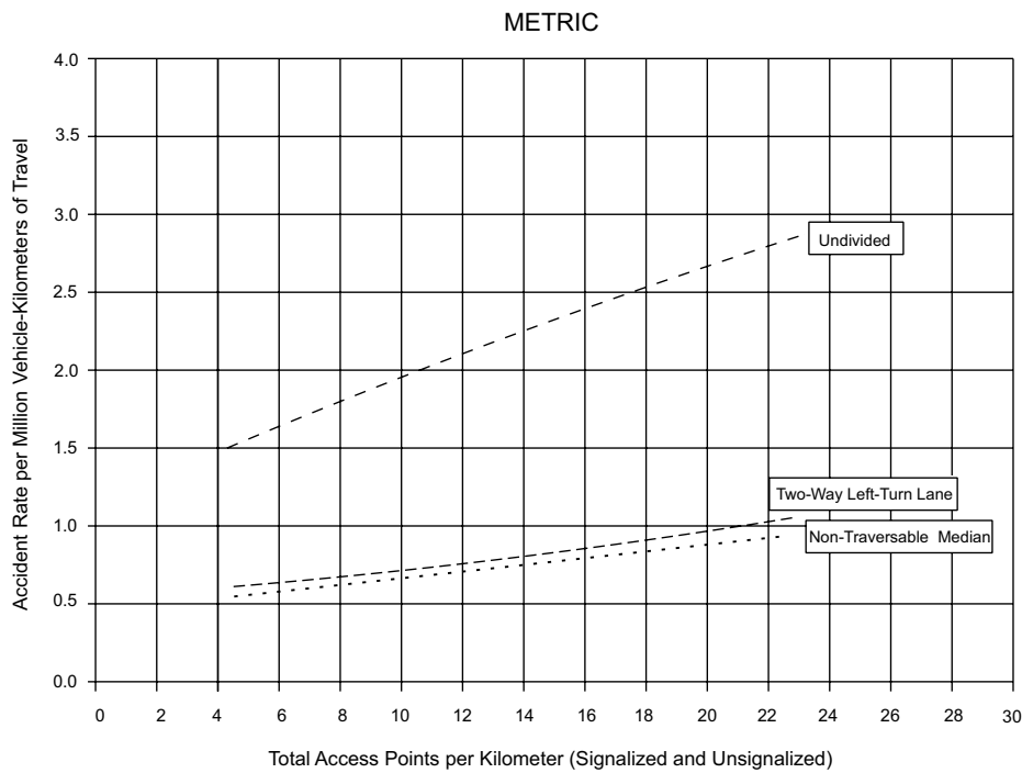
Figure 2-8. Estimated Crash Rates by Type of Median—Rural Areas (25)
