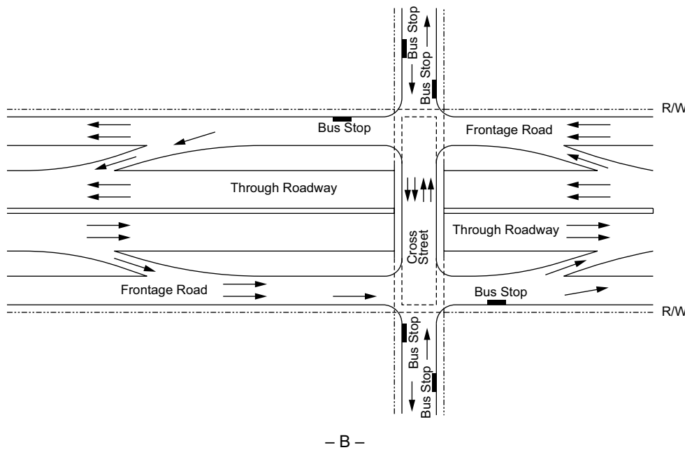
Figure 8-26. Bus Stops at Street Level on Diamond Interchange
