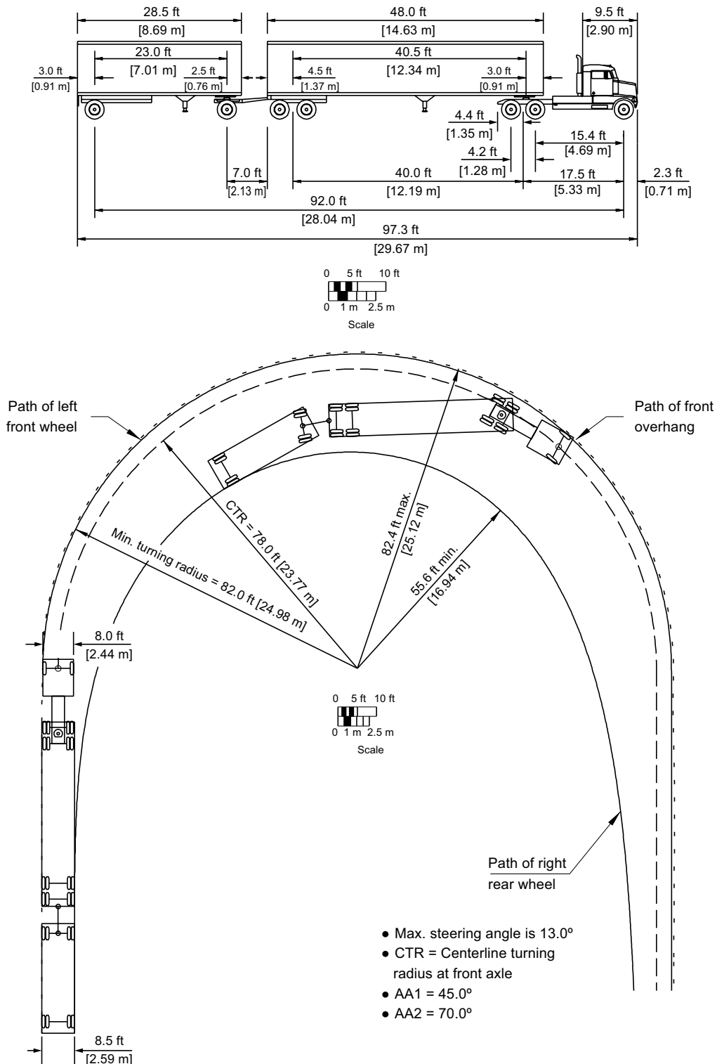
Figure 2-26. Minimum Turning Path for Rocky Mountain Double-Trailer Combination (WB-28D [WB-28D]) Design Vehicle
