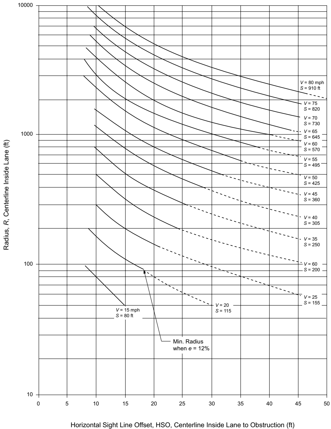
Figure 3-14. Horizontal Sightline Offset (HSO) to Provide Stopping Sight Distance on Horizontal Curves
