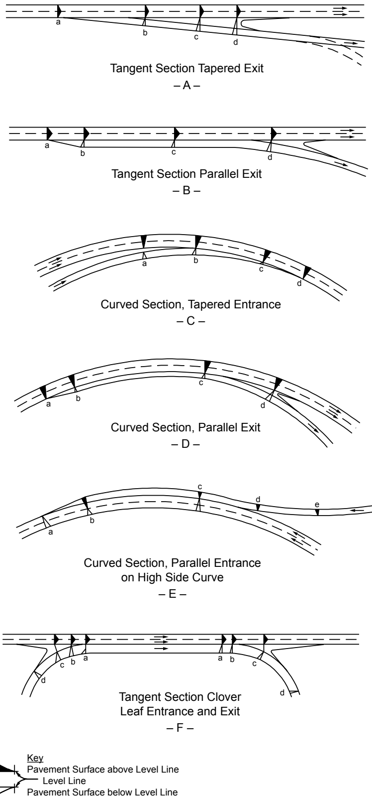
Figure 10-62. Development of Superelevation at Free-Flow Ramp Terminals
