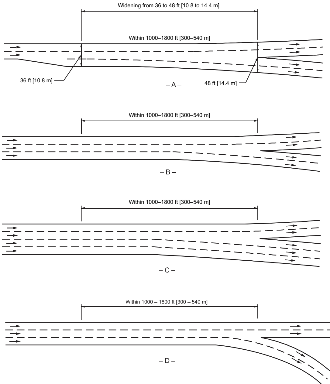
Figure 10-78. Major Forks
