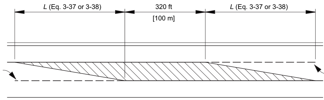
Figure 3-29. Schematic for Adjacent Lane Drop Tapers on a 2+1 Roadway
