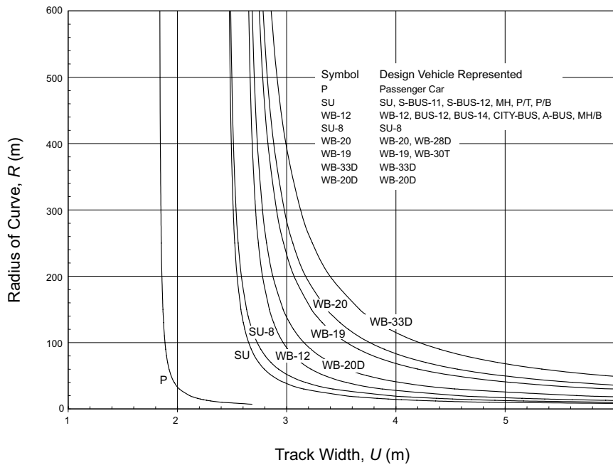
Figure 3-9. Track Width for Widening of Traveled Way on Curves
