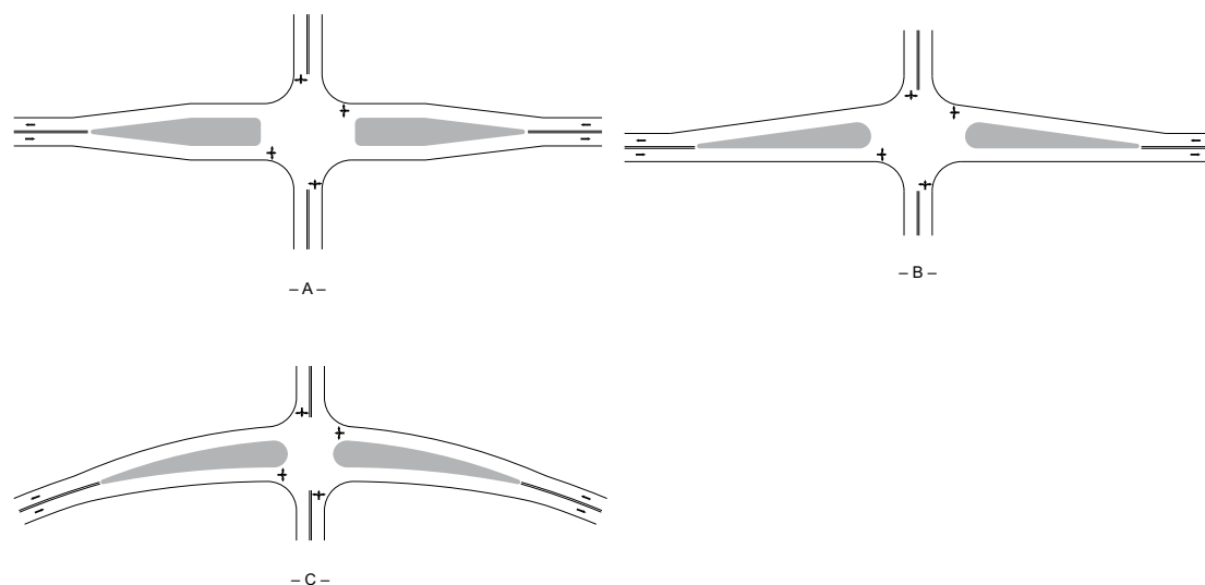
Figure 9-23. Alignment for Addition of Divisional Islands at Intersections
