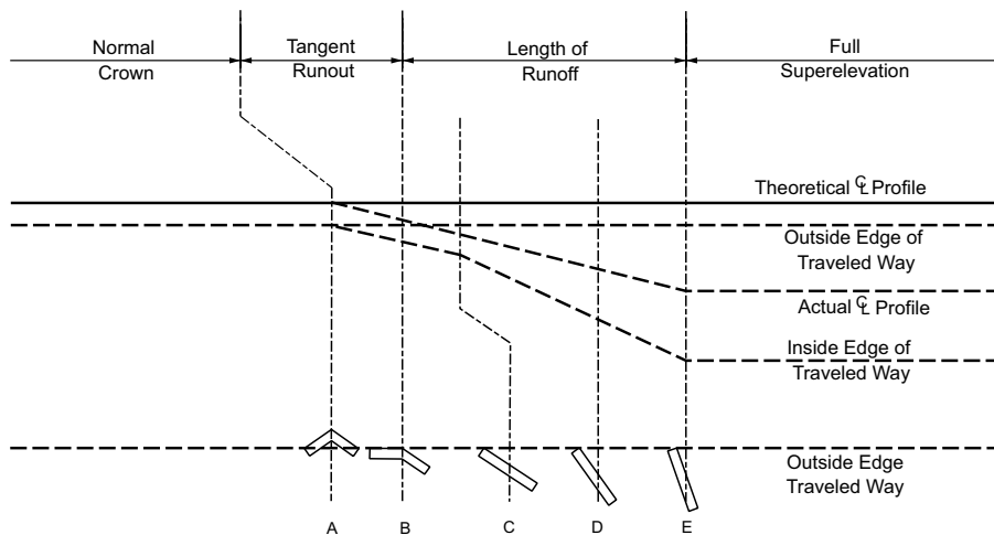
Crowned Traveled Way Revolved about Outside Edge
