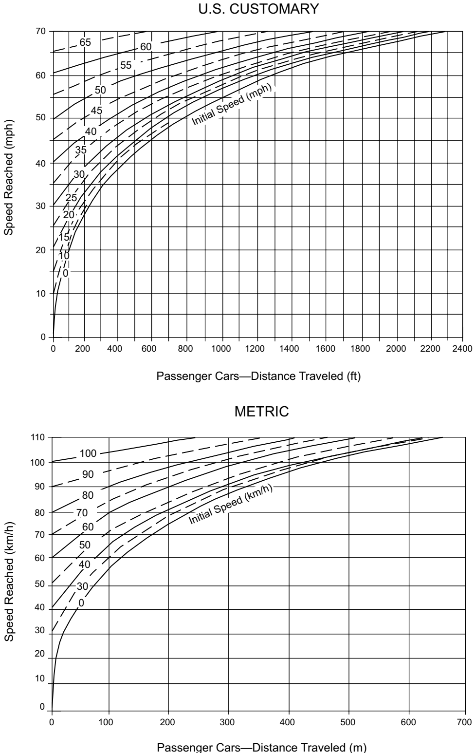
Figure 2-33. Acceleration of Passenger Cars, Level Conditions
