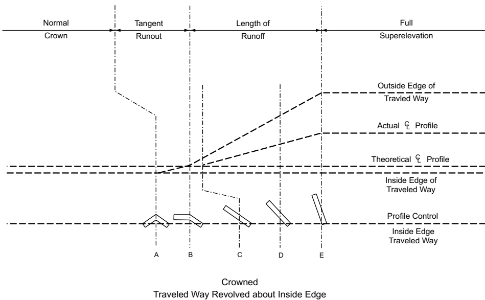
Figure 3-8. Diagrammatic Profiles Showing Methods of Attaining Superelevation for a Curve to the Right
