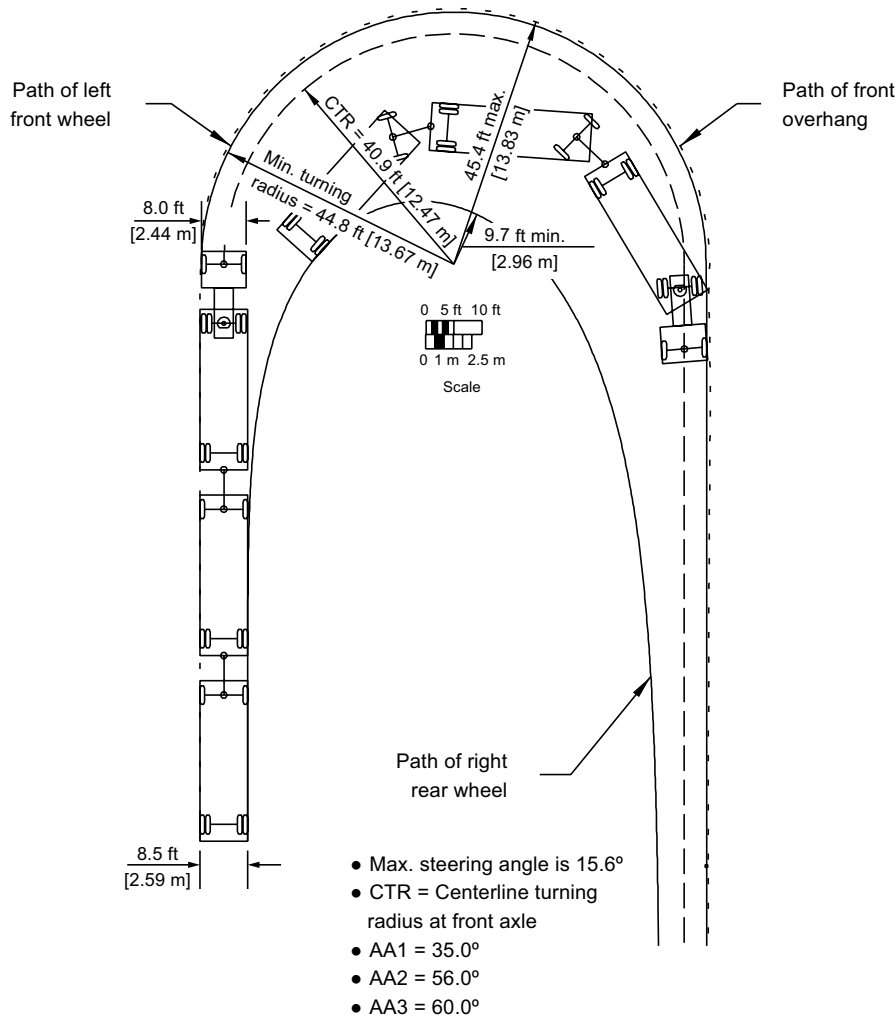
Figure 2-27. Minimum Turning Path for Triple-Trailer Combination (WB-100T [WB-30T]) Design Vehicle
