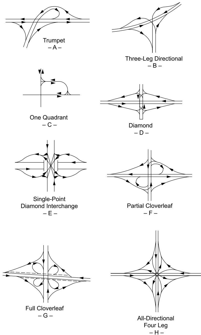
Figure 10-1. Interchange Configurations
