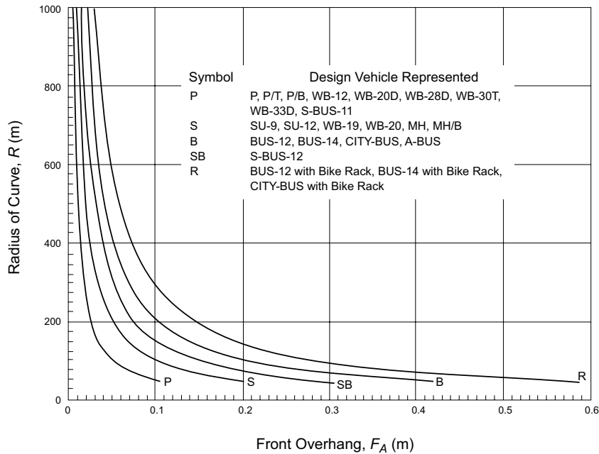
Figure 3-10. Front Overhang for Widening of Traveled Way on Curves
