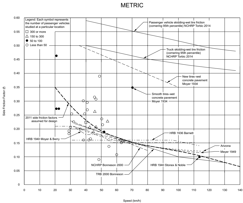
Figure 3-3. Side Friction Factors for Streets and Highways
