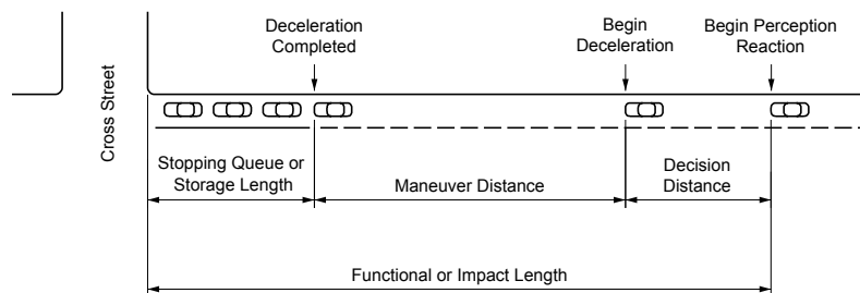
Figure 9-3. Elements of the Functional Area of an Intersection
