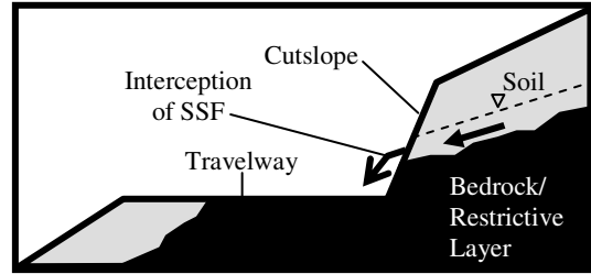
Figure 2. Schematic showing how subsurface stormflow (SSF) along the soil-bedrock interface can be intercepted by a road cutslope to create overland flow (modified from Ziegler et al., 2001b).
