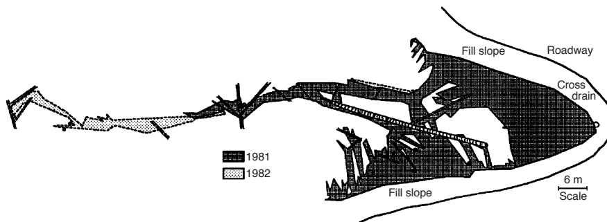
Figure 3 —Map of a typical cross drain sediment deposit over time.
