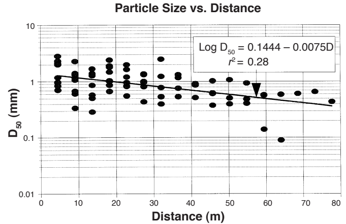
Figure 7—Median sediment particle size ( D_{50} ) as a function of travel distance.
