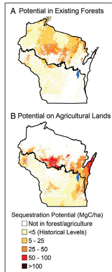
Figure 15.—Potential increases in aboveground carbon density if existing forests were allowed to grow to old age and all suitable agricultural land were converted to forest and allowed to fully re-grow. (From Rhemtulla et al. 2009, used with permission).
