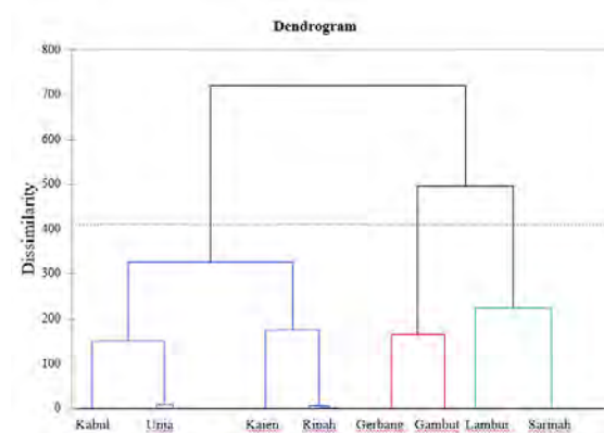
b) Dendrogram without biomass variable
