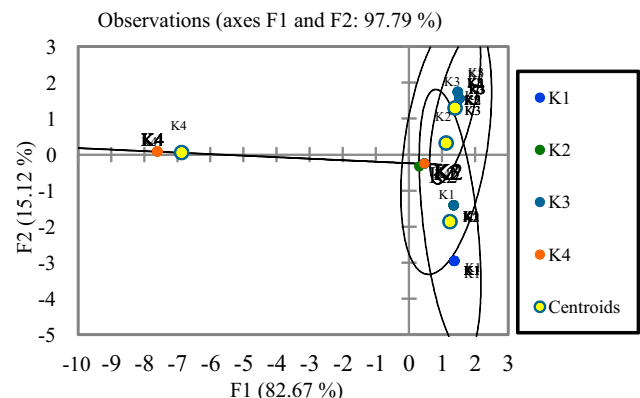
Figure 6 Scattered diagrams of K1 ~ K4 classes using canonical discriminant functions of F1 & F2 (variance of 97.8%).
