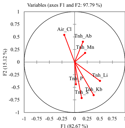
Figure 5 Relationship between the selected original variable and the canonical discriminant axis F1 and F2.
