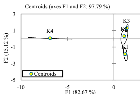
Figure 7 Diagram of centroid of each K1 ~ K4 classes using F1 and F2 axes.
