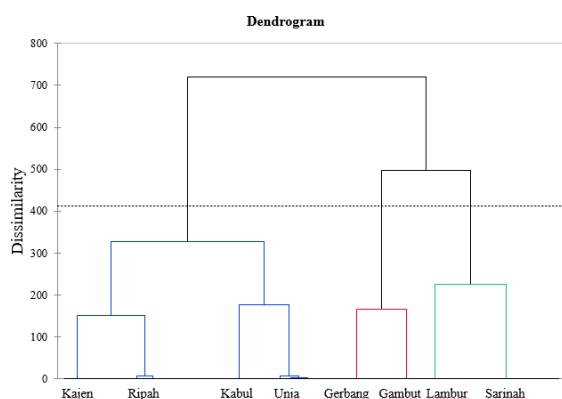
a) Dendrogram with biomass variable
